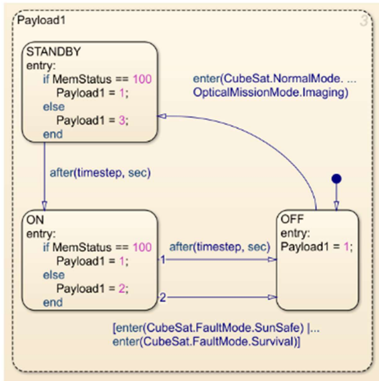
Figure 17: CubeSat Stateflow
