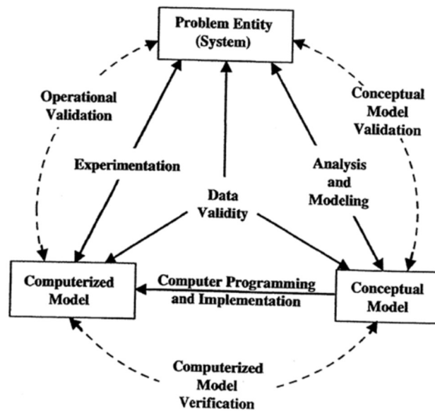
Figure 3: Verification & Validation (Sargent, 2014)
