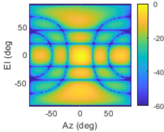
(c) 3 x 3 GS isolated unit cell.
