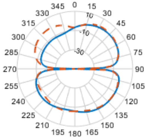
(c) GO at 5.14 GHz.
