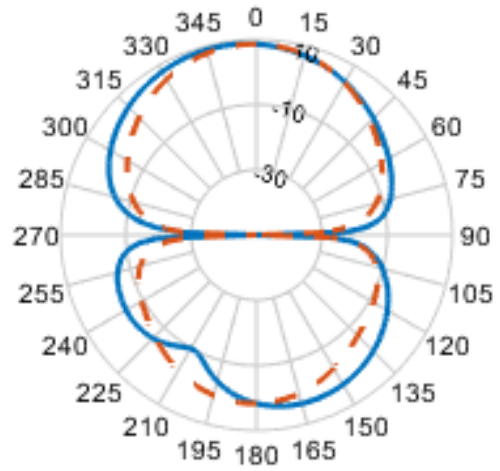
(b) NO at 5.78 GHz.
