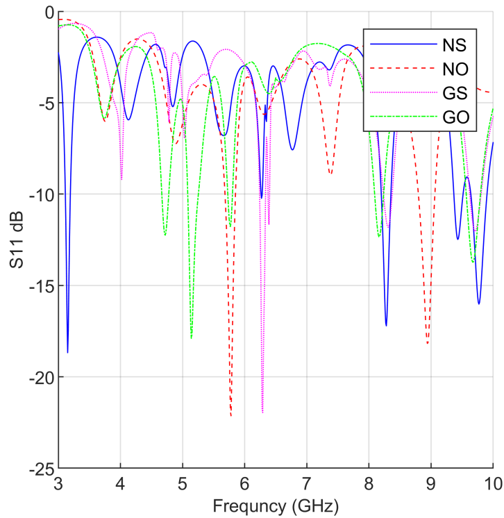
Figure 4.1: S11 in dB of the unit cell for each of the switch states.
