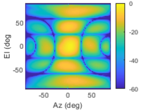
(b) 3 x 3 GO embedded unit cell.
