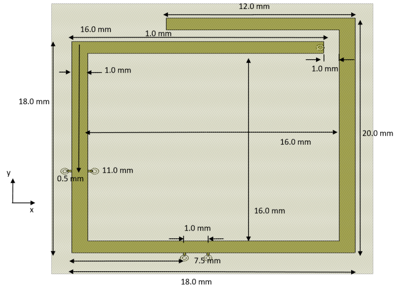
Figure 1.1: Single Square Spiral.
