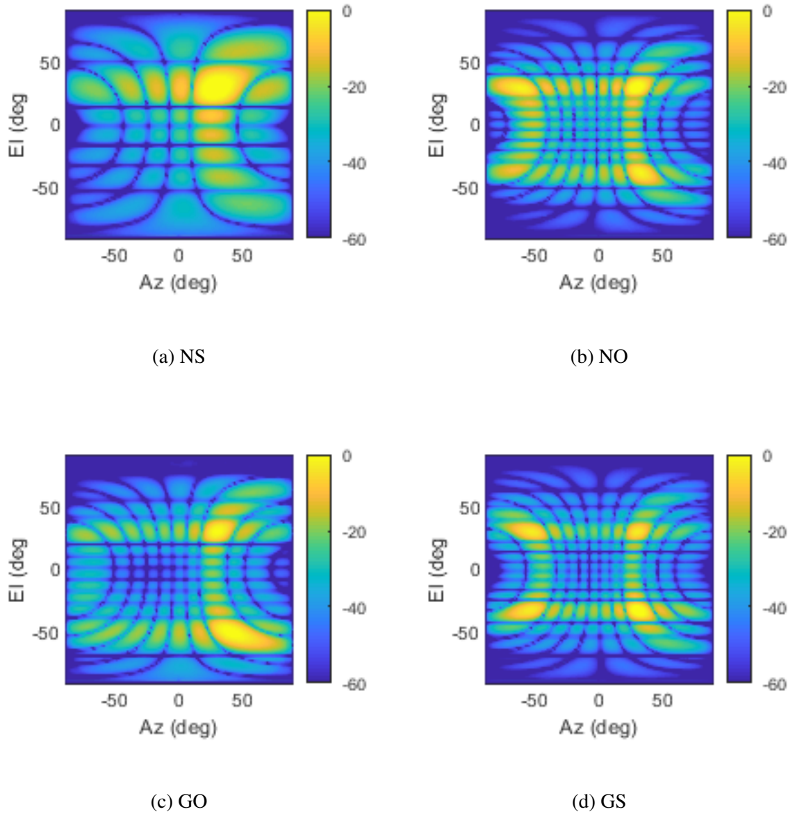
Figure 4.6: Normalized 3D gain pattern in dB for the 8x8 array. The signal is arriving from aspect ( \theta = 30 deg, \phi = 30 deg.)
