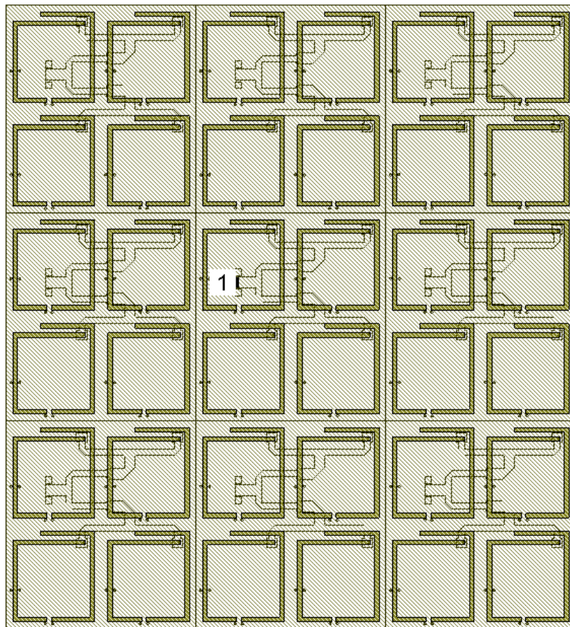
Figure 3.7: Embedded unit cell.
