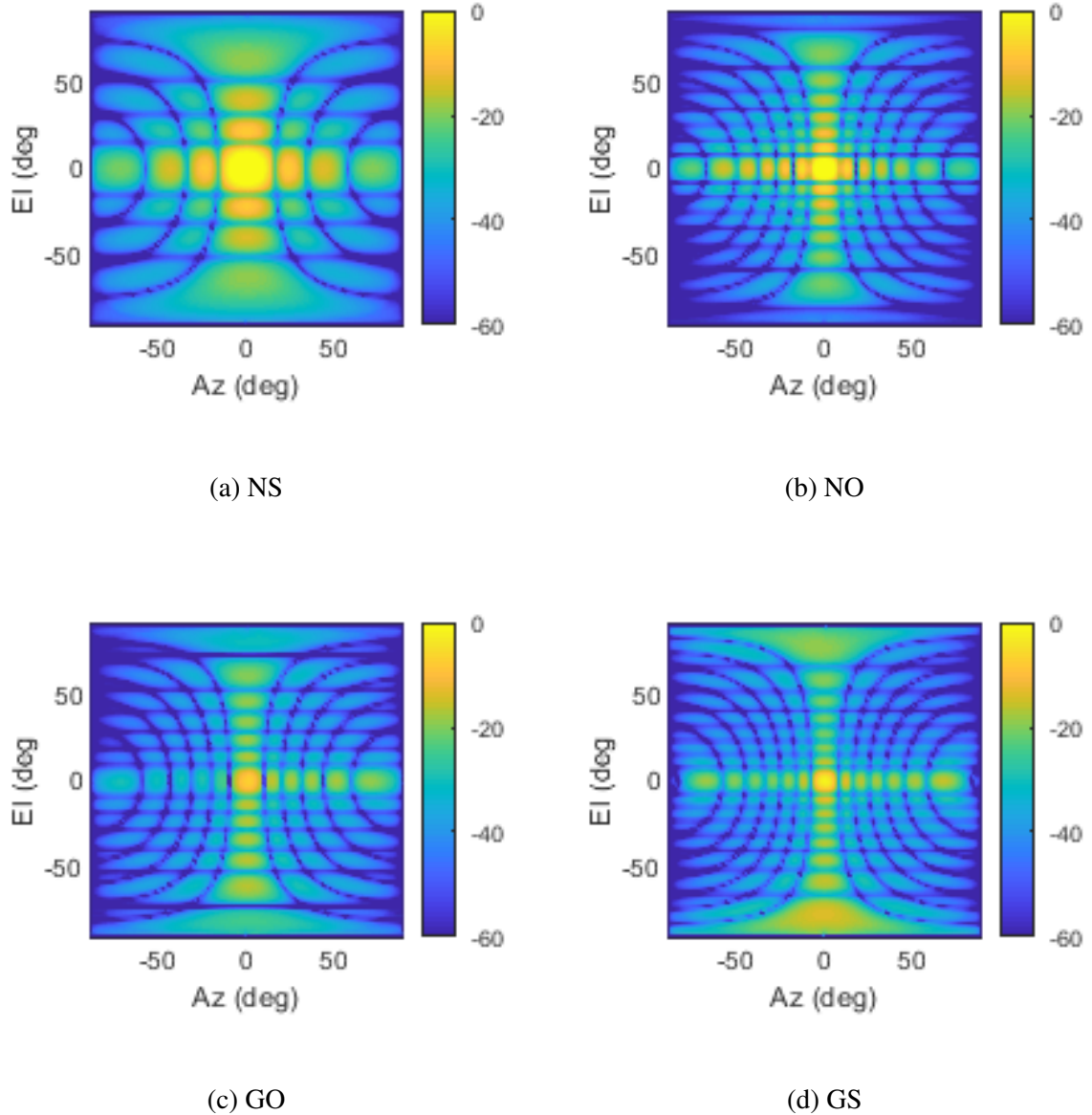
Figure 4.5: Normalized 3D gain pattern in dB for the 8x8 array. The signal is arriving from aspect ( \theta = 0 deg, \phi = 0 deg ).
