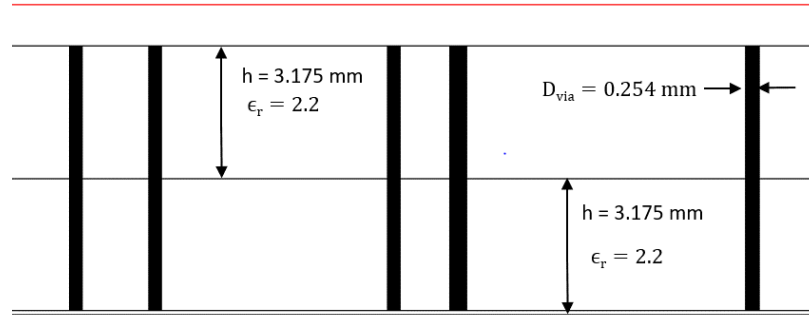
Figure 3.5: Substrate Side View With Dimensions.
