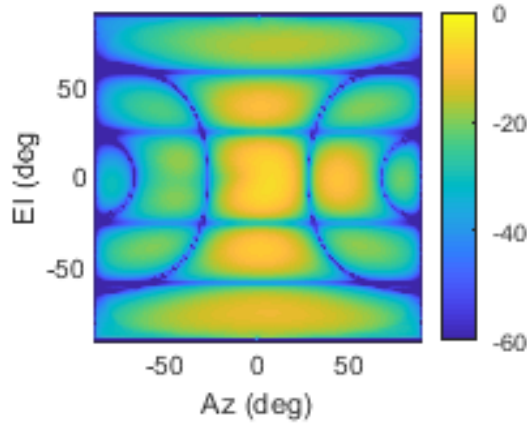
(a) 3 x 3 GO isolated unit cell.
