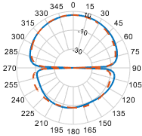
(a) NS at 3.15 GHz.
