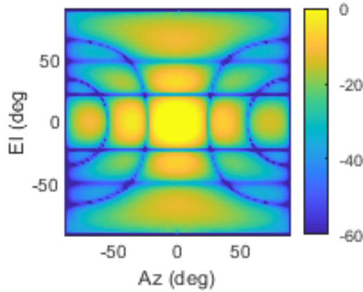
(c) 3 x 3 NO isolated unit cell.
