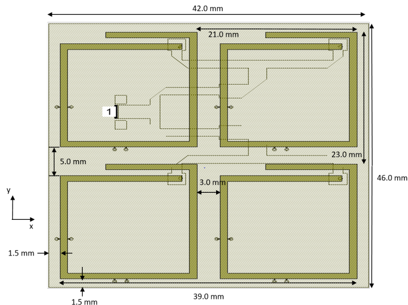
Figure 3.3: Unit cell with dimensions.
