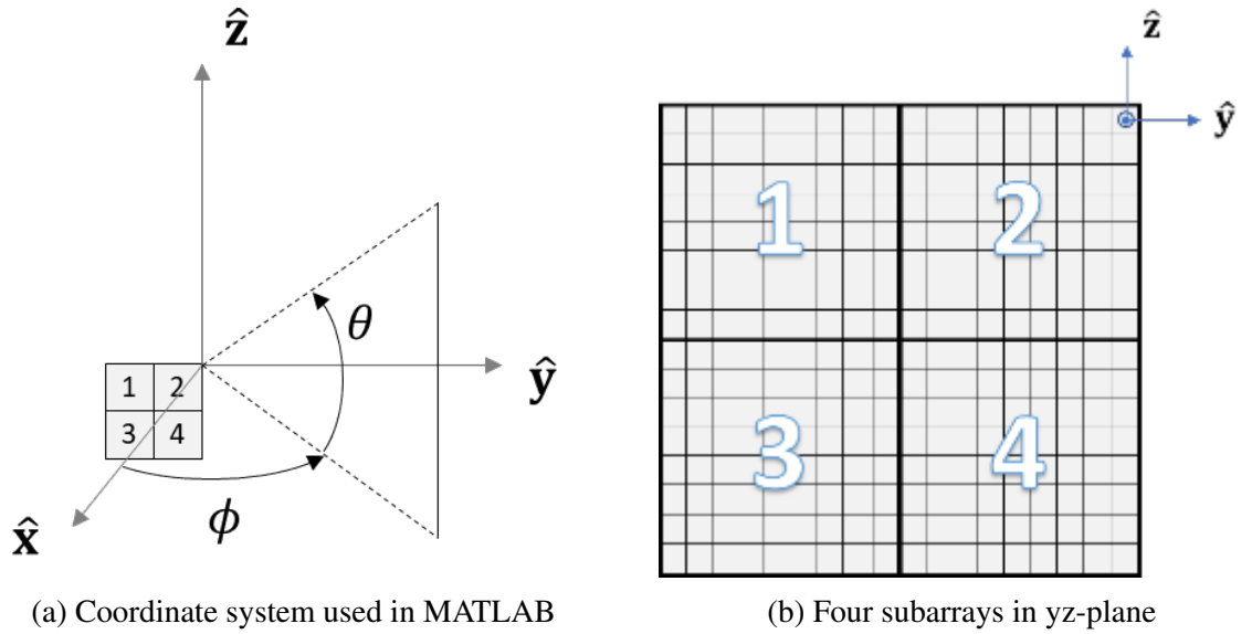
Figure 3.6: Array frame of reference
