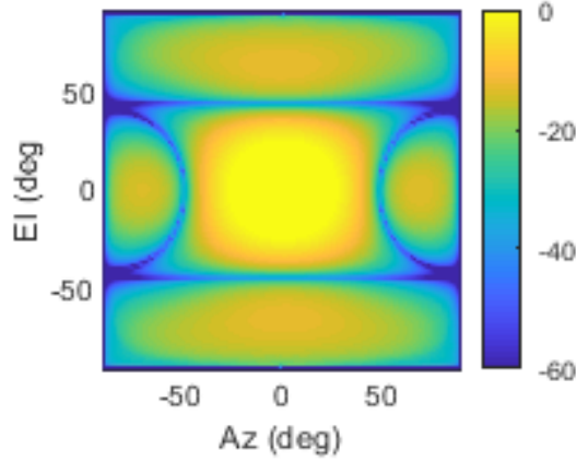
(a) 3 x 3 NS isolated unit cell.
