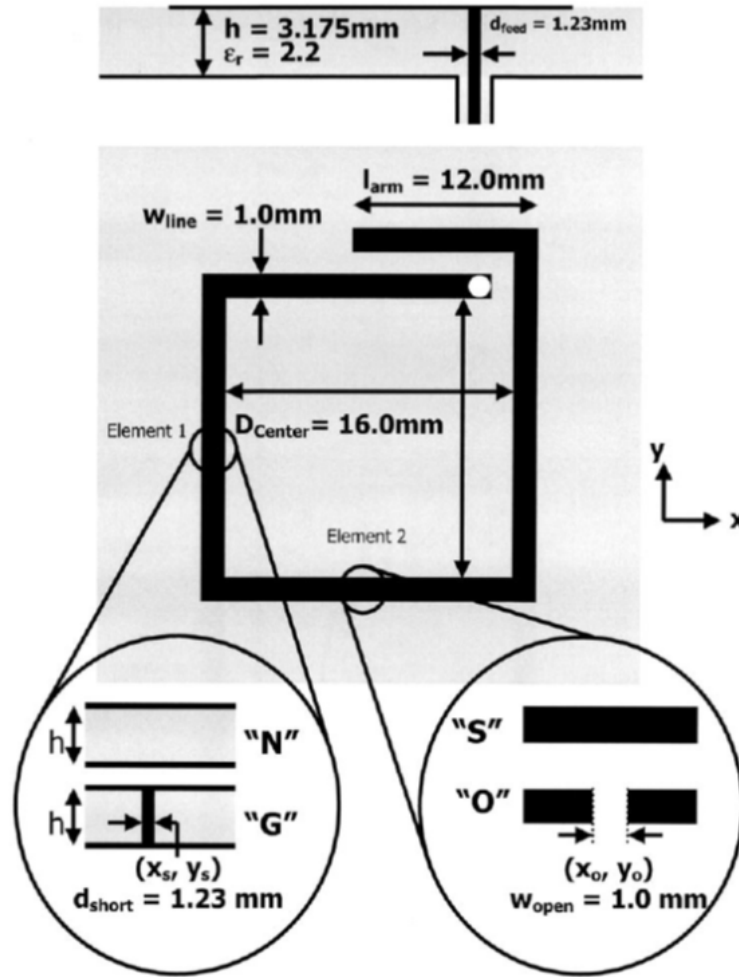
Fig. 1. Antenna geometry showing switches necessary for reconfiguration.
