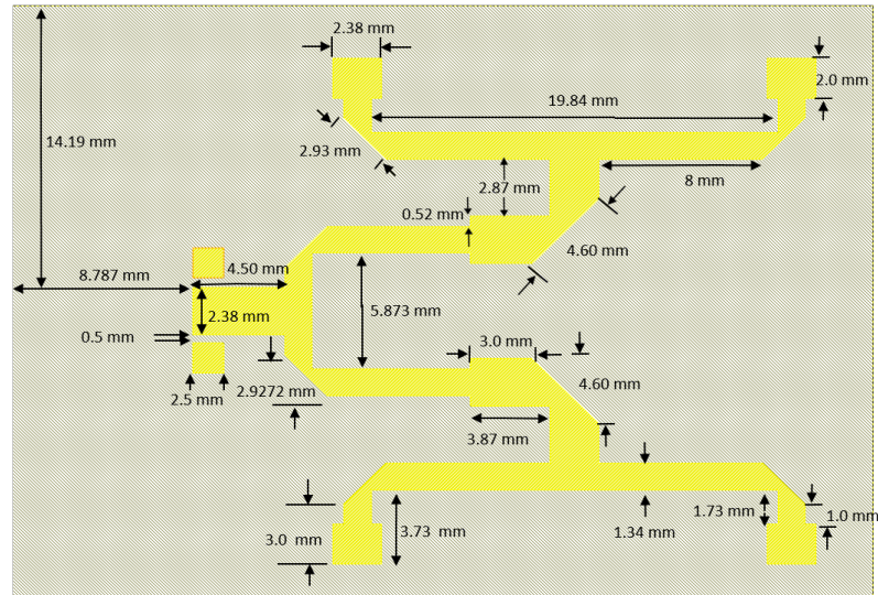
Figure 3.4: Feed network with dimensions.
