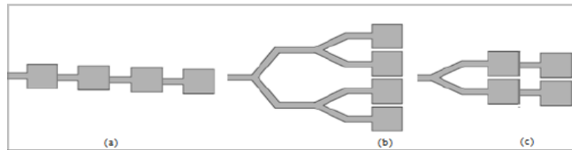
Figure 2.1: (a) series fed array. (b) Multiple feed lines known as corporate feed. (c). Combination of both feeding techniques. [1]
