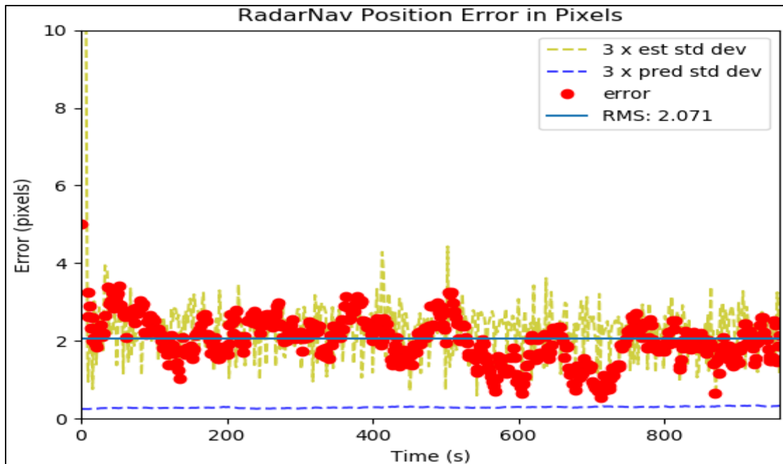
Figure 46. Plot of pixel errors vs. time for Astoria, OR data set.
