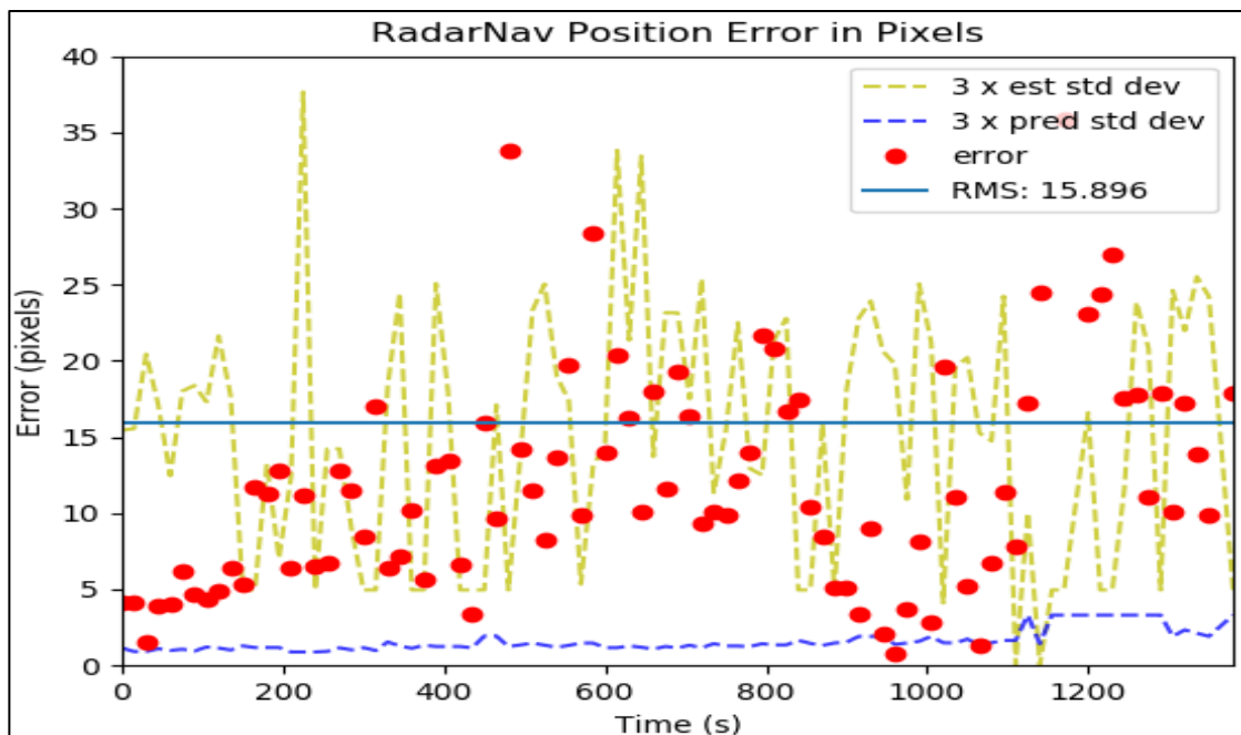
Figure 31. Plot of pixel errors vs. time for Norfolk, VA data set.
