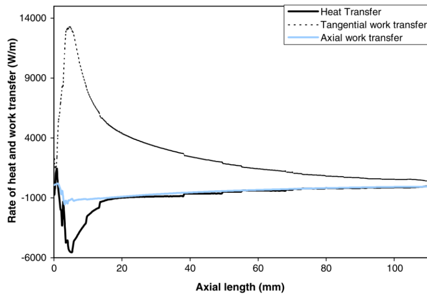
Figure 54. Vortex tube energy transfer components from CFD ( \mu_c = 0.74 ) [66]
