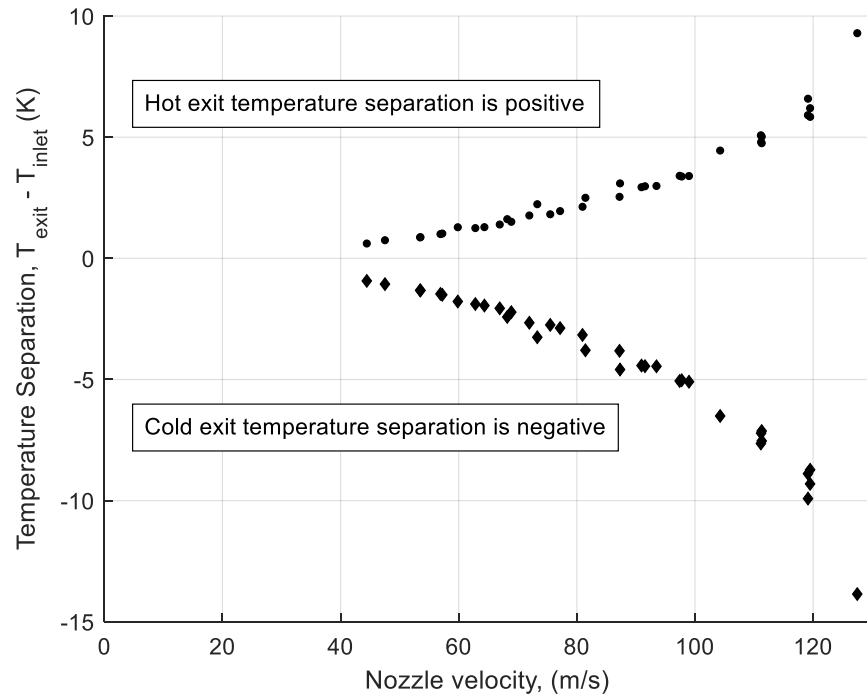
Figure 69. Temperature separation vs. nozzle velocity ( \mu_C = 0.40 )
