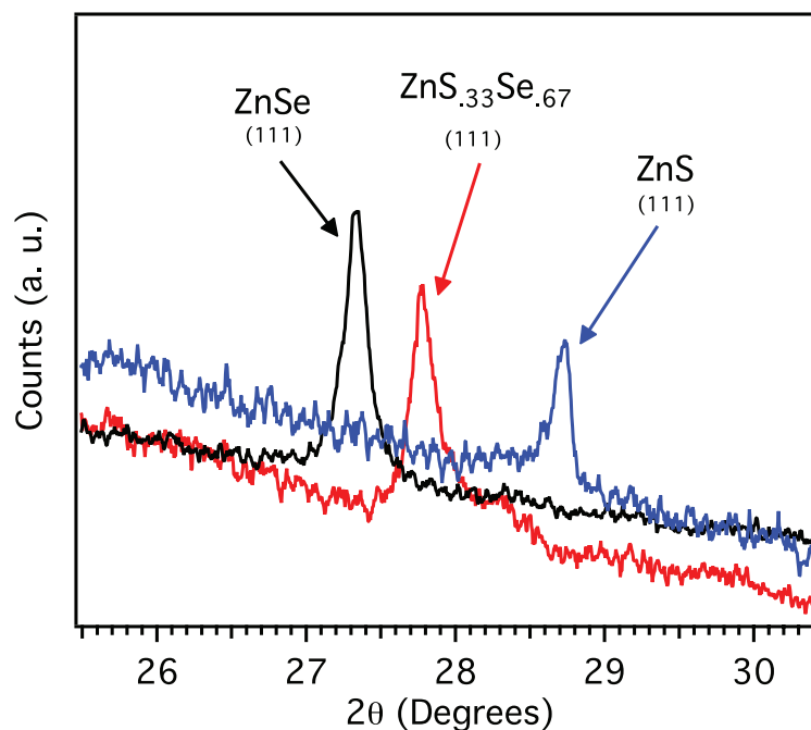
Figure 4.4: Vegard's law analysis of ZnS x Se (1-x) alloys. The shift in the (111) diffraction peak is consistent with the stoichiometry of the material determined by energy dispersive spectroscopy.
