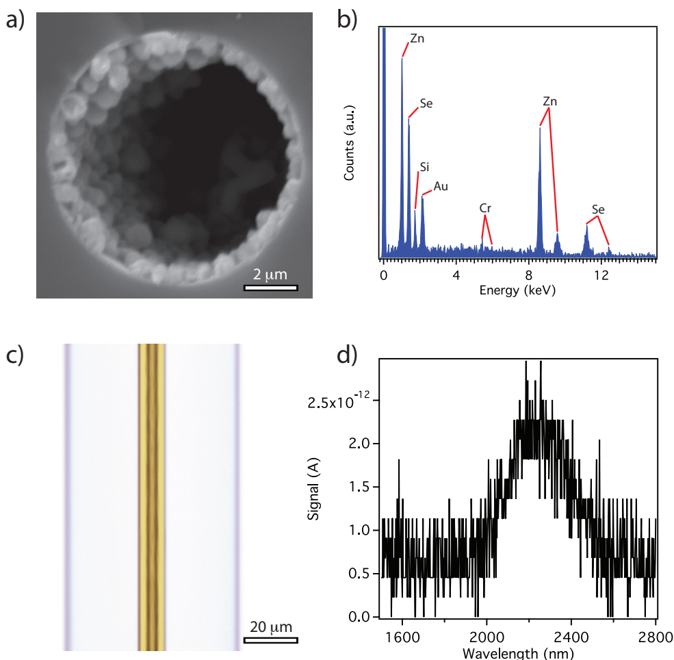
Figure 6.3: Deposition of \text{Cr}^{2+}:\text{ZnSe} with \text{Cr}(\text{CO})_6 as the chromium source. \text{Cr}/\text{Zn} islands are observed in SEM (a) and EDS (b) when the reactant ratios are not optimized. After optimization, \text{Cr}^{2+}:\text{ZnSe} films can be deposited (c), but the doping level is very low as indicated by mid-IR emission (d) due to the low thermal stability of \text{Cr}(\text{CO})_6 compared to the \text{ZnSe} reaction.
