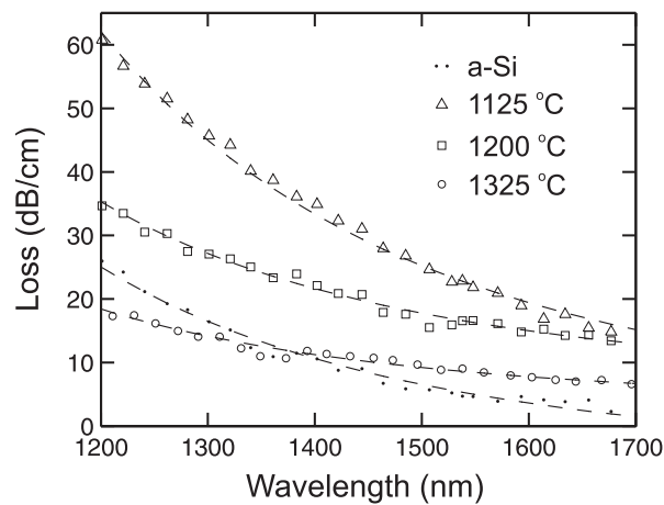
Figure 3.3: Optical loss as a function of wavelength of silicon optical fibers in the amorphous state and annealed at different temperatures. [1] Dashed lines are \lambda^{-4} fits.
