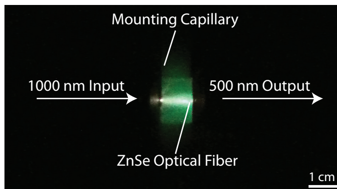
Figure 5.6: Photograph of a ZnSe optical fiber generating second harmonic light.
