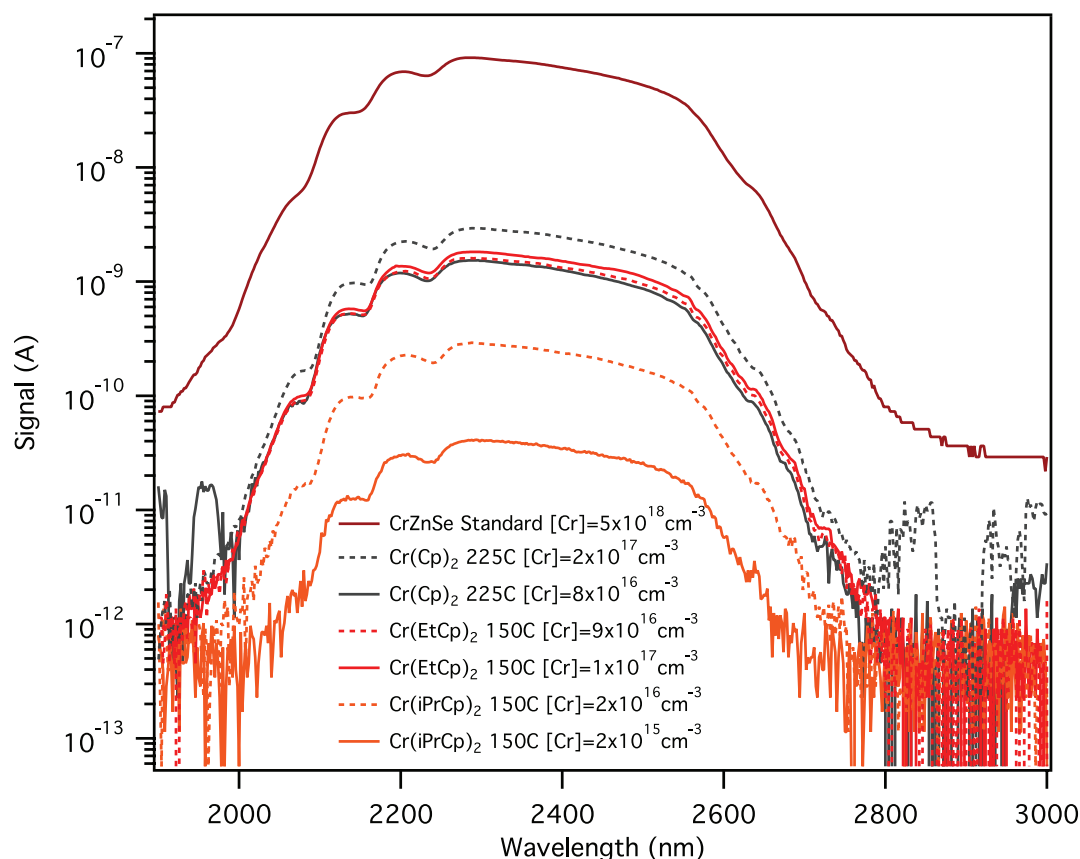
Figure 6.7: \text{Cr}^{2+} :ZnSe signal as a function of ring substitution on chromocene. The length difference from the dashed and solid lines of a given sample is \sim 1 cm. The concentrations of chromium are calculated by comparing to the standard of known concentration.
