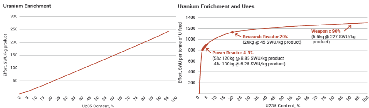
Figure A-1 Left: SWU required to produce uranium of a given U-235 enrichment, per kg of output product uranium. Right: SWU required to produce uranium of a given U-235 enrichment, per tonne of natural uranium feed. 229
