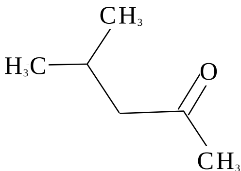
Figure 2. Methyl Isobutyl Ketone (MIBK)
