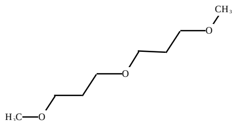
Figure 22. Dipropylene Glycol Dimethyl Ether
