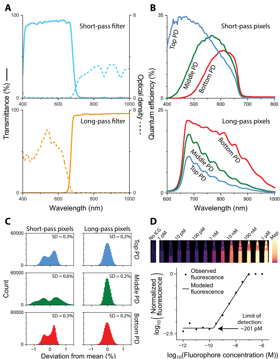
Fig. 2. Optoelectronic characteristics of the bioinspired imager. (A) Transmission and optical density curves for the short-pass filters (top) and long-pass filters (bottom). (B) Quantum efficiency curves for the three photodiode layers under the short-pass filters (top) and long-pass filters (bottom). (C) Fixed pattern noise histograms at half the linear full-scale range for the three photodiode layers under the short-pass filters (left) and long-pass filters (right). The fixed pattern noise is the SD of the histograms. (D) Normalized fluorescence observed and modeled across different concentrations of indocyanine green (ICG). Temporally averaged intensity images are displayed against concentration (top), and spatiotemporally averaged intensities are plotted against concentration (bottom). The detection limit (201 pM) is the transition point between the constant region below the noise floor and the linear region above the noise floor. PD, photodiode.
