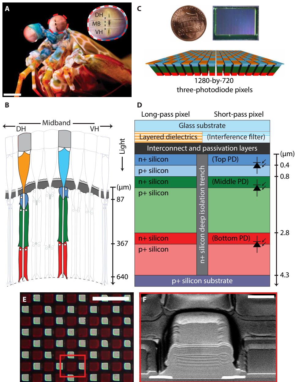
Fig. 1. Comparison of the mantis shrimp compound eye and the bioinspired image sensor. (A) Photograph of the mantis shrimp Odontodactylus scyllarus and magnified photograph of its compound eye (inset); scale bar, 5 mm. (B) A cross-section of the compound eye of the mantis shrimp Gonodactylus chiragra shows the photosensitive cells and spectral filters; structures without dimensions are not to scale. The photosensitive cells at the bottom, middle, and top have been colored red, green, and blue, respectively, to emphasize that longer wavelengths of light penetrate farther than shorter wavelengths. (C) Photograph of the bioinspired imager (top) and magnified illustration of the pixel array (bottom); scale is indicated by the penny. (D) A cross-section of the bioinspired imager shows the vertically stacked photodiodes, composed of layers of n-doped silicon and p-doped silicon, and the interference filters, composed of layers of different dielectric materials; structures without dimensions are not to scale. The photodiodes at the bottom, middle, and top have been colored red, green, and blue, respectively, to emphasize that longer wavelengths of light are absorbed deeper in the silicon than shorter wavelengths. (E) An optical microscope image of the pixelated optical filters shows the long-pass filters as dark colored squares and the short-pass filters as bright colored squares; scale bar, 50 \mu\text{m} . (F) A scanning electron microscope image depicts a long-pass filter in the center and short-pass filters on both sides; scale bar, 5 \mu\text{m} . (A) Credit: Michael Bok, University of Lund. In (B), the cross-section is adapted from (23). In (C) and (D), the magnified illustration and cross-section present a conceptual view of the device, omitting some details for clarity. DH, dorsal hemisphere; MB, midband; PD, photodiode; VH, ventral hemisphere.
