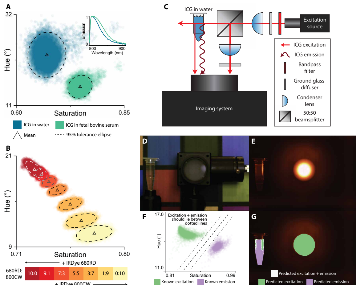
Fig. 3. Imaging capabilities of the bioinspired imager. (A) Discrimination of indocyanine green (ICG) diluted in two different media (deionized water and fetal bovine serum) showing the uncertainty created by temporal and spatial noise. Observations of different solutions appear in different clusters and are circled by 95% tolerance ellipses ( n_{\text{observations}} = 27,000 per solution). Emission spectra for the two solutions are displayed in the top-right inset. (B) Discrimination of IRDye 680RD and IRDye 800CW mixed in different volumetric ratios showing the uncertainty created by temporal and spatial noise. Observations of different ratios appear in different clusters and are circled by 95% tolerance ellipses ( n_{\text{observations}} = 27,000 per solution). Emission spectra for IRDye 680RD and IRDye 800CW are strongest at ~694 and ~794 nm, respectively. (C to G) Discrimination of ICG excitation and emission in the presence of spatial noise. (C and D) Schematic (C) and color photograph (D) of the experimental setup. Excitation is projected from the port; emission is generated in and excitation is reflected from the vial. (E) Near-infrared image of the experimental setup. Pure excitation is observed inside the port; pure excitation, pure emission, and mixed excitation-emission are observed inside the vial. (F) Temporally averaged observations of pure excitation and pure emission cluster differently, permitting classification via a simple margin classifier such as a linear support vector machine ( n_{\text{observations}} = 8246 for excitation and 2665 for emission). Observations of mixed excitation-emission should lie between and are classified accordingly. (G) Labels of pure excitation, pure emission, and mixed excitation-emission can be applied to the near-infrared image using the classifier.
