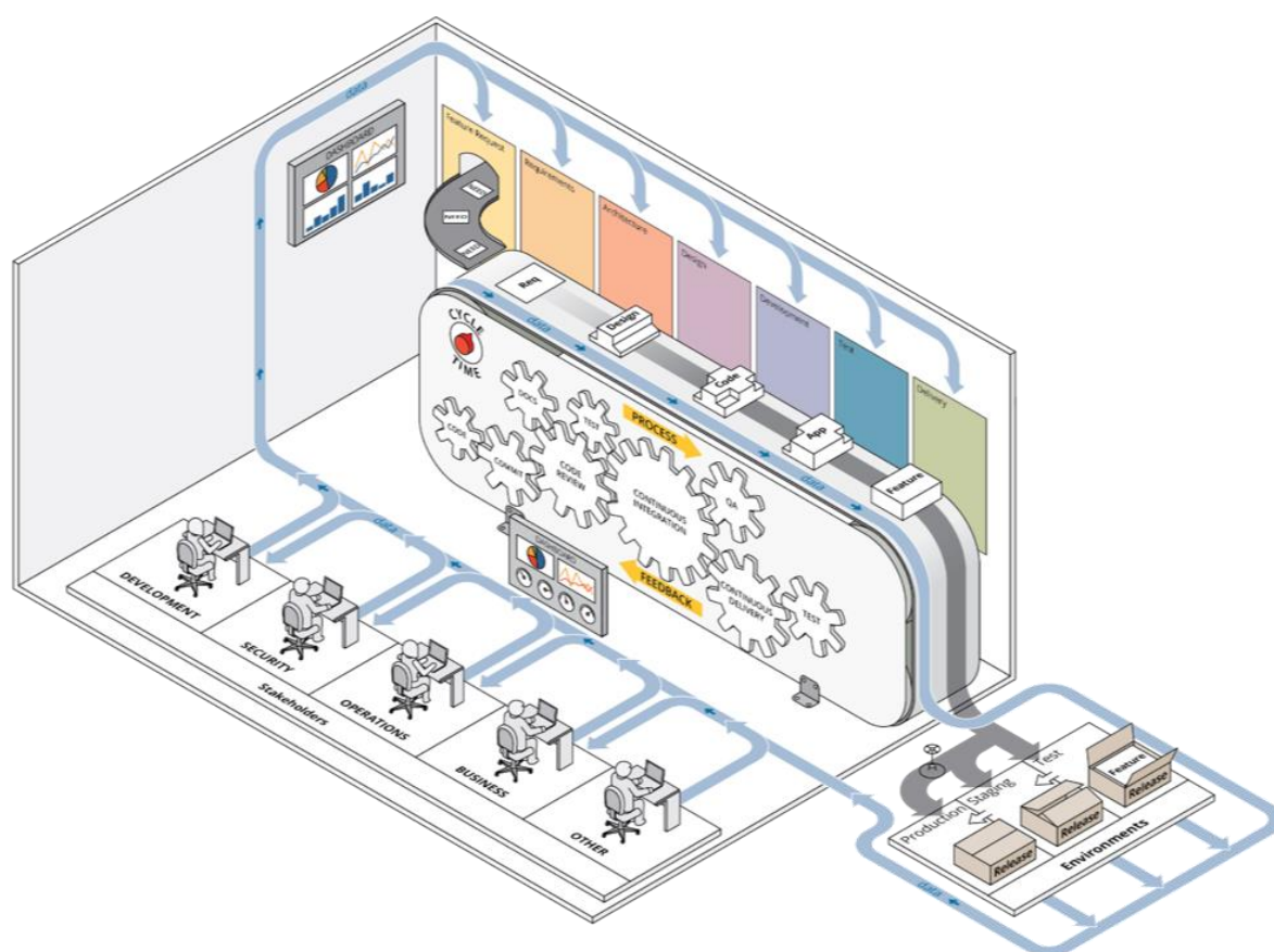
Figure 9: DevSecOps Pipeline
