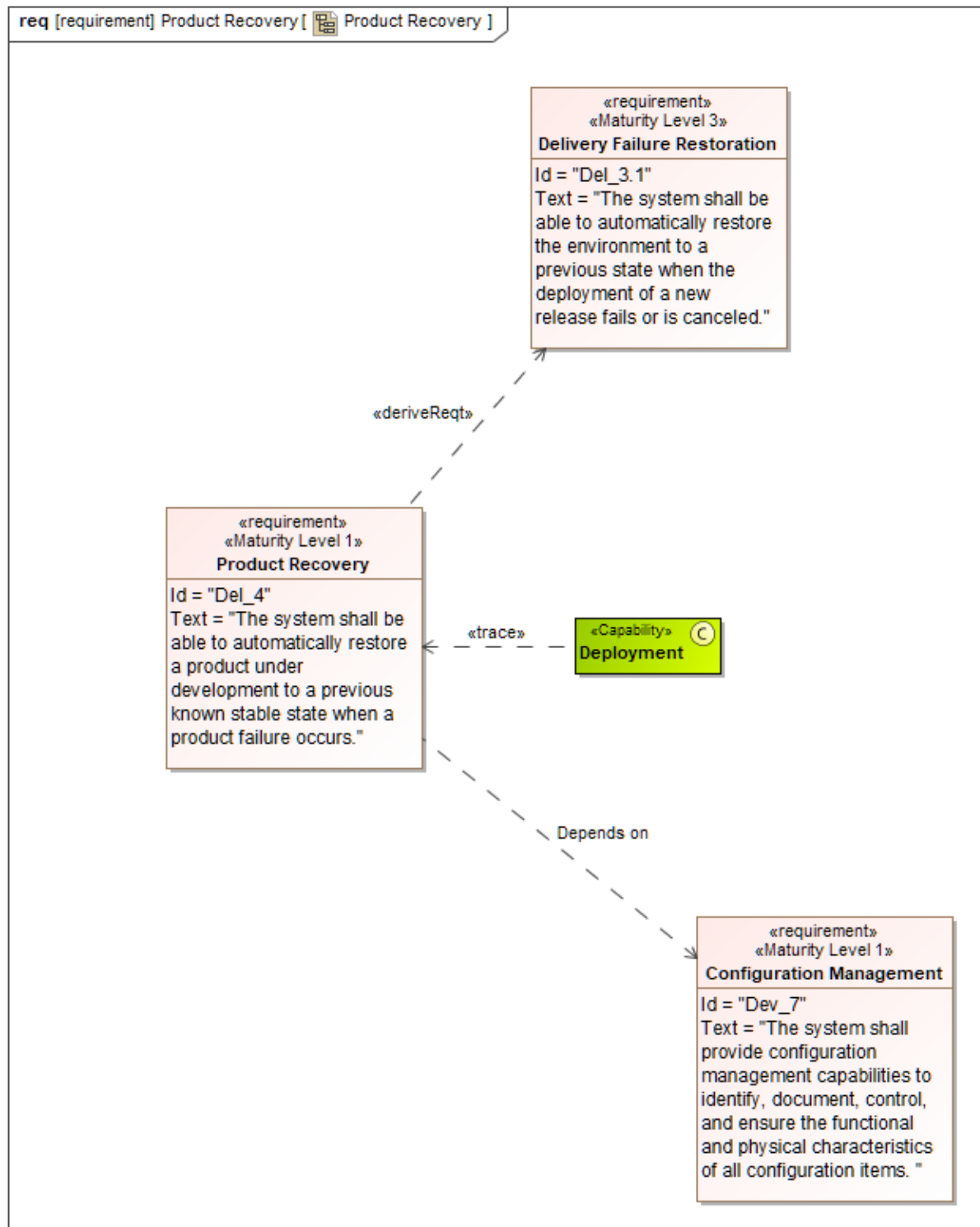
Figure 48: Product Recovery
