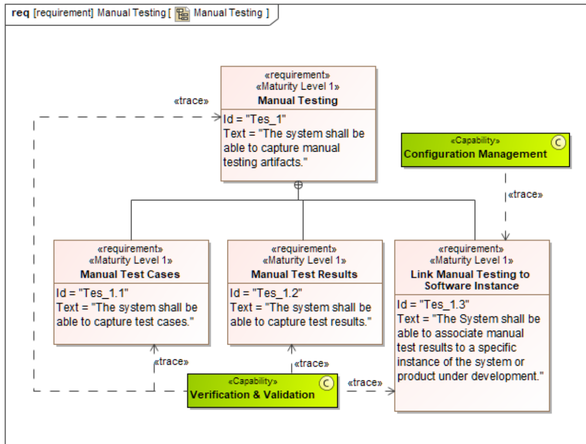
Figure 38: Manual Testing
