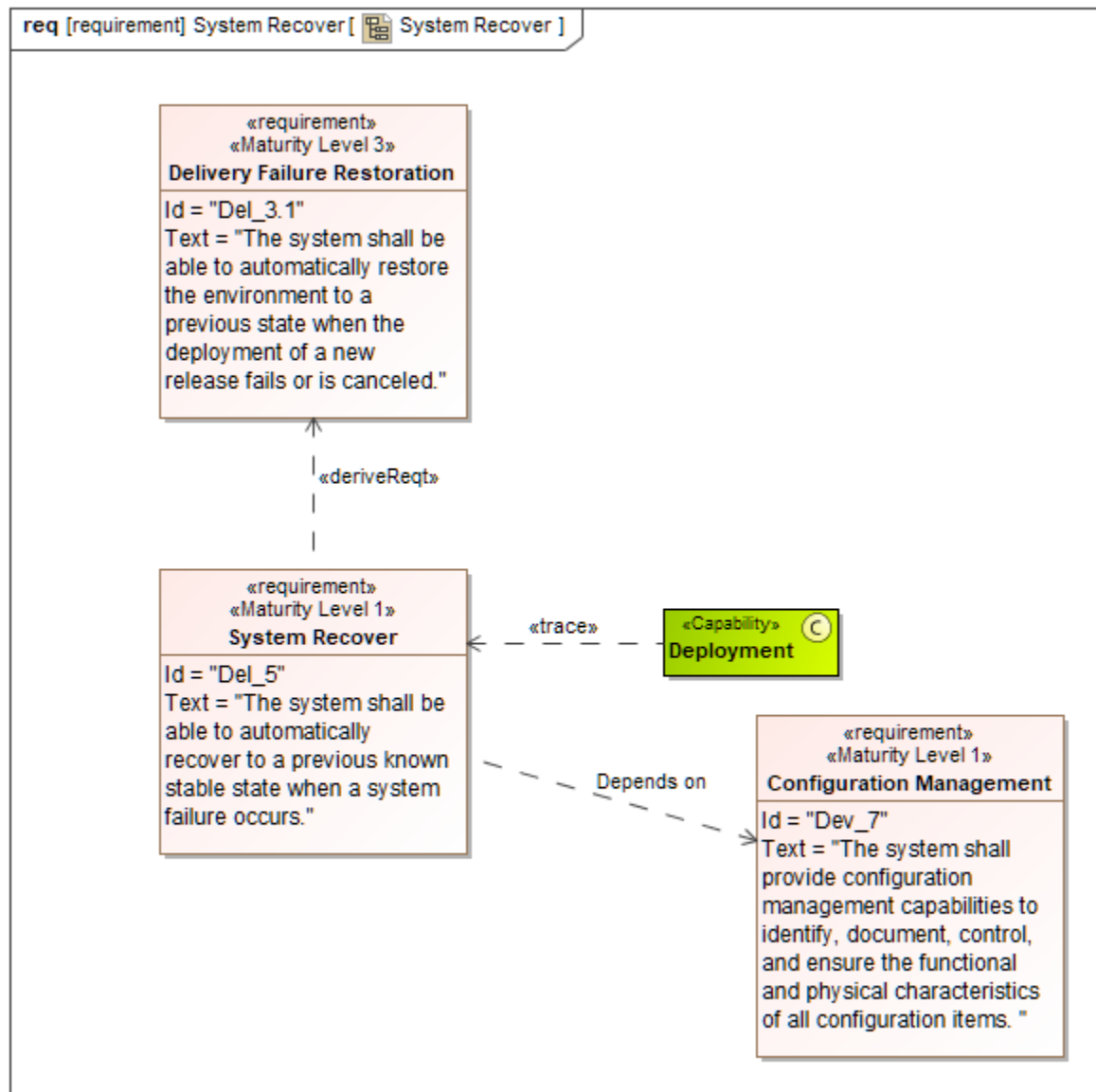
Figure 49: System Recover
