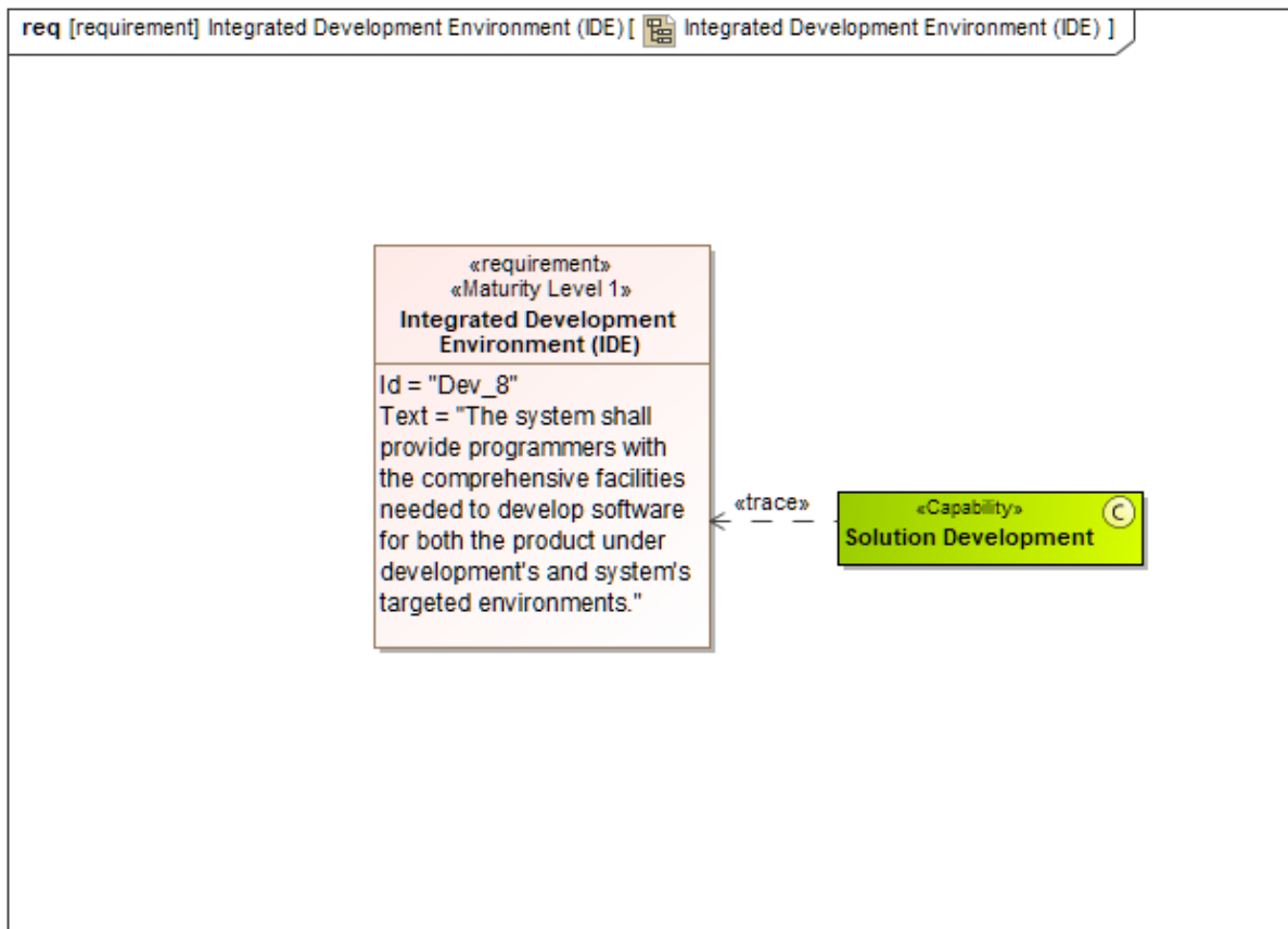
Figure 36: Integrated Development Environment (IDE)
