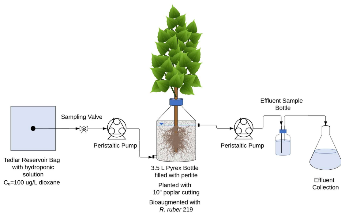
Figure 4. Flow-through experimental design conducted in modified 3.5-L Pyrex bottles filled with perlite.
