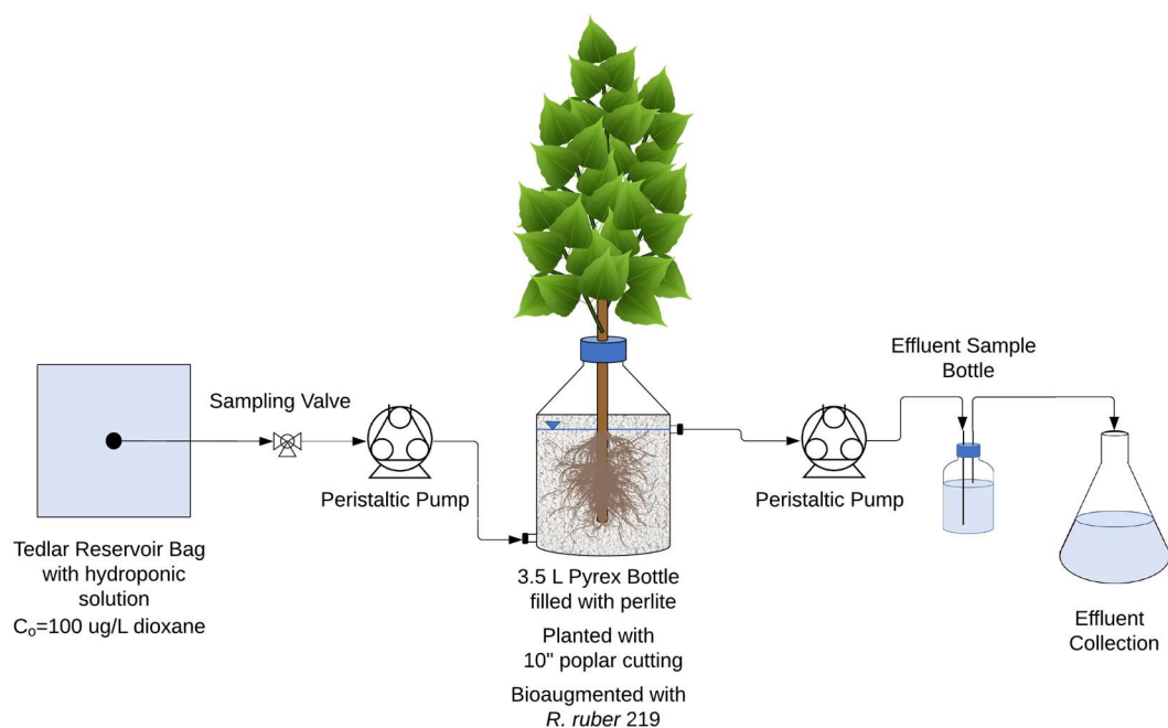
Figure 1. Flow-through experimental design used to evaluate bioaugmented phytoremediation as a strategy to treat dioxane-contaminated groundwater.
