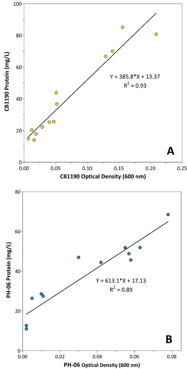
Figure A1. Correlation between optical density (600 nm) and biomass measured as protein for Pseudonocardia dioxanivorans CB1190 (A) and Mycobacterium dioxanotrophicus PH-06 (B). Strains grown in Ammonium Mineral Salts media with C_0 = 500 mg/L dioxane. Reactors were sonicated for 10 minutes prior to sampling.
