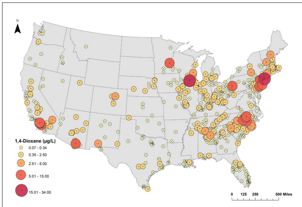
Figure 1. Locations with 1,4-dioxane concentrations in finished drinking water above Mandatory Reporting Limit (MRL) of 0.07 µg/L at Public Water Systems, 2013-2015. Data obtained from US EPA Unregulated Contaminant Monitoring Rule 3 (UCMR 3) (USEPA, 2017a). Map made using ArcGIS 10.4.1 (ESRI, Redlands, CA).
