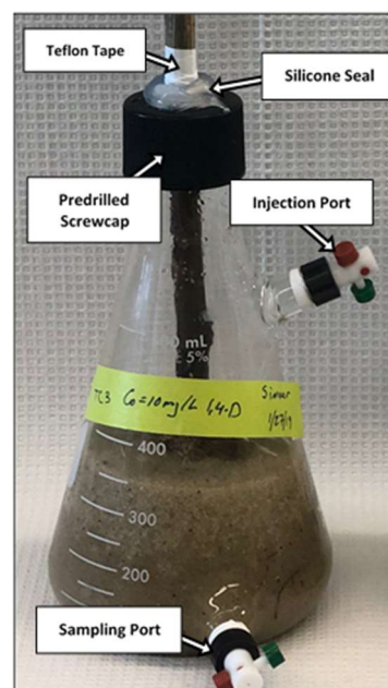
Figure 3. Hybrid poplar in a modified Erlenmeyer bioreactor.
