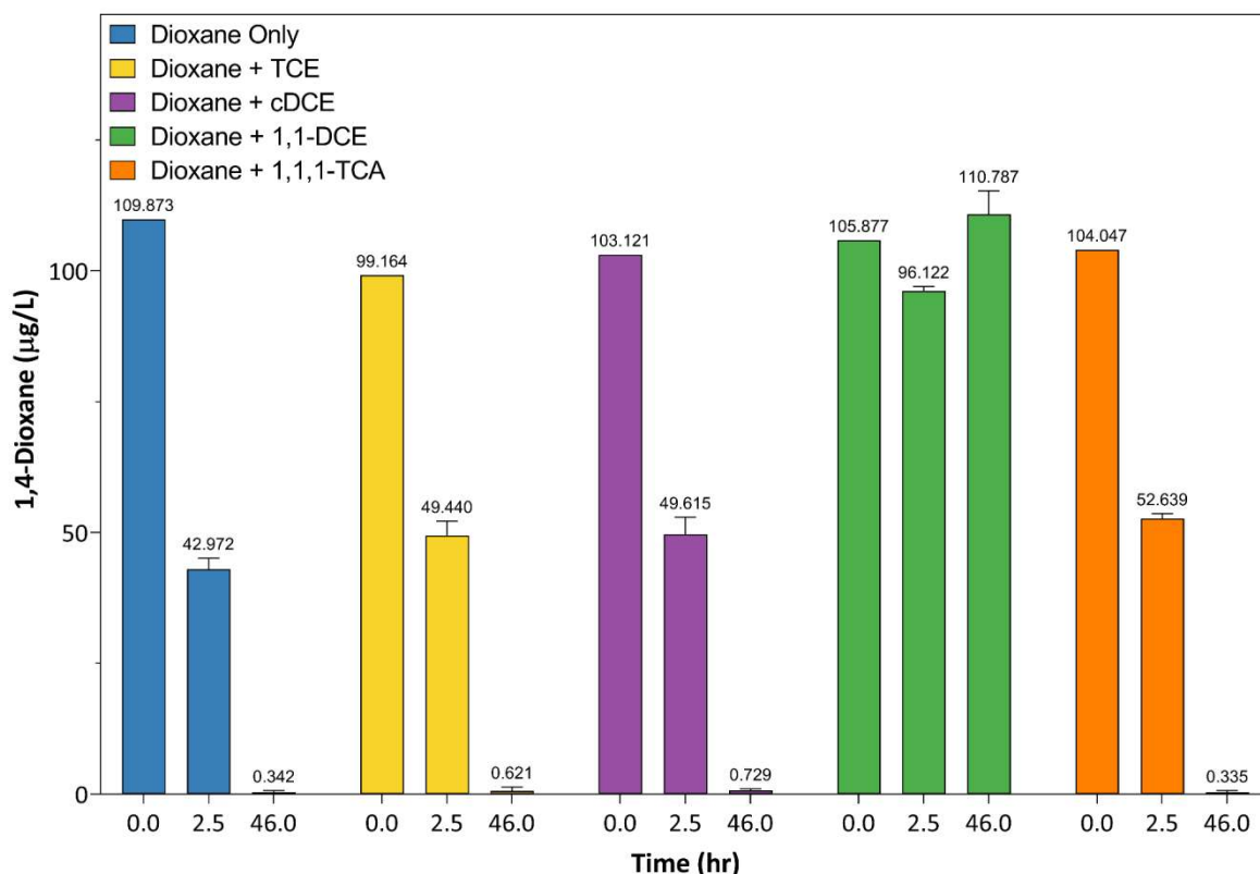
Figure 11. Dioxane degradation by R. ruber 219 measured over time in chlorinated solvent inhibition tests. Numbers above bars indicate the average dioxane concentration in µg/L. Experiment conducted in triplicate with \pm 1 standard deviation error bars.
