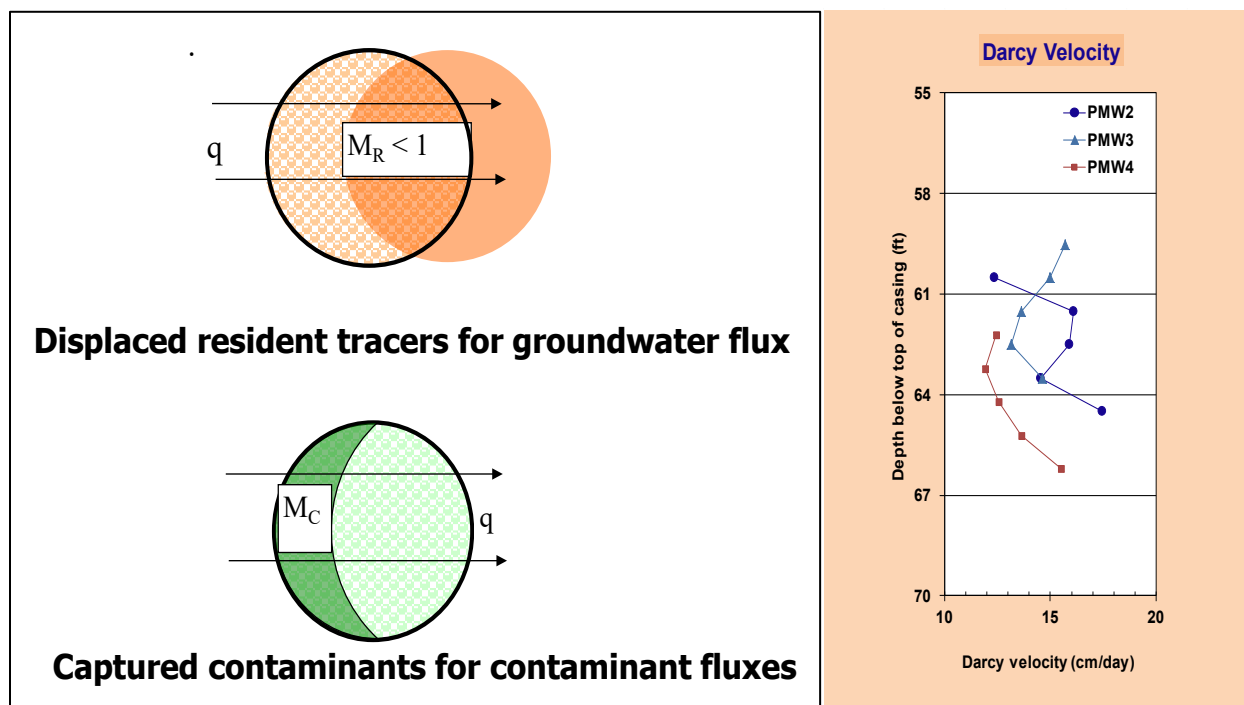
Figure 2-2. Graphic Showing the Dual Use of Mass Flux Meters for Both Groundwater and Contaminant Mass Flux (Left Panel) and an Example of Data Generated Using Passive Flux Meters to Quantify Fluid Flux in a Groundwater Aquifer in Rancho Cordova, CA (Right Panel).
