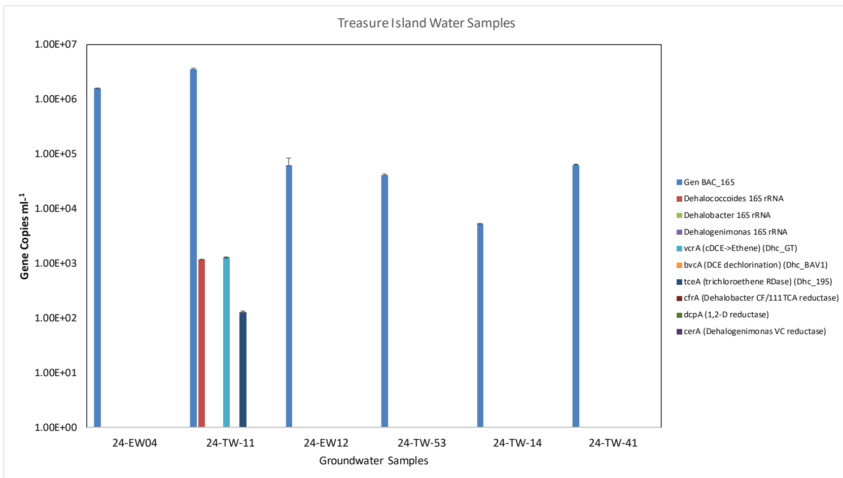
Figure 5-83. Organisms and Genes Associated with Reductive Dechlorination Detected in Wells at the Treasure Island Site.
