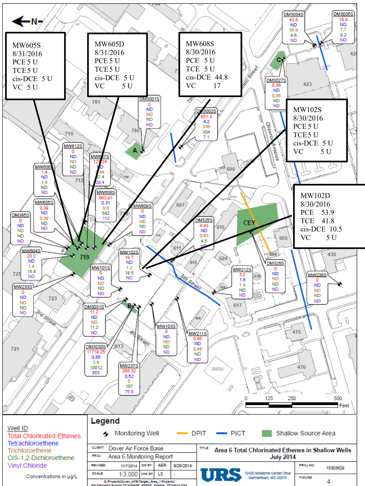
Figure 5-15. Site Plan. Dover Air Force Base Area 6.
