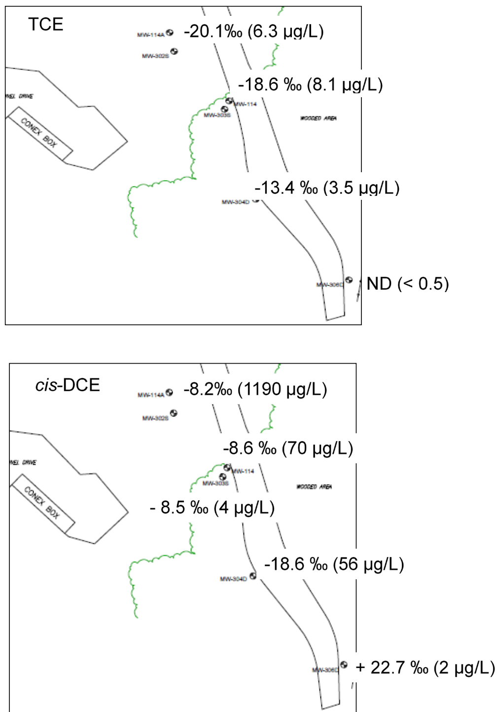
Figure 5-11. Overhead View of the Well Locations, VOC Concentrations (Top Panel; TCE, Bottom Panel; cis-DCE), and \delta^{13}\text{C} Values for the Relevant VOCs.
