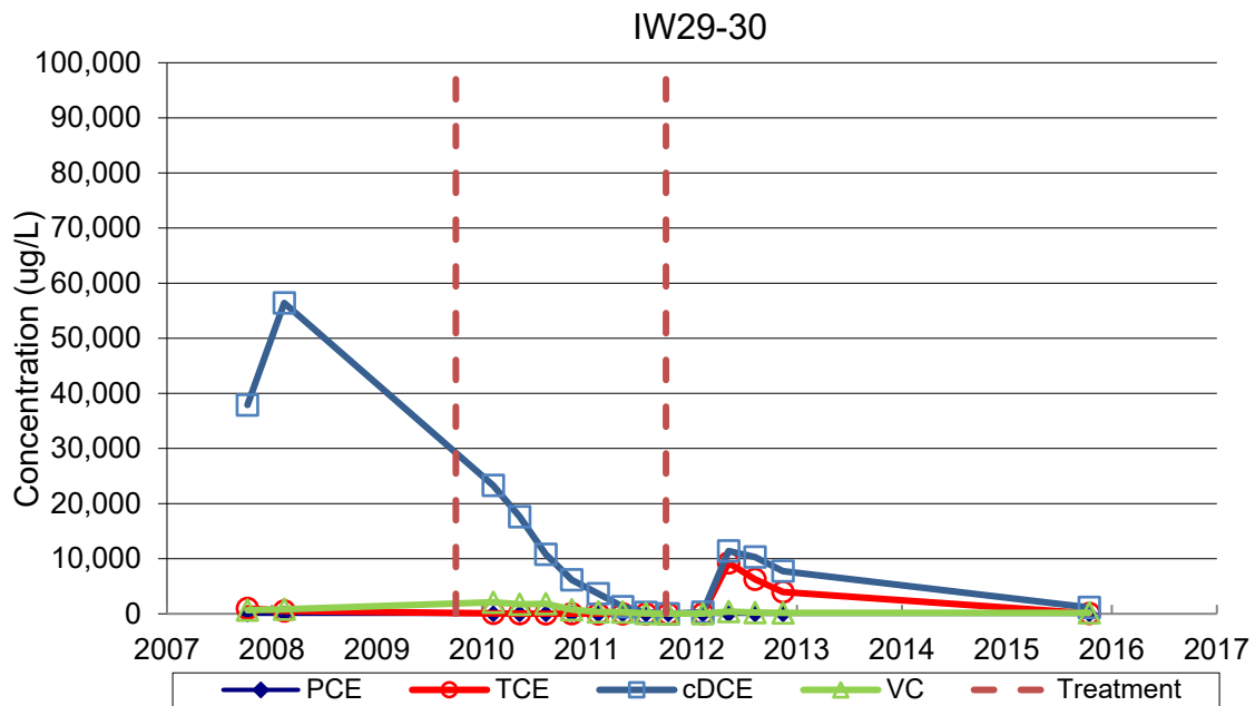
Figure 5-31. VOC Trends for IW29-30, Former Charleston Air Force Base Zone 4.
