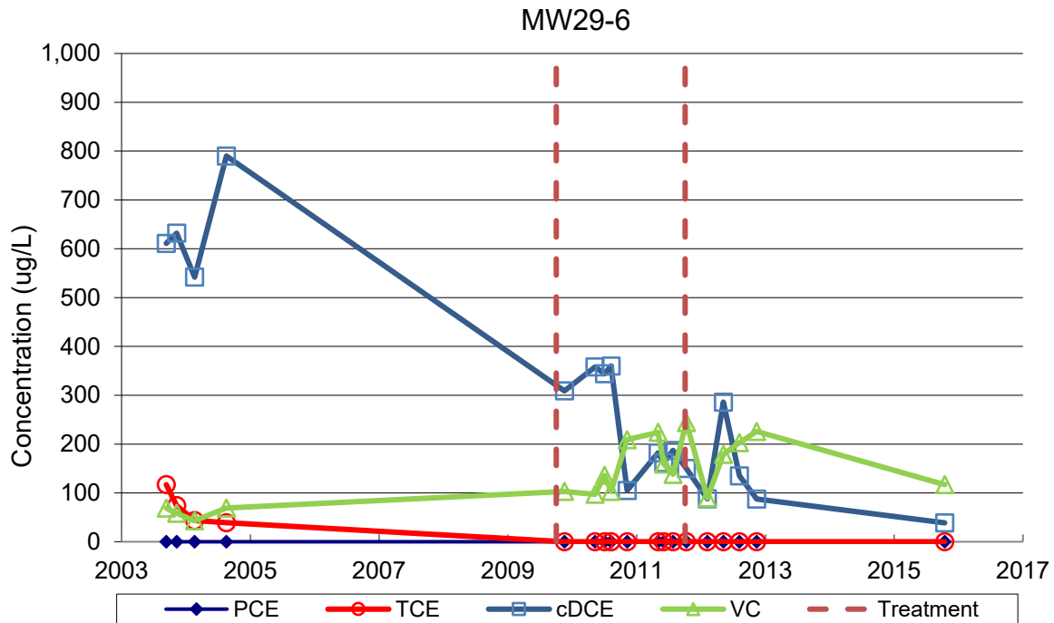
Figure 5-37. VOC Trends for MW29-6, Former Charleston Air Force Base Zone 4.
