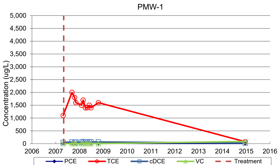
Figure 5-58. VOC Trends for PMW-1, Seal Beach Naval Weapons Station Site 70.
