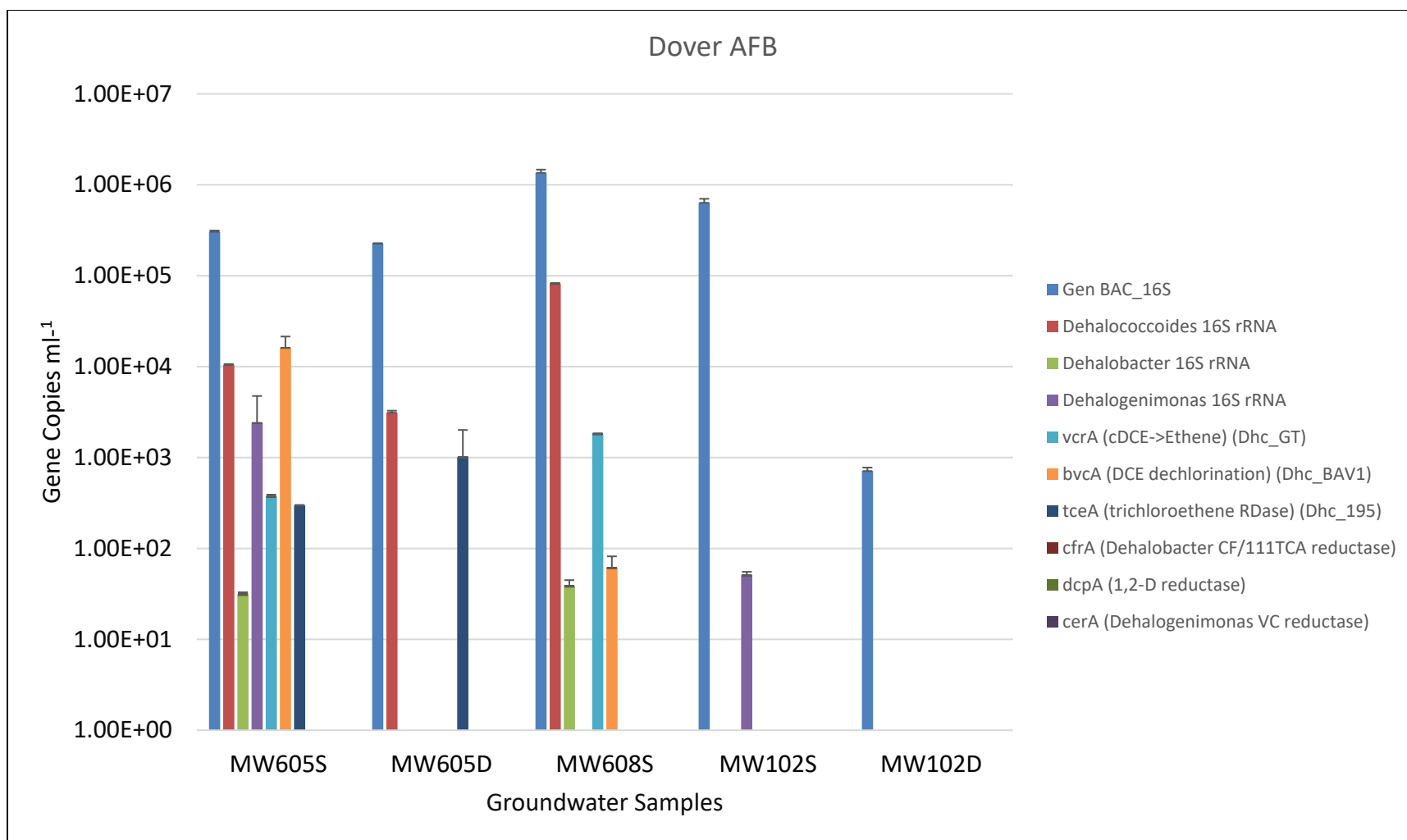
Figure 5-25. Organisms and/or Genes Associated with Reductive Dechlorination Detected in Wells at Dover Air Force Base Area 6.
