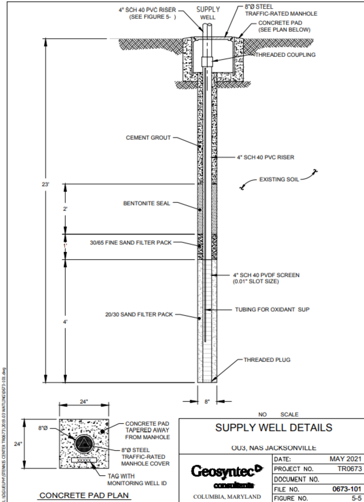
Figure 5-5. Supply Well Details
