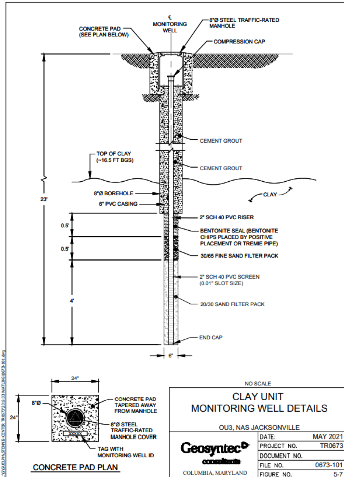
Figure 5-7. Clay Unit Monitoring Well Details
