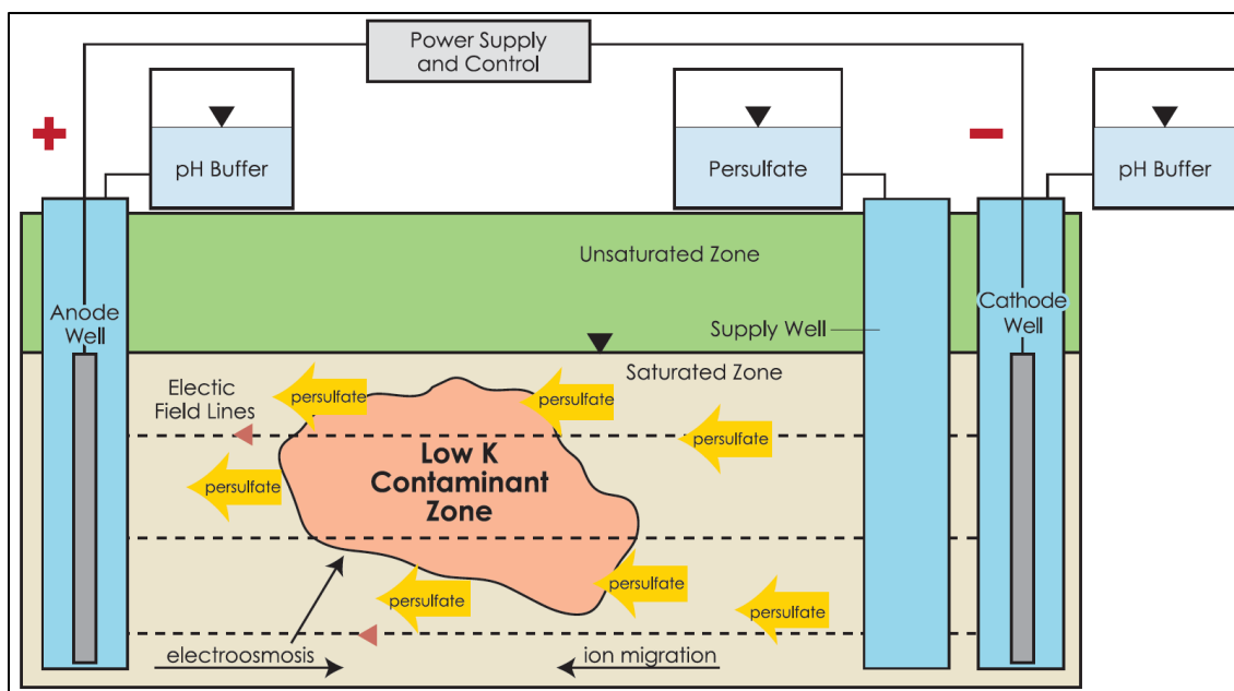
Figure 2-2. Schematic of EK-Enhanced Amendment Delivery Technology
