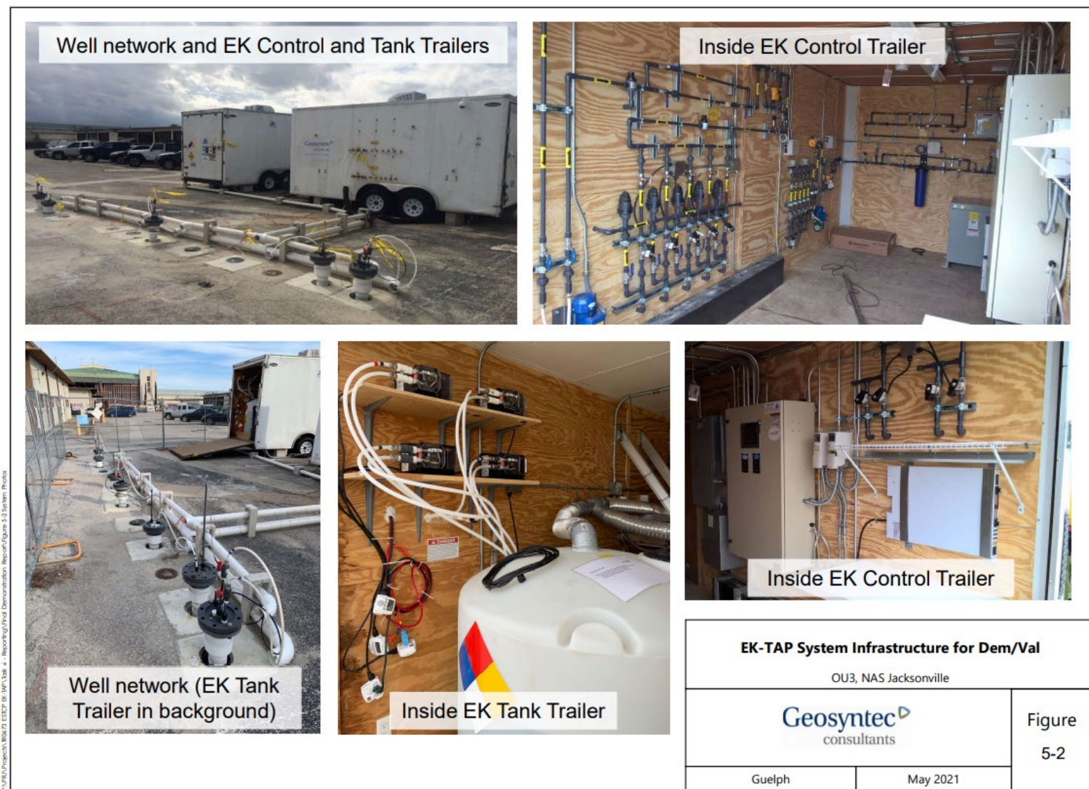
Figure 5-2. EK-TAP System Infrastructure for Dem/Val
