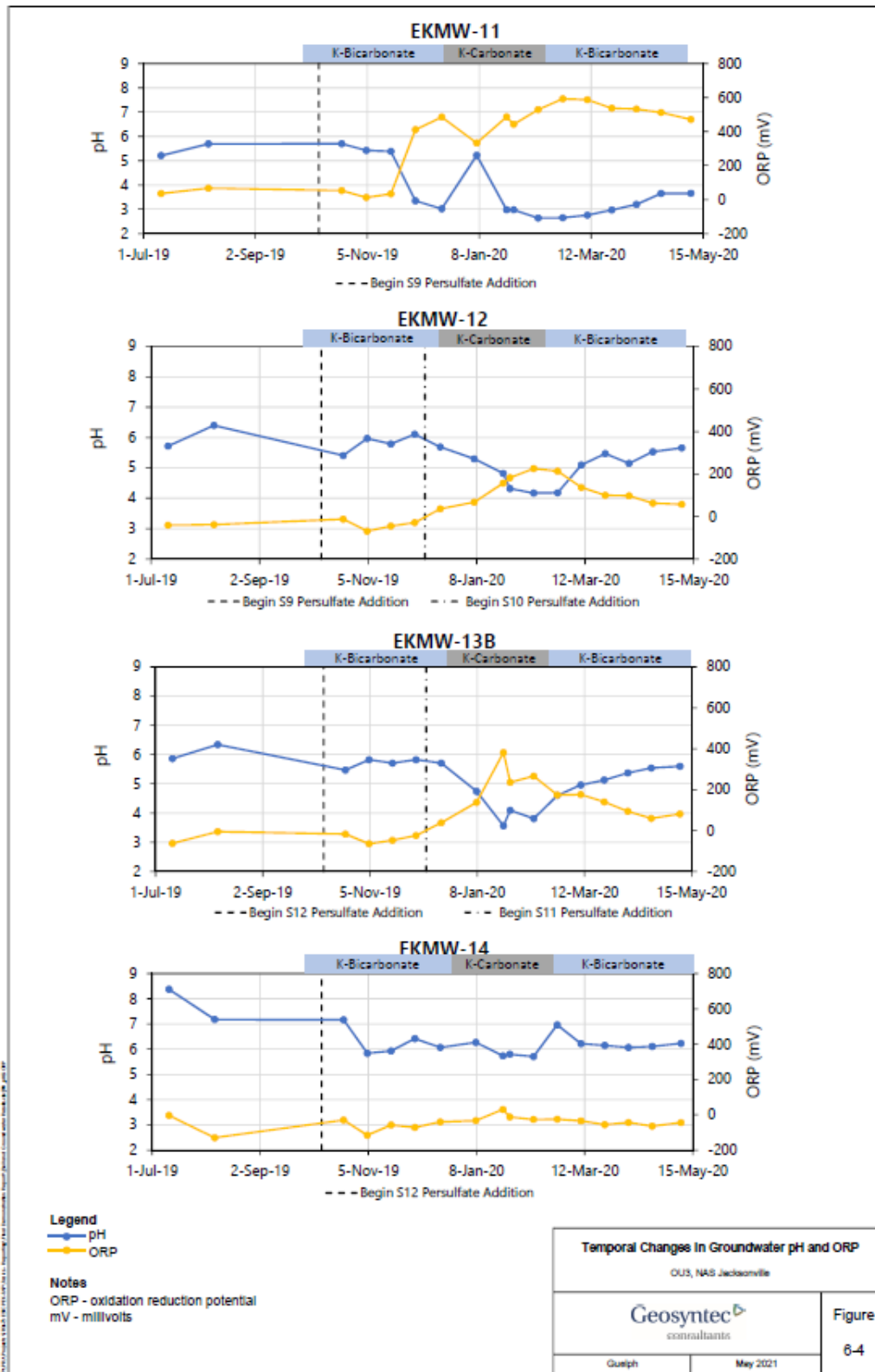
Figure 6-4. Temporal Changes in Groundwater pH and ORP
