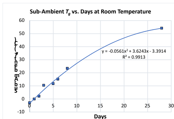
Figure 1: B-stage T_g temperature of prepreg aged at room temperature.
