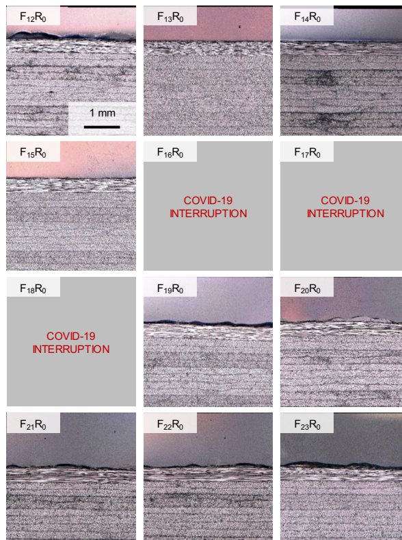
Figure 4: Micrographs of laminates produced from freezer aged prepreg using the MRCC.
