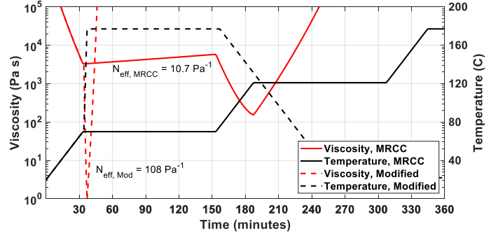
Figure 7: Viscosity profiles and corresponding effective flow number of overaged prepreg ( T_g = 15.8^\circ \text{C} ) cured using the MRCC and a modified cure cycle.
