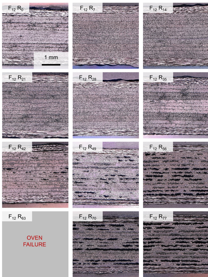
Figure 2: Micrographs of laminates produced from room temperature aged prepreg using the MRCC.
