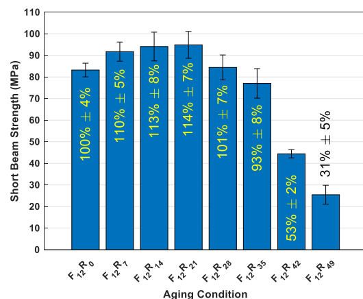
Figure 3: Average short beam strength of laminates aged at room temperature (labels indicate strength normalized against the F_{12}R_0 case).
