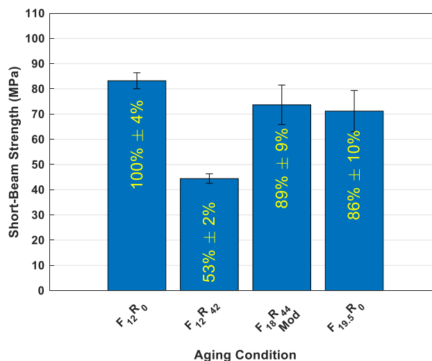
Figure 10: Short beam strength for laminates produced from prepreg with various aging conditions processed using the MRCC ( F_{12}R_0 , F_{12}R_{42} , F_{19.5}R_0 ) and a modified cure cycle ( F_{18}R_{44} Mod).
