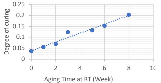
Figure 8. Relationship of degree of curing vs. aging time calculated by the DiBenedetto relationship
