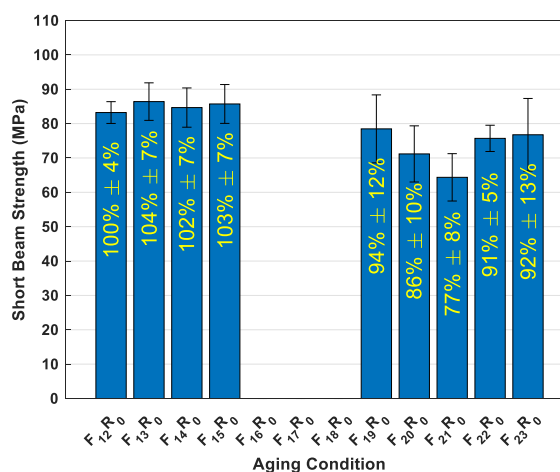
Figure 5: Average short beam strength of laminates aged in the freezer (labels indicate strength normalized against the F 12 R 0 baseline case).
