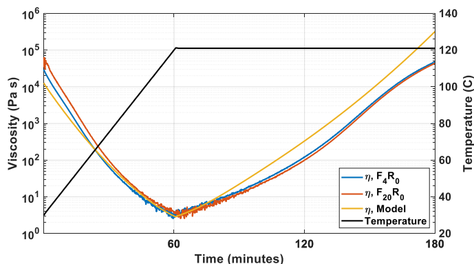
Figure 6: Viscosity profile of resin squeezed from prepregs with different aging conditions.
