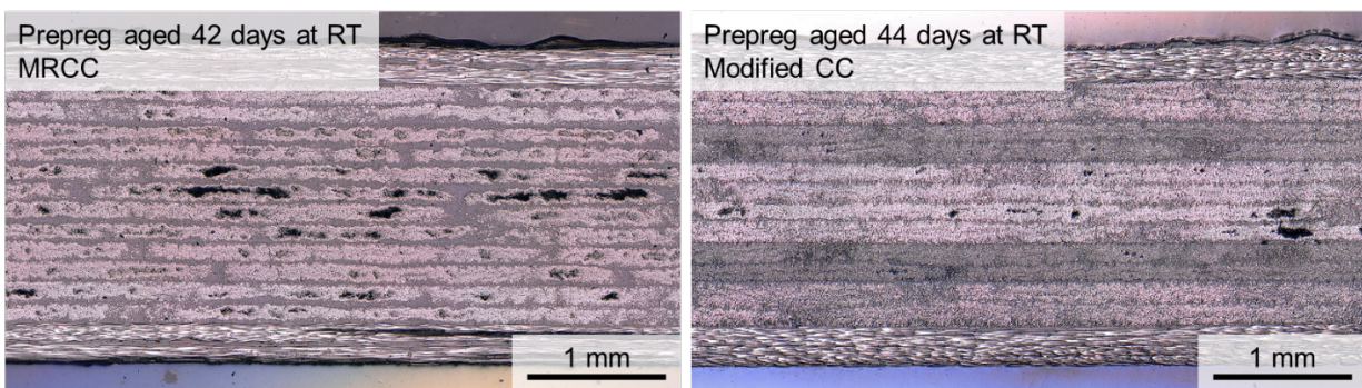
Figure 9: Comparison of microstructure in laminates produced from (left) prepreg aged for 42 days at room temperature, cured using the MRCC and (right) prepreg aged for 44 days at room temperature, but cured using the modified cure cycle show in Figure 7.
