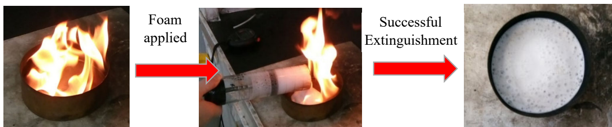
Figure 5.4. Laboratory small scale fire test. (a) 10 s preburn, (b) application of foam, (c) measurement of extinguishment and burnback.
