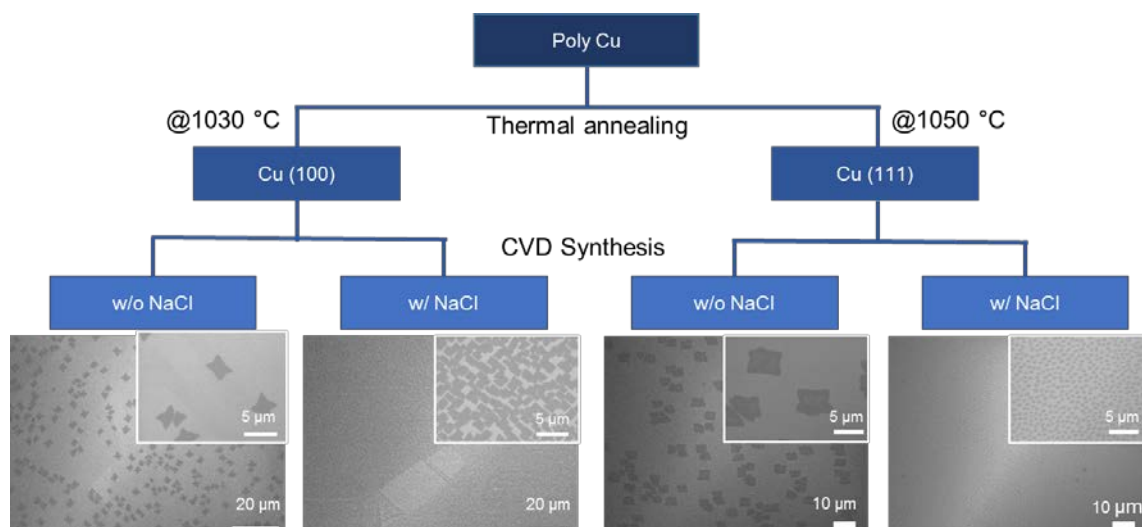
Figure 9. SEM images of graphene flakes on Cu(100) and Cu(111) without and with NaCl additive
