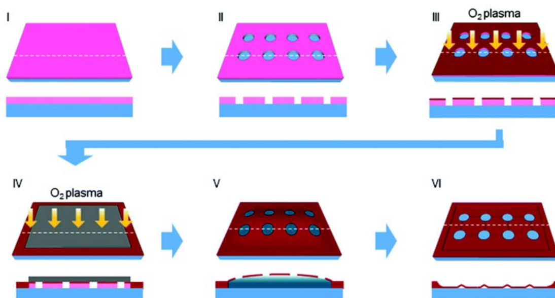
Figure 1. Hardening and wrinkling of a thin polymer film. Schematics of the overall process: patterning of the hole array (I and II), hardening (III and IV), and wrinkling (V and VI). Bottom panels: cross-sectional structures along the dashed lines in the top panel. Note that position of the dashed line in (VI) is different from those in (I-V).
