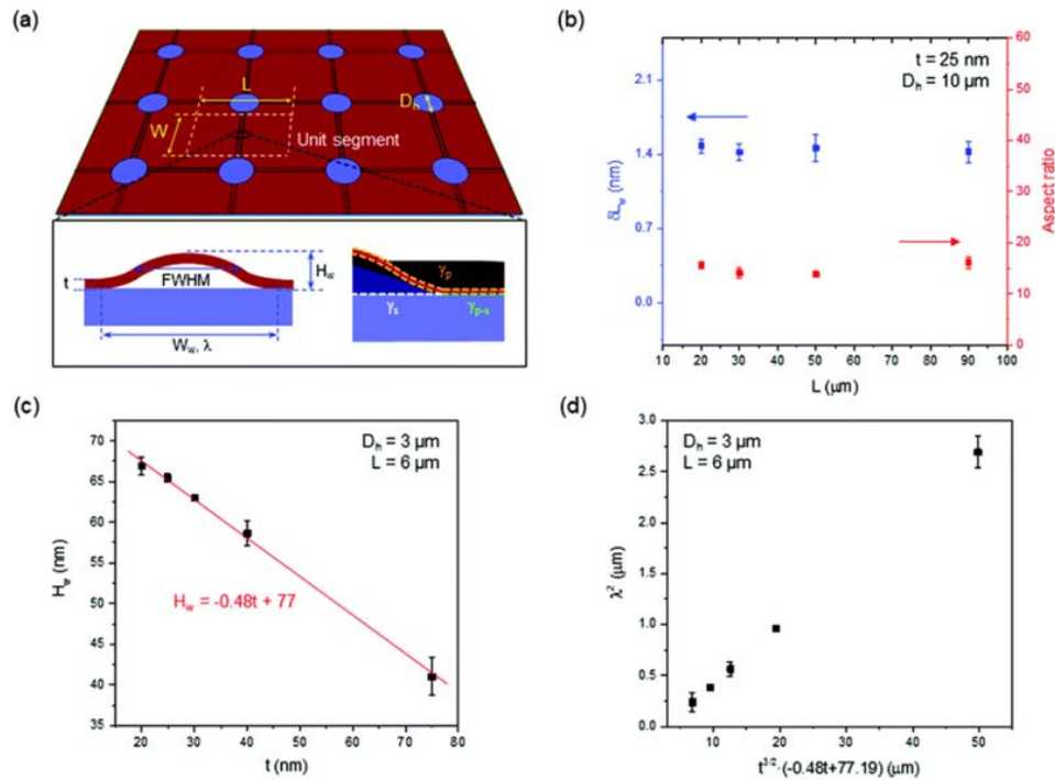
Figure 16. Analysis of the wrinkles. (a) Schematic images of the wrinkle structure with geometry and definitions of the parameters: hole diameter ( D_h ), center-to-center distance ( D_c ), length ( L ) and width ( W ) of a unit segment, film thickness ( t ), wrinkle height ( H_w ), wrinkle width ( W_w ), elongated length ( \delta L_w ), polymer surface ( \gamma_p ), substrate surface ( \gamma_s ), and polymer-substrate ( \gamma_{p-s} ). (b) The \delta L_w (blue squares) and aspect ratio (red squares) as a function of L . (c) The relationship between H_w and t ( H = -0.48t + 77 ) of wrinkles. (d) Plot of \lambda^2 versus t^{3/2} \cdot (-0.48t + 77) of wrinkles.
