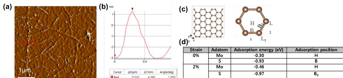
Figure 22. (a) AFM analysis of graphene/MoS 2 heterostructure. (b) Height profiling from red line of (a). (c) Graphene lattice modeling in DFT calculation. (d) Adhesion energy analysis of Mo and S atoms at strain-free graphene and 2% strained graphene.
