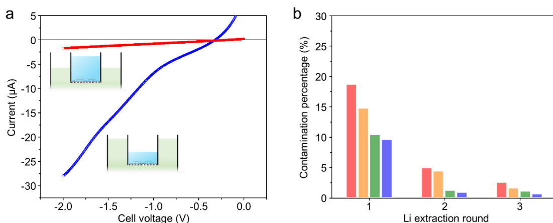
Figure 26. Operation of the system designed by the scaling-up and energy-efficiency strategies. (a) Current polarization curves depending on solution level difference. (b) ICP-MS analysis on the solutions collected after each filtering round.
