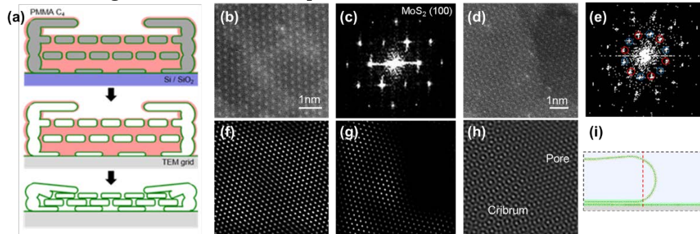
Figure 23. (a) Schematic of the processing steps (PMMA coating, silica etching, and PMMA removal with acetone vapor) for preparing TEM specimens. (b) ADF STEM image of the honeycomb lattice structures, which are observed in the inner hole region of the diatom cribrum. (c) FFT image of the Mo atom arrangement with a 3.1 Å lattice parameter, which corresponds to the monolayer MoS 2 (100) plane. (d) ADF STEM image of the boundary between the inside and outside of the holes in the diatom frustules. The inside of the holes shows the continuous hexagonal lattice patterns, while the outside exhibits a Moiré interference pattern. (e) FFT image of the entire region exhibiting two sets of hexagonal diffraction patterns (red and blue circle). iFFT patterns of each different MoS 2 monolayer, corresponding to red (f) and blue (g) circles, respectively. (h) iFFT image of both of (100) spots from the FFT patterns. (i) Schematic illustrating the sticking phenomenon of MoS 2 layers on the multidimensional valves, as determined by TEM analysis
