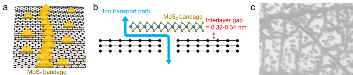
Figure 4. The structure of MFs-on-MLGDs membrane. (a) Schematic illustrating the membrane structures of MFs-on-MLGDs membrane. (b) Cross-sectioned images of the MFs-on-MLGDs membrane describing the ionic transport path. (c) SEM images of the MFs-on-MLGDs membrane.
