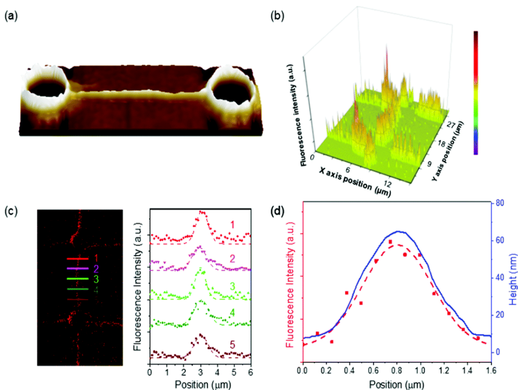
Figure 17. Utilization of polymer wrinkles as nanofluidic channels. (a) 3D AFM image of wrinkle via analysis. (b) Position-dependent fluorescence intensity map showing the distribution of the fluorescent dye along the linear and circular wrinkles. (c) Fluorescence image and the cross-sectional profiles of the fluorescence intensity at five locations. (d) Overlap of fluorescence intensity (red dots and dashed line) and height profile of the wrinkle (blue line).
