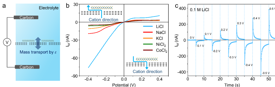
Figure 25. The scaling-up and energy-efficiency strategy using MFs-on-MLGDs membrane. (a) Schematic illustrating I_M -V measurement system. (b) I_M -V curves depending on the electrolytes. (c) Chronoamperometry.
