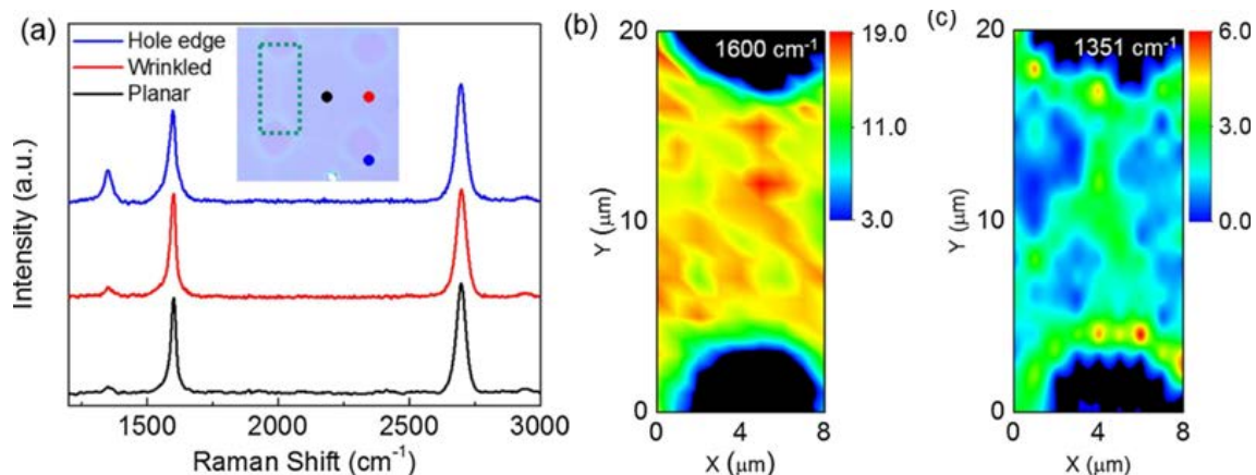
Figure 19. Raman spectroscopy analysis. (a) Raman spectra from different regions of Gr in the OM image (inset): circular edge (blue), wrinkled (red) and planar (black) regions. (b) and (c) Raman mapping images of the G peak ( 1600\text{ cm}^{-1} ) and D peak ( \sim 1351\text{ cm}^{-1} ), collected at the dotted square area of the OM image shown in the inset of (a).
