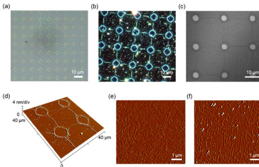
Figure 18. Structural characterization of Gr wrinkles. (a) Bright field and (b) dark field OM images, (c) SEM image, and (d) 3D AFM image of the square lattice pattern of Gr wrinkles. Hole diameters/center-to-center distances: 2 \mu\text{m} /10 \mu\text{m} (a), 8 \mu\text{m} /20 \mu\text{m} (b), 4 \mu\text{m} /16 \mu\text{m} (c) and 8 \mu\text{m} /20 \mu\text{m} (d). "(e), (f) AFM images comparing the planar region surrounded by wrinkles in (d) and that of conventional wet-transferred Gr.
