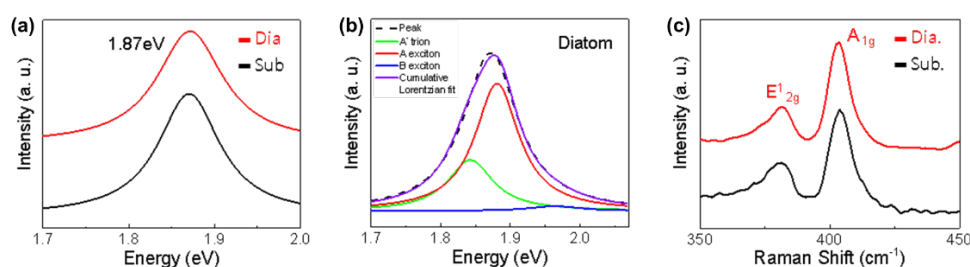
Figure 24. PL and Raman analysis of the MoS 2 diatom frustule. (a) Typical PL spectra of MoS 2 films on the Si/SiO 2 substrate (black curve) and the diatom frustule (red curve). (b) PL spectrum of the MoS 2 film on the diatom frustule fitted with three Lorentzian peaks at 1.83 eV (A - trion), 1.88 eV (A exciton), and 2.03 eV (B exciton). (c) Raman spectra of MoS 2 films.
