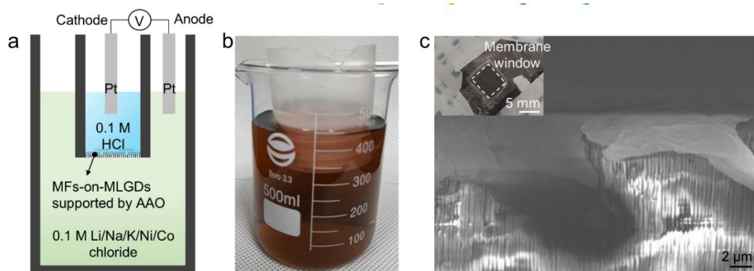
Figure 5. The scaling-up and energy-efficiency strategy using MFs-on-MLGDs membrane. (a) Schematic illustrating the homemade system. The MFs-on-MLGDs membrane separates the acidic solution and mixed solution. (b) Photograph of the homemade system. (c) SEM images showing the MFs-on-MLGDs membrane supported by AAO substrate. The inset is the photograph of MFs-on-MLGDs membrane fixed with the PDMS well.
