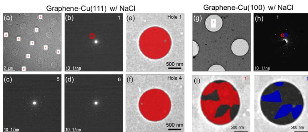
Figure 10. (a) Low magnification TEM images of graphene grown on Cu (111) with the NaCl additive. (b-d) SAED patterns collected at the holes labelled in (a). (e, f) False color DF-TEM images of the holes 1 (e) and holes 4 (f) labelled in (a), recorded with the same diffraction spot marked by red circle in (b).
