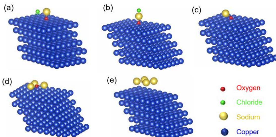
Figure 8. Effects of NaCl adsorption on a Cu(111) surface by DFT calculations. (a,b) NaCl adsorption on a Cu(111) surface with an adsorbed O atom. (c-e). [\text{Na}^+] is shown to assist in desorbing the oxygen atom adsorbed on the Cu(111) surface.
