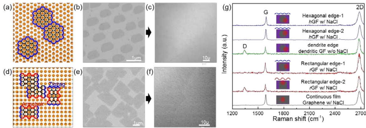
Figure 13. (a) Atomic configuration of hGFs on Cu (111) and (b, c) corresponding SEM images of GFs and continuous graphene film. (d) Atomic configuration of rGFs on Cu (100) and (e, f) SEM images of rGFs and graphene. (g) Raman spectra measured at the edges of hGFs (blue), dendrites (green), rGFs (red), and continuous graphene (black).
