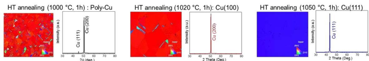
Figure 6. EBSD images and XRD curves for Cu foils with high temperature annealing at (a) 1000°C (b) 1020°C and (c) 1050°C for 1 hour.
