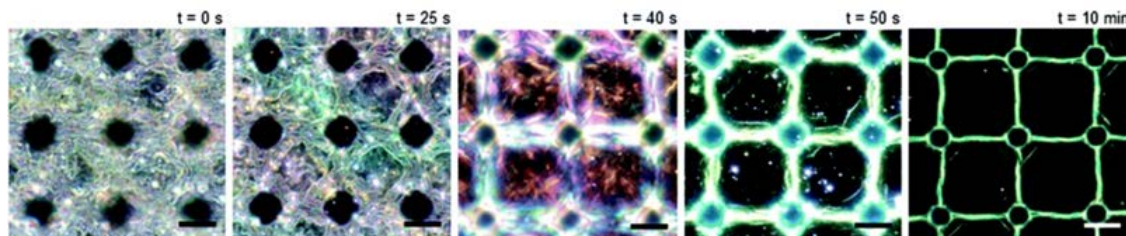
Figure 14. Hardening and wrinkling of a thin polymer film. In situ dark field microscopy images taken during wrinkling of a 25 nm thick polymer film from 0 to 10 min. Scale bars: 5 \mu\text{m} .
