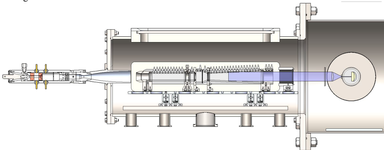
Figure 3. OH-PLIF optical setup in freejet-model configuration.
