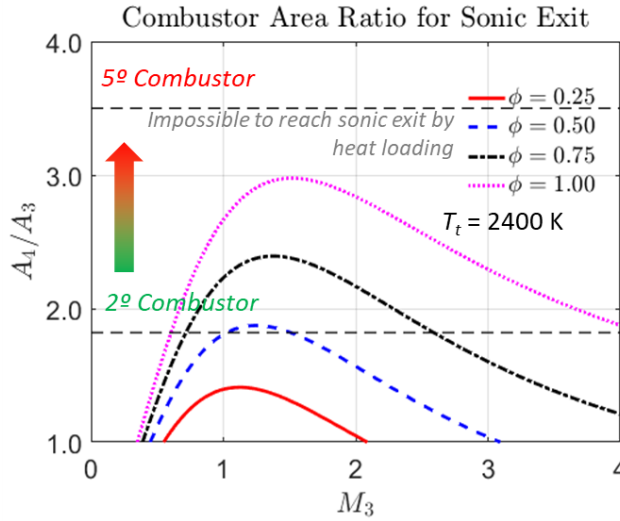
Figure 13. Scramjet operational diagram with the sonic condition at combustor exit.
