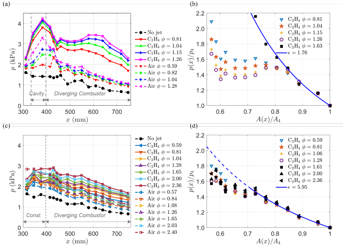
Figure 17. Pressure distributions in a model scramjet with a) a cavity flameholder, and c), d) without a cavity flameholder.
