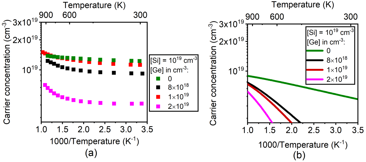
Figure 3: (a) Temperature-dependent free carrier concentration in Al 0.65 Ga 0.35 N as a co-doped with constant [Si] of \sim 1 \times 10^{19} \text{ cm}^{-3} and variable [Ge]. (b) Calculated temperature-dependent free carrier concentration simulating doping concentration in Figure 3 (a) but assuming coexistence of Ge -1 and Si + . Notably, the expected behavior is completely different from the experimental data.
