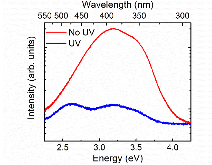
Figure 1. Room temperature photoluminescence spectra for Si-implanted AlN annealed without (red) and with (blue) UV illumination, showing more than one order of magnitude reduction in V_{\text{Al}}\text{-nSi}_{\text{Al}} -related point defects. The spectra were normalized with respect to the band edge luminescence to facilitate direct comparison of the midgap luminescence peaks.
