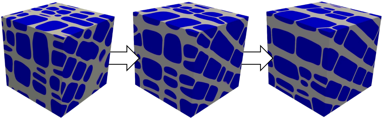
Figure 18 : Phase-field simulation of a creep test at 1050°C/180 MPa on the \langle 011 \rangle -oriented RVE presented in the previous figure.
