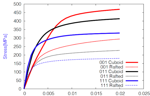
Figure 19: Crystal-plasticity finite-element simulations of a monotonic tensile tests at 10^{-3} \text{ s}^{-1} 1050°C for different orientations and microstructural states.
