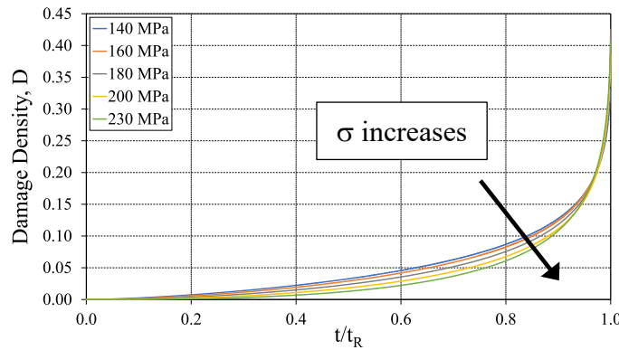
Figure 11: Evolution of the new damage variable D as a function of the time fraction t/t_R at 1050°C for the simulated curves. t_R is the simulated time at rupture.
