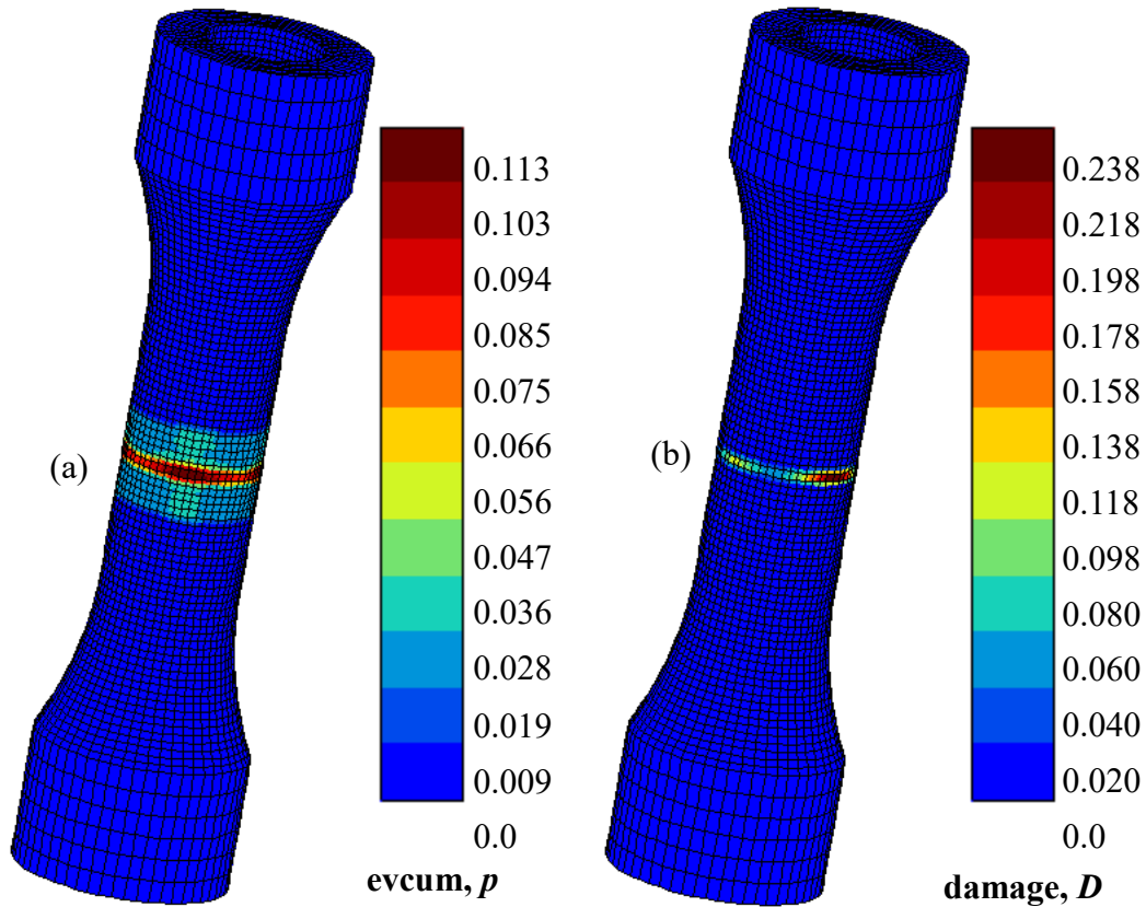
Figure 14: (a) Accumulated plastic strain and (b) damage distribution at rupture ( N_{f-predicted}=855 ) for a tube subjected to tension/torsion at 1050^{\circ}\text{C}/\sigma_{Mises}=113\text{ MPa} .
