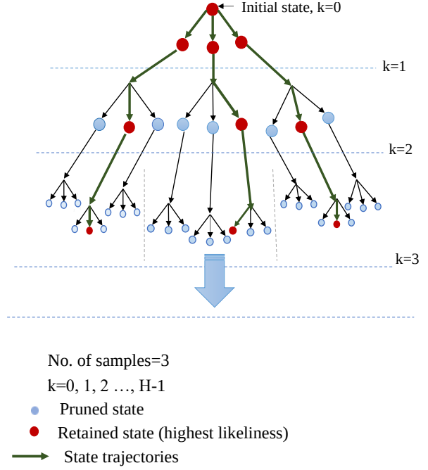
Fig. 5: Sampling in RS-MHP approach with pruning (3 nodes allowed to remain at each stage).
