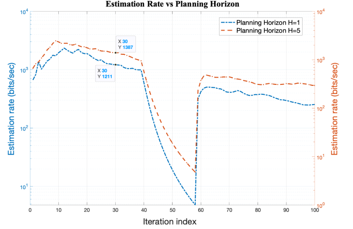
Fig. 5: Estimation rate vs. planning horizon
