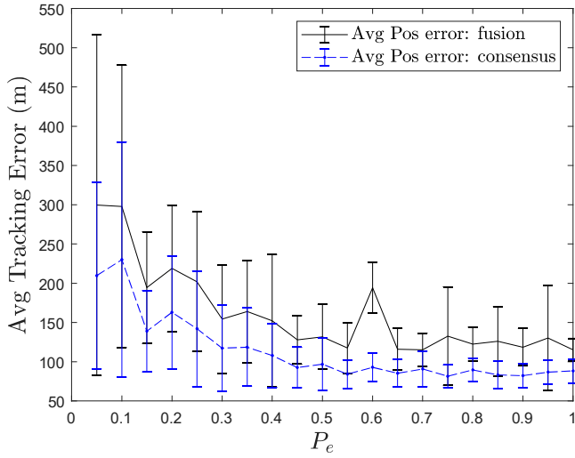
Fig. 5. Average tracking error across all sensors with respect to edge probability P_e
