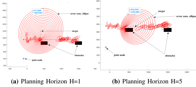
Fig. 7: Myopic vs. non-myopic approach
