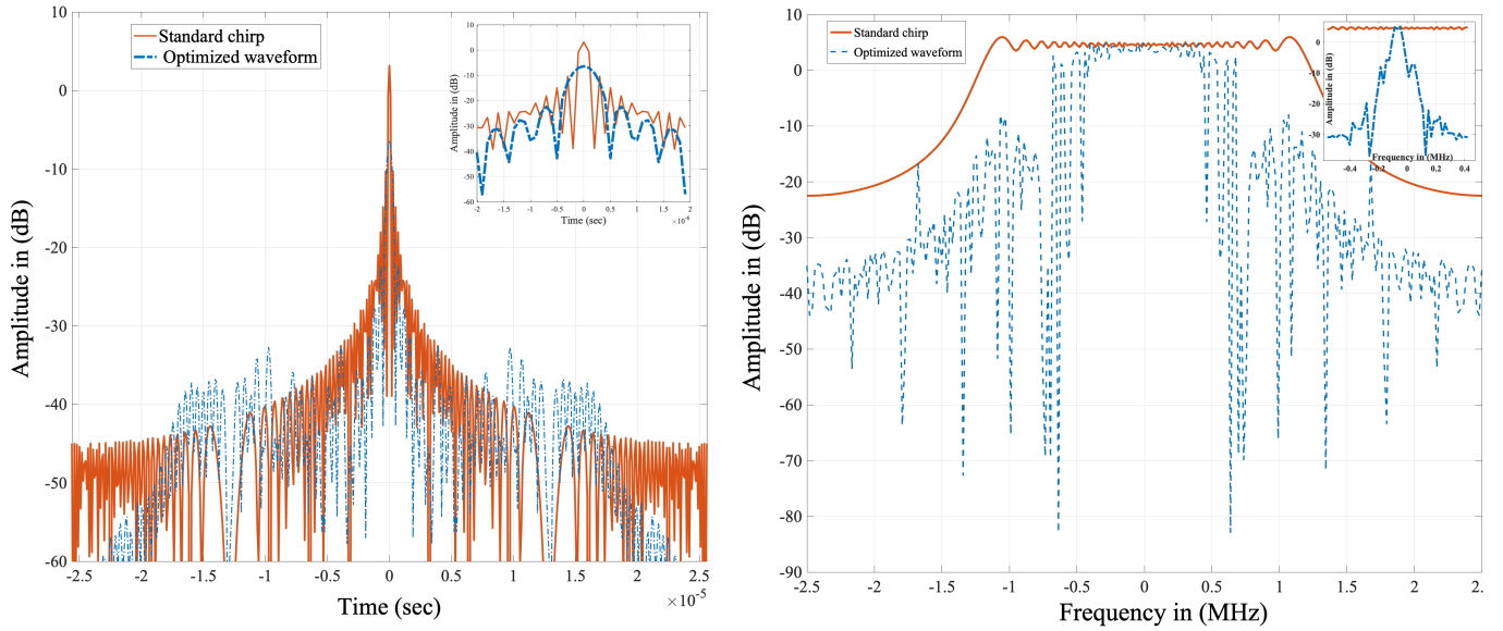
(a) Radar waveform autocorrelation function of the optimized waveform with \alpha = 0.5 and H = 1 (b) Radar waveform spectrum with \alpha = 0.5 and H = 1 . The standard chirp is depicted by the red line, and the optimal waveform spectrum is shown by the blue dotted line
