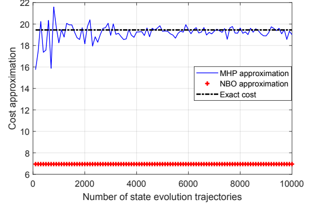
Fig. 2. MHP vs. NBO
