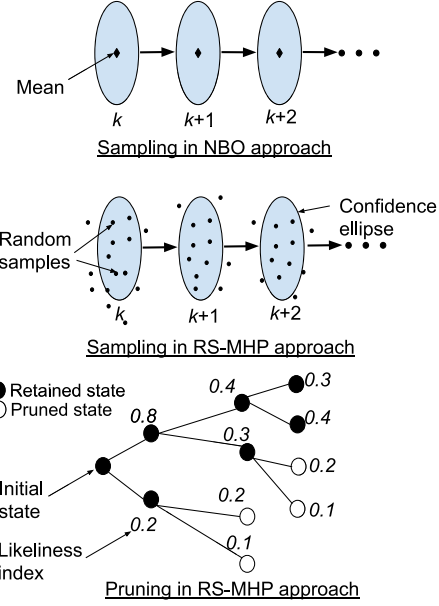
Fig. 2. Top two figures show the sampling probability distributions of noise variables: NBO vs. RS-MHP. The bottom figure shows a branch pruning strategy in RS-MHP.
