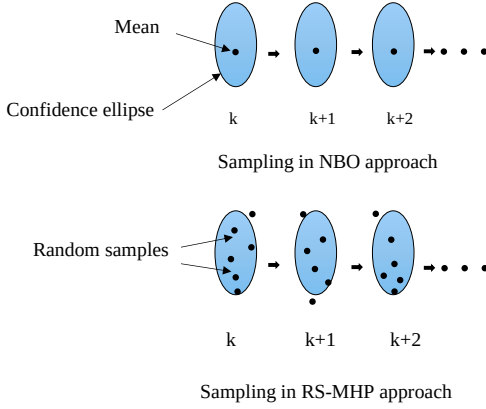
Fig. 4: Sampling in NBO vs. RS-MHP approach
