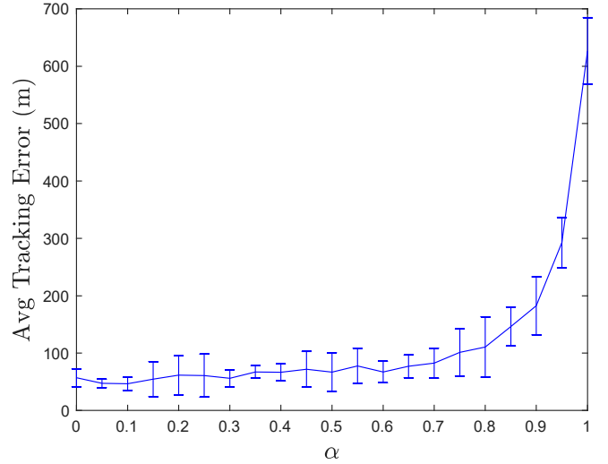
Fig. 7. Average tracking error across all sensors with respect to weighting parameter \alpha
