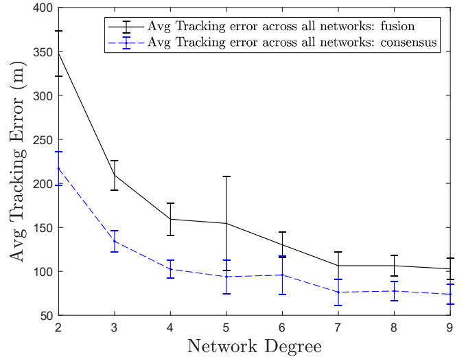
Fig. 4. Average tracking error across all sensors for configuration I
