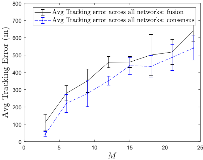
Fig. 2. Average tracking error across all sensors with respect to number of time steps, M
