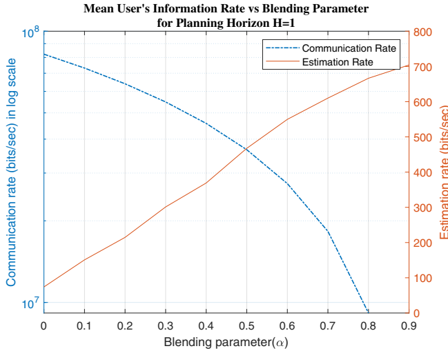
Fig. 4: Average rate vs. \alpha
