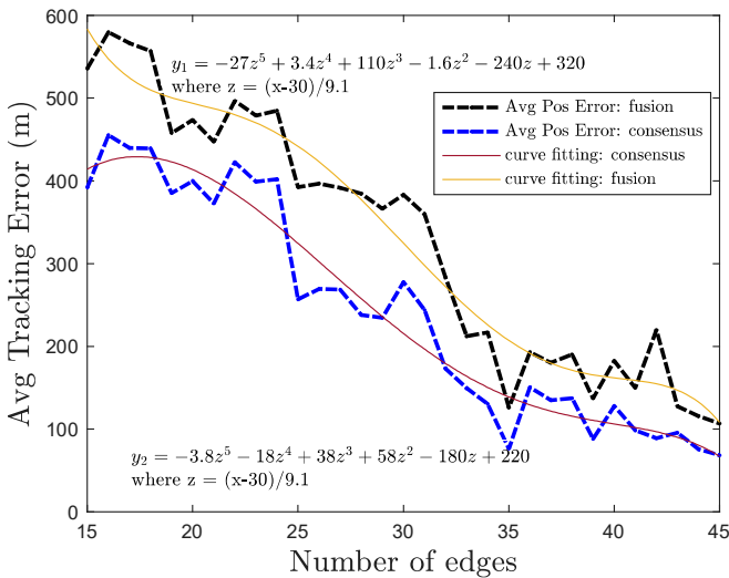
Fig. 6. Average tracking error across all sensors with respect to number of edges
