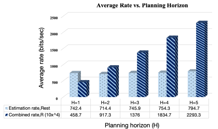
Fig. 6: Average rate vs. planning horizon
