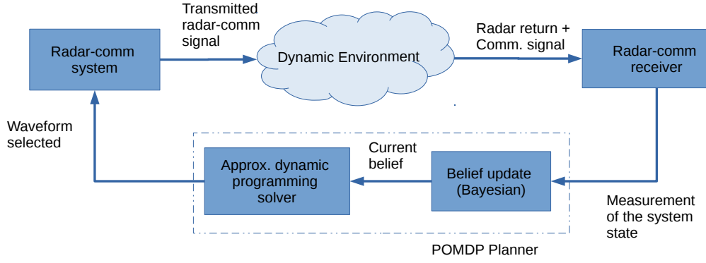
Fig. 3: Adaptive waveform optimization in a dynamic environment.
