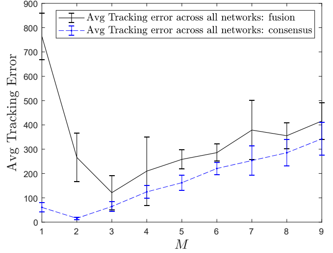
Fig. 3. Average tracking error across all sensors with respect to number of time steps, M
