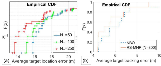
Fig. 4. (a) Cumulative distribution of average target location errors. Here N_T represents the number of state evolution trajectories. (b) Cumulative distribution of target location errors: NBO vs. RS-MHP.
