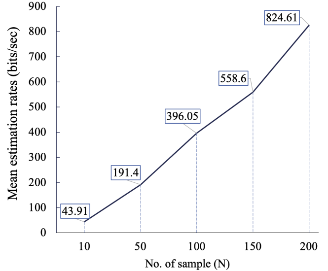
Fig. 13: Mean estimation rate vs. number of samples N \in \{10, 50, 100, 150, 200\} .
