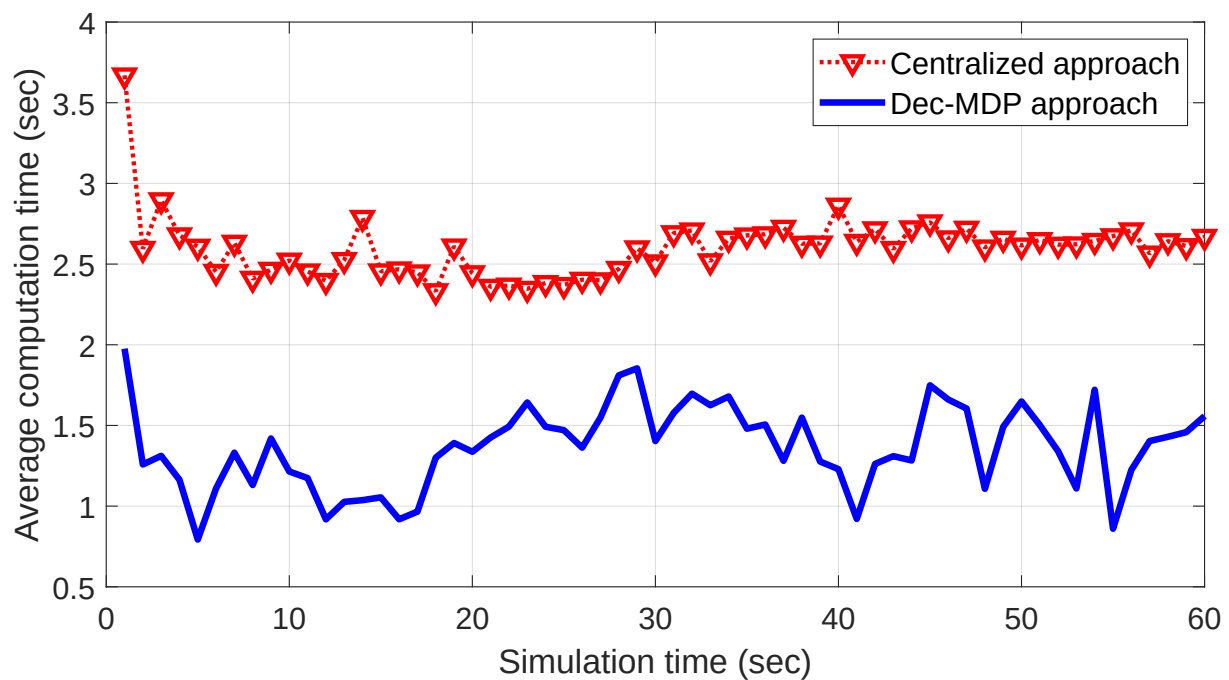
Figure 5. Computation time ( T_c ): centralized vs. decentralized method.
