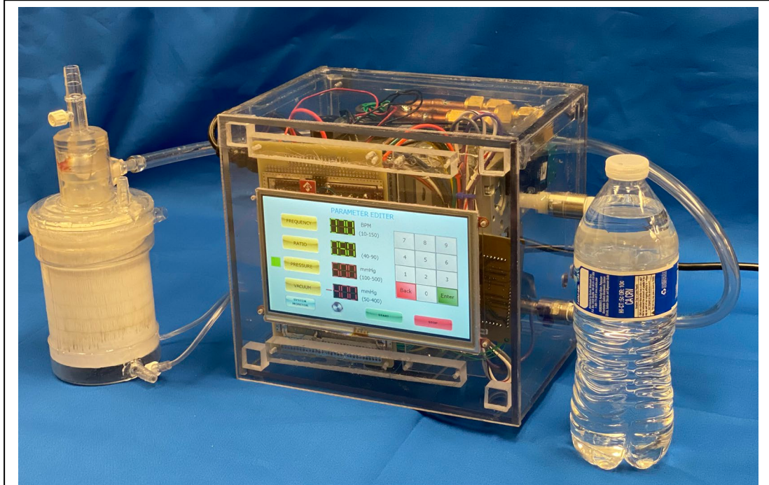
Fig 8: Very compact size of latest pPIAL system prototype.
