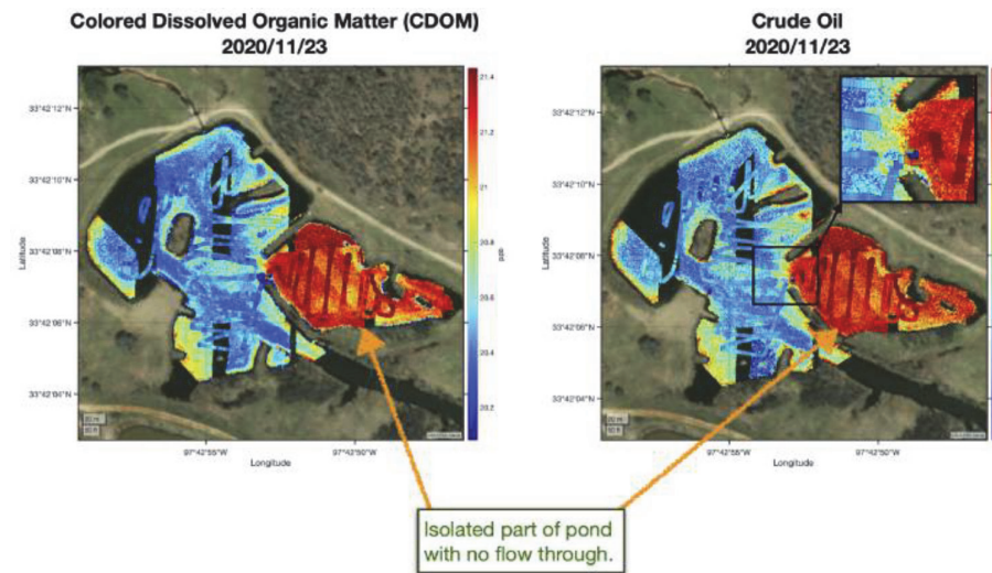
Figure 5. Example crude oil and colored dissolved organic matter (CDOM) data collected autonomously by the robot team on November 23, 2020 in North Texas. The maps show the CDOM and crude oil estimated from the hyper-spectral imager using machine learning as the background colors and the actual in-situ boat observations as the overlaid color filled squares. Note that the isolated part of the pond which has now fresh water in-flux has higher levels of CDOM and crude oil with a sharp gradient across the inlet in both the estimates using the hyper-spectral image and the boat observations.
