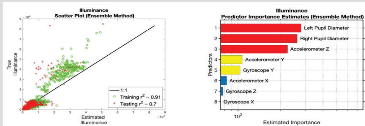
Figure 9: Plots for the illuminance model.
