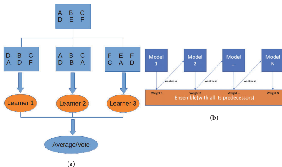
Figure 3. Schematics illustrating the various ensemble model approaches. (a) Bagging, (b) Boosting.
