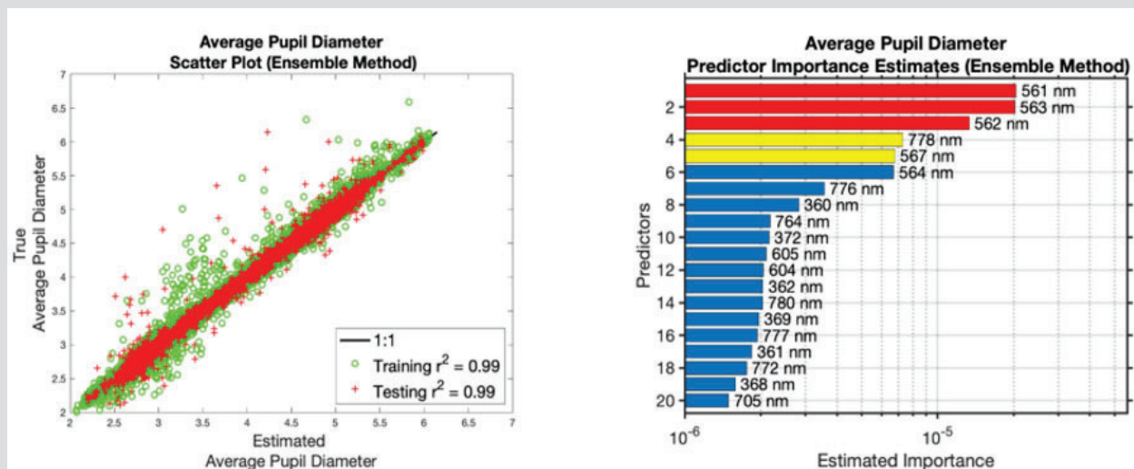
Figure 4: Plots for the average pupil diameter model.
