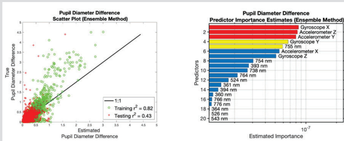
Figure 7: Plots for the pupil diameter difference model.
