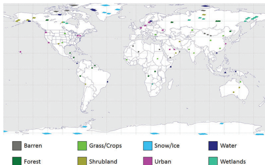
Figure 1. Global distribution of the 96 unique Landsat 8 Cloud Cover Assessment scenes, adopted from [6].
