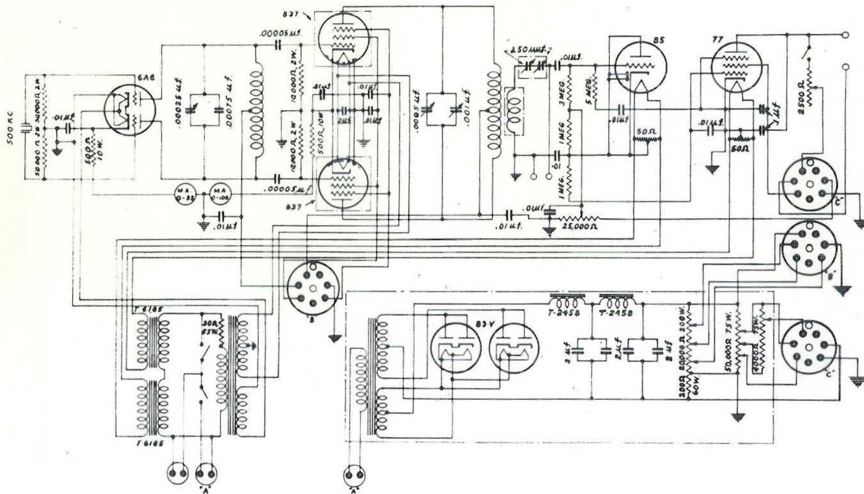
500 KC. DRIVER AND VACUUM TUBE VOLTMETER USED WITH INTERELECTRODE CAPACITANCE MEASURING EQUIPMENT.
