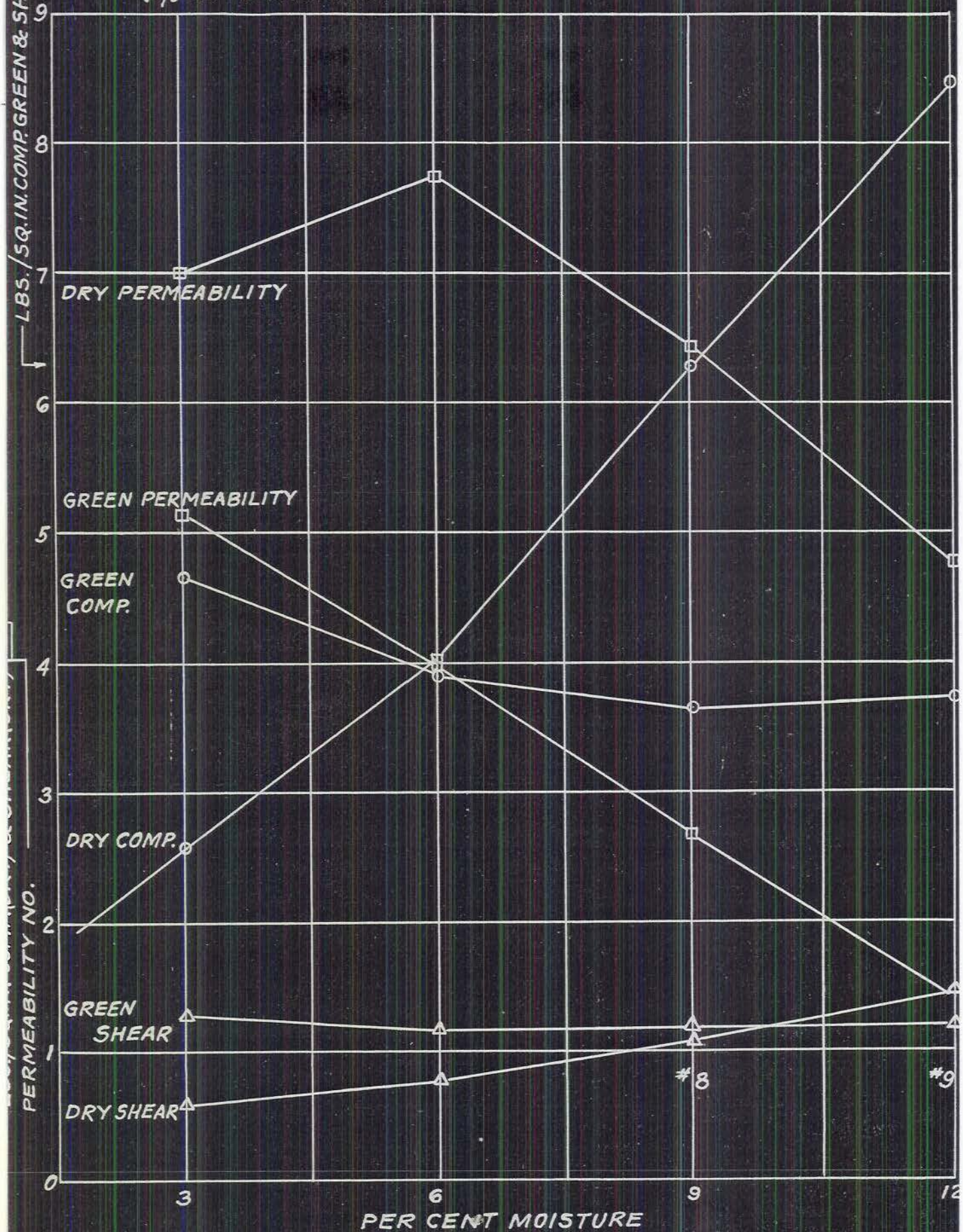
THE EFFECT OF MOISTURE ON DRY COMPRESSION STRENGTH OF SILICA SAND A.F.A. NO 63 WITH 4% OF BENTONITE.
