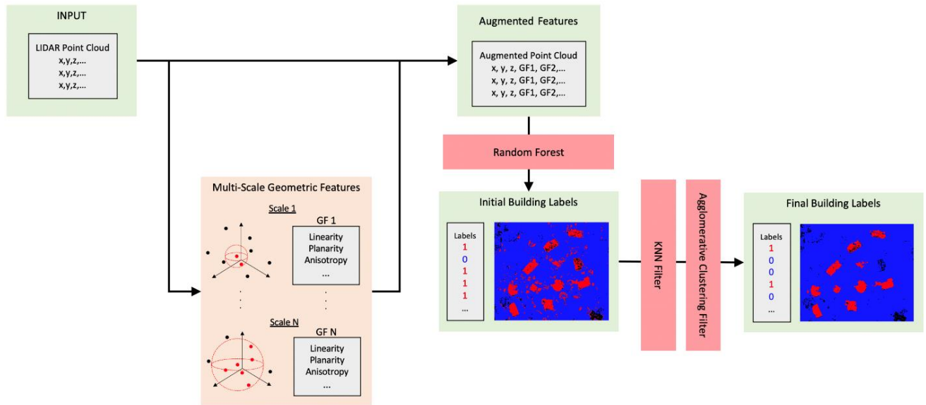
Figure 24. Building detection workflow overview.
