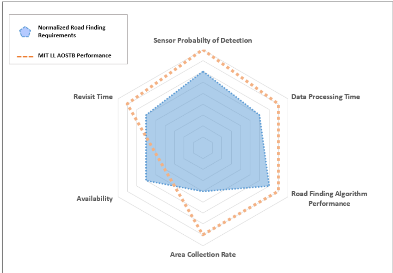
Figure 33. Spider chart depiction of requirements vs. system performance.
