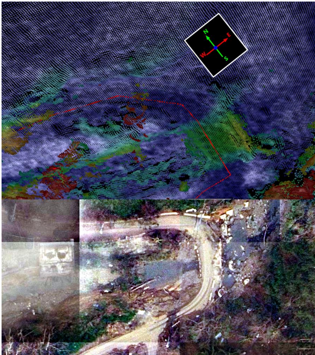
Figure 39. Bridge damage: LIDAR (top), Vexcel Visual (bottom).
