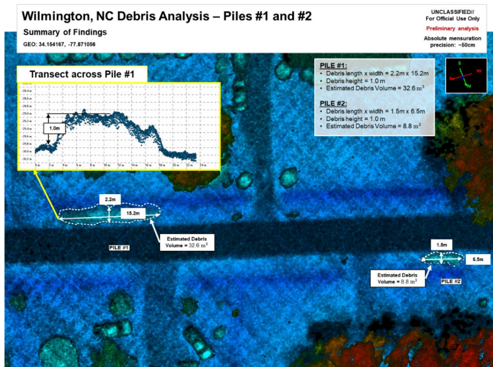
Figure 41. Mensuration of debris piles for debris quantity (volumetric) estimation.
