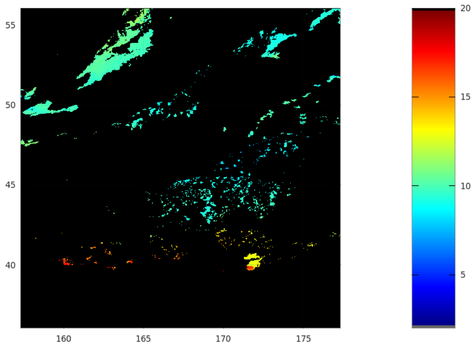
Figure 7: S-NPP/VIIRS SST retrievals on 21 July 2019 at approximately 0130 UTC. Areas that are identified as contaminated are blacked out, including the area corresponding to the Raikoke associated sub-plume.
