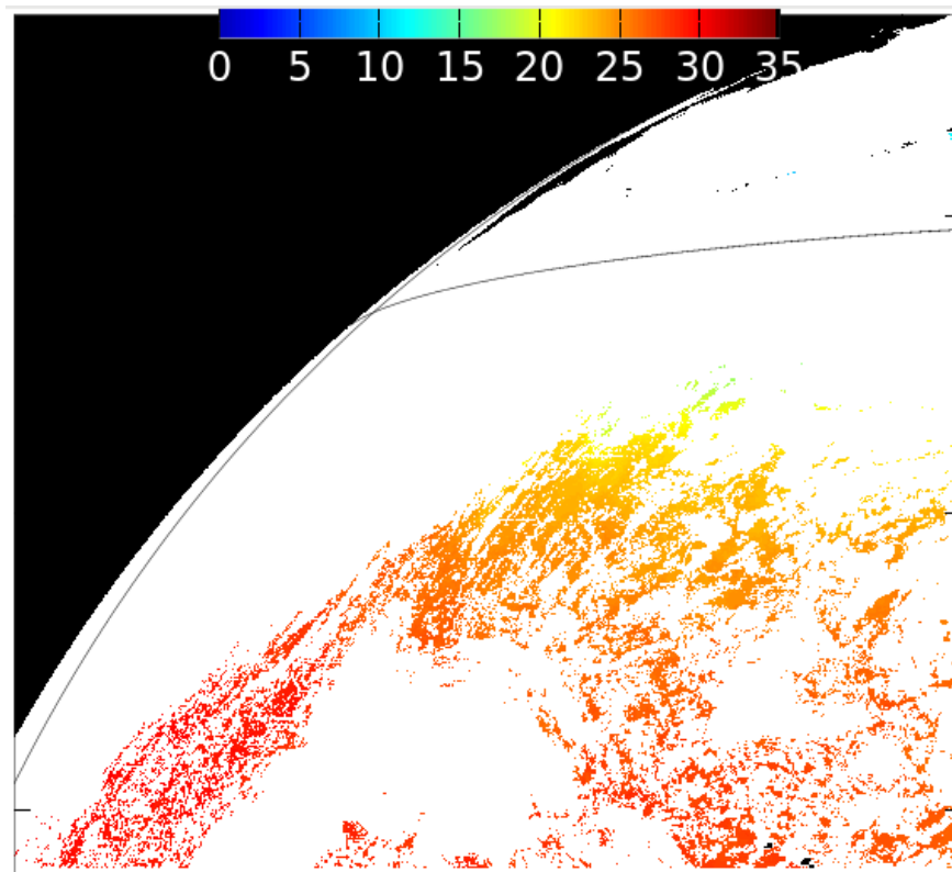
Figure 5: GOES-17/ABI SST retrievals without satellite zenith angle threshold on 21 July 2019 at 0300 UTC. The two black line indicate the latitude at 48.35^\circ\text{N} and the longitude at 153.23^\circ\text{E} with the intersection pointing to the Raikoke volcano.
