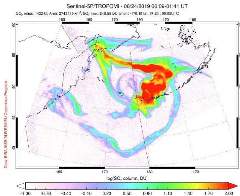
Figure 2: Sentinel-5P/TROPOMI measured \text{SO}_2 from 24 June 2019.
