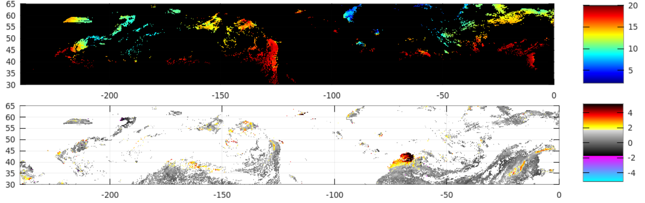
Figure 8: (Top) S-NPP/VIRS SST retrievals on 21 July 2019 from 30°N to 65°N and 120°E to 0°W. Areas identified as contaminated are blacked out. (Bottom) Corresponding SST retrieval field minus K10 background field.
