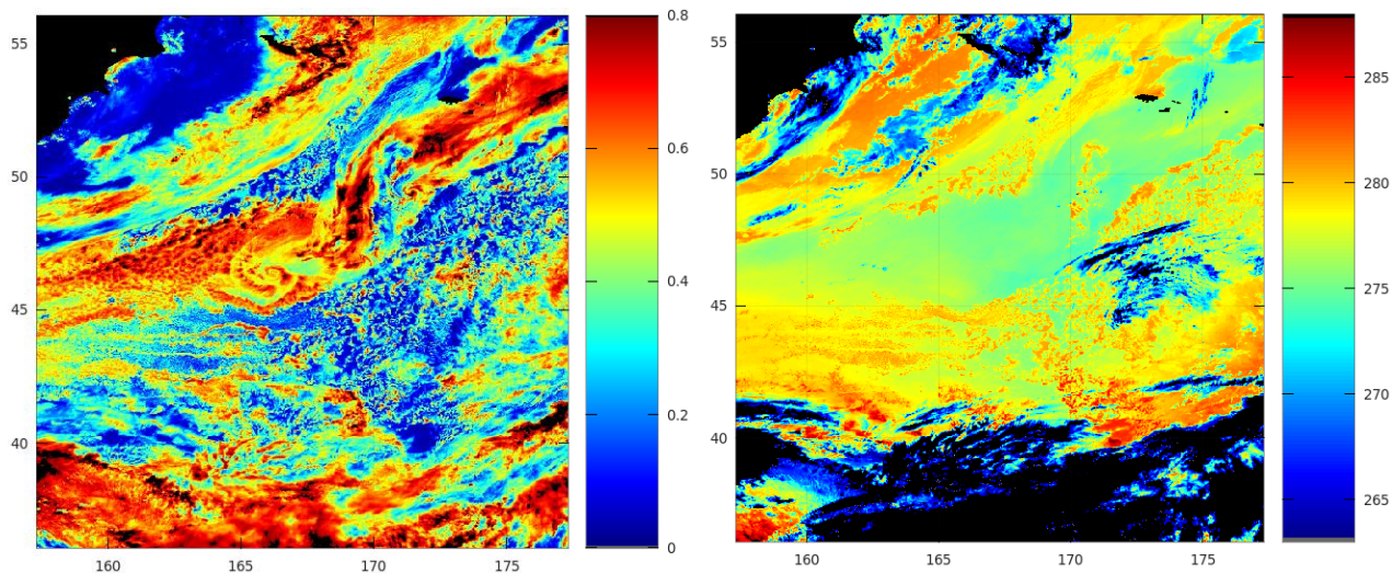
Figure 6: S-NPP/VIIRS reflectance field at 0.9 \mu\text{m} (left) and brightness temperature field at 10.7 \mu\text{m} (right) on 21 July 2019 at approximately 0130 UTC
