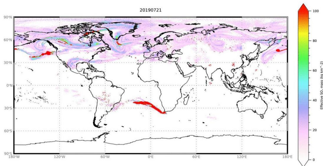
Figure 3: Effective \text{SO}_2 mass as derived from the Infrared Atmospheric Sounding Interferometer (IASI) on-board Metop European satellites July 21, 2019, image provided by Dr. Michael Fromm (NRL-DC).
