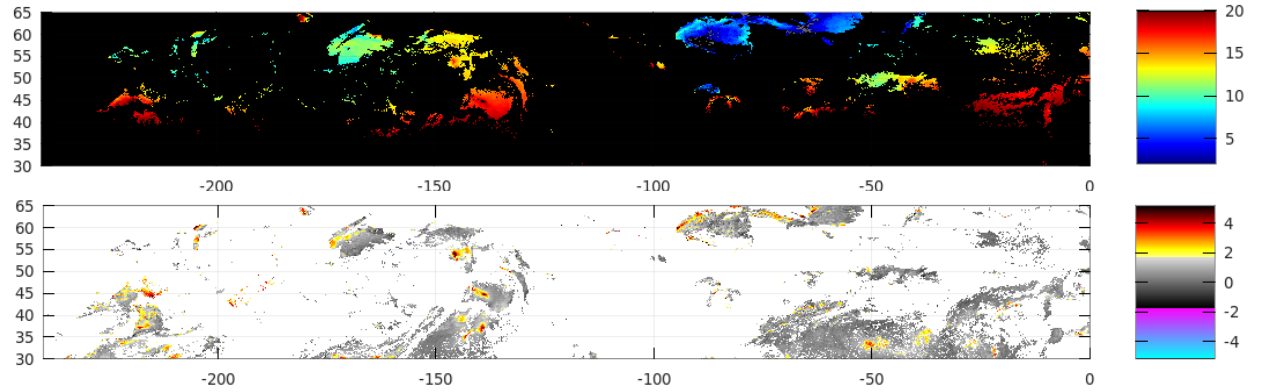
Figure 9: (Top) S-NPP/VIRS SST retrievals on 14 July 2014 from 30°N to 65°N and 120°E to 0°W. Areas identified as contaminated are blacked out. (Bottom) Corresponding SST retrieval field minus K10 background field.
