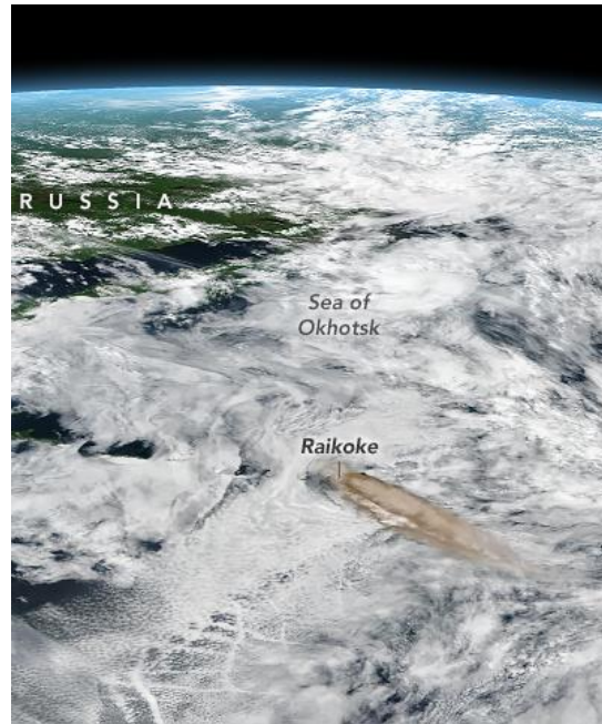
Figure 1: VIIRS composite image from 22 June 2019 over Raikoke. Clouds are seen in white and the volcanic ash cloud can be seen in tan extending from Raikoke.
