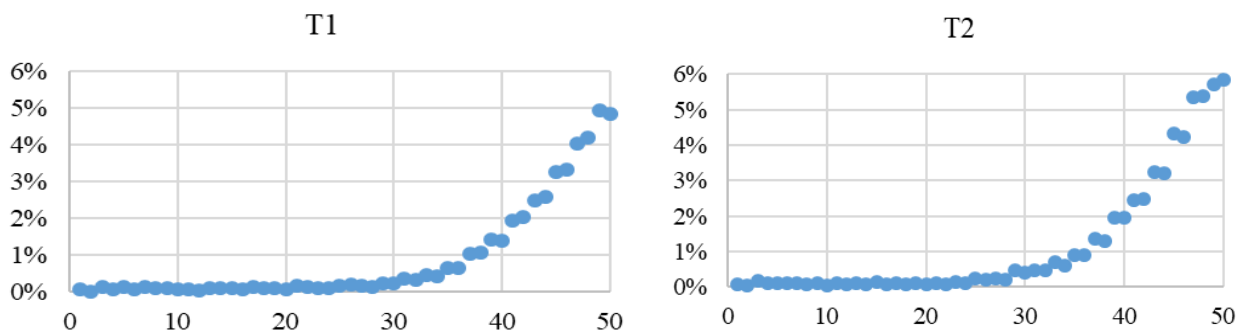
Figure 4. Response Omissions
