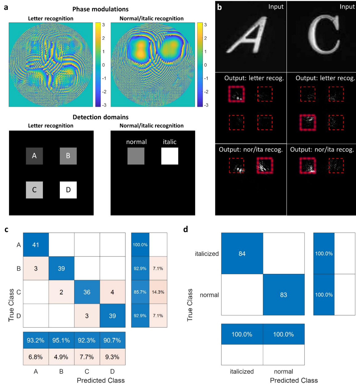
Figure 3.4 Recognition of the identity and typographic styles of 4 letters using a polarization-multiplexing smart glass. (a) Trained phase modulations at two orthogonal incident polarizations on the metasurface and arrangement of detection domains on the output layer. (b) Two examples showing the recognition of an italicized ‘A’ and a normal ‘C’. Upper panels: Input images. Lower panels: Intensity distributions on the output plane showing that the detection domains corresponding to the identity and typographic style of a letter have the highest integrated optical intensity. (c) and (d) Confusion matrices summarizing the results of recognizing 168 letters.
