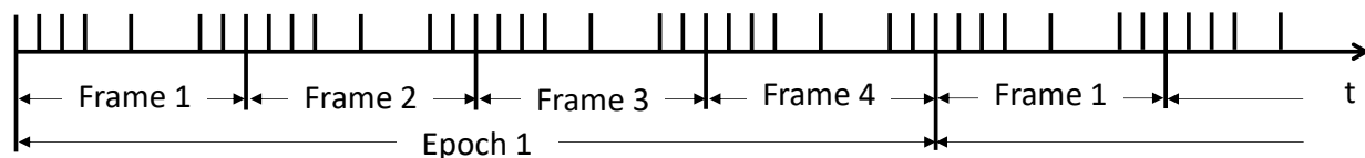
Figure 2-5. Example of Three Levels of Transmission Opportunities
