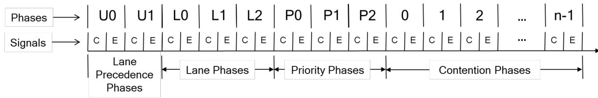
Figure 4-1. CRS Using Four Sets of Phases for Lane Precedence, Lane Selection, Use Precedence, and Contention Resolution
