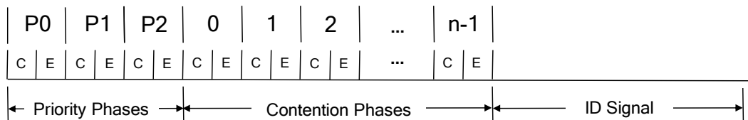
Figure 4-13. Using a Modulated Signal to Provide an ID
