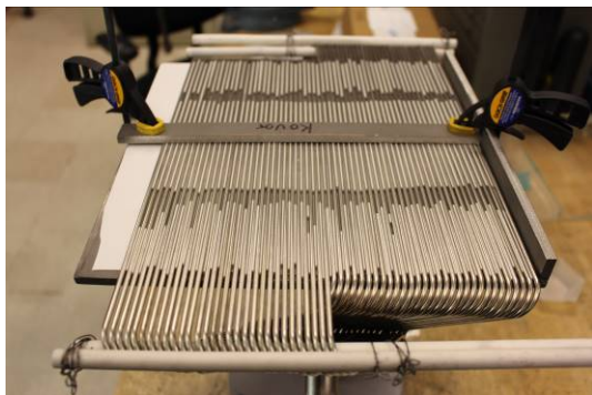
Figure 9. The Gas Tubing Array is clamped down to a Kovar setting plate with 0.020 inch thick Alumina strips separating tubes, and 0.020 inch thick Alumina plates between the Inconel tubes and the Kovar setting plate, also Alumina rods tied together with Molybdenum wire help align tube ends.
