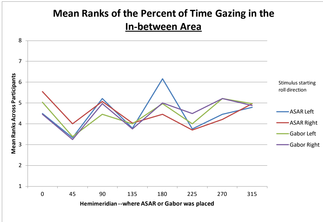
Figure 44. Mean ranks of the percent of time gazing in the in-between area. For the in-between gaze area, mean ranks are plotted across hemimeridian and data are shown separately for the four different contexts.
