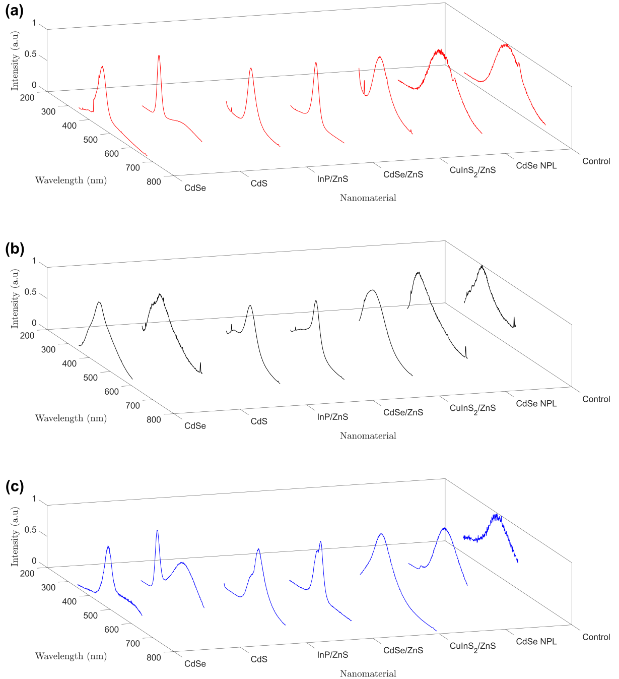
Figure 4. PL spectra of: CdSe, CdS, InP/ZnS, CdSe/ZnS, CuInS 2 /ZnS, CdSe NPL, and control applied: (a) as a thin-film, (b) into a 3D printed structure, (c) into a polymer structure.
