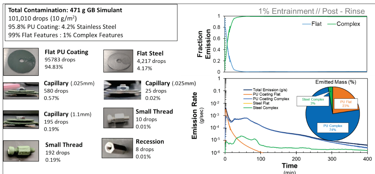
Figure 50. Predicted post-rinse vapor emission from a vehicle with 1% entrainment in capillary features.
