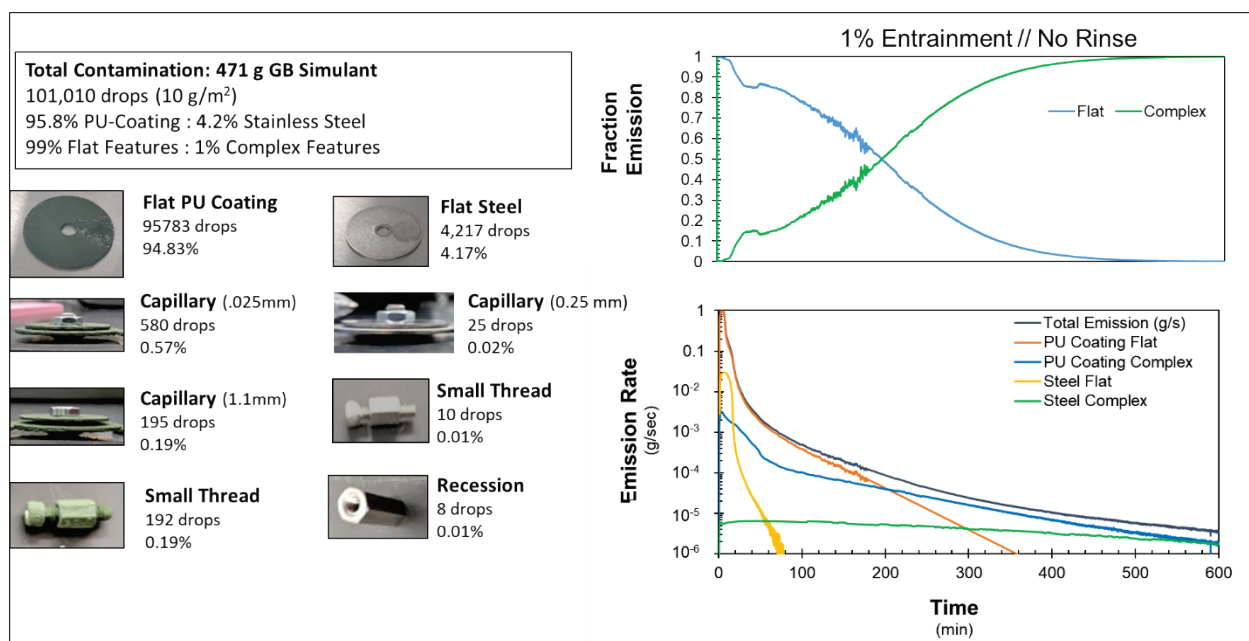
Figure 46. Predicted vehicle emission profile with 1% entrainment in capillary features (no rinse).
