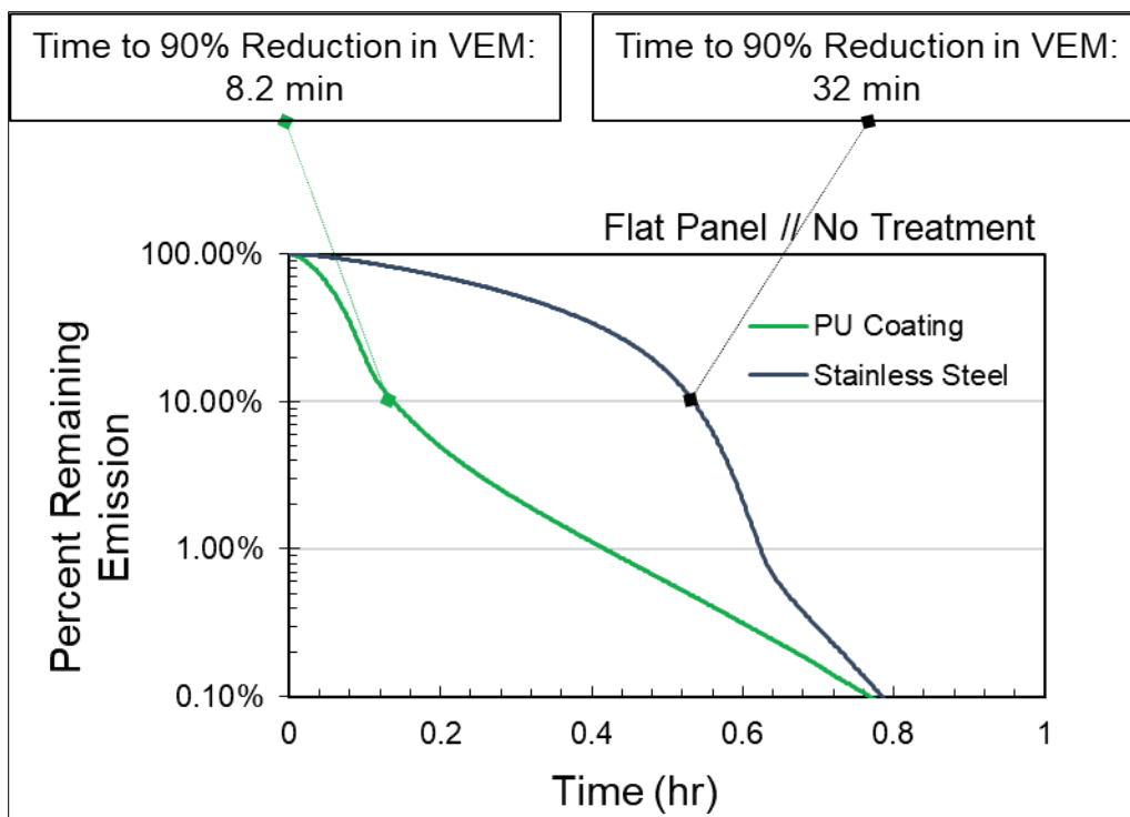
Figure 18. Percent remaining emission vs time for untreated bare stainless steel (gray) and coated surfaces (green).
