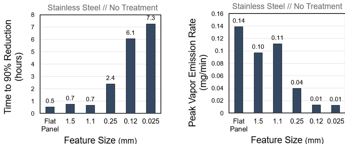
Figure 20. Vapor duration and peak emission rate for stainless steel capillaries.
