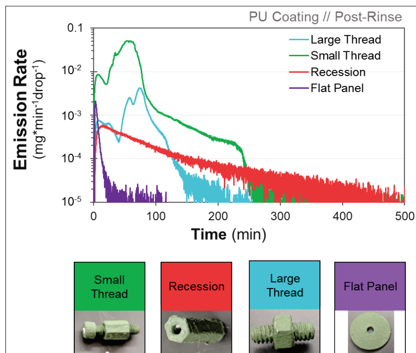
Figure 37. Influence of feature geometry on post-rinse vapor emission from PU-based coatings.
