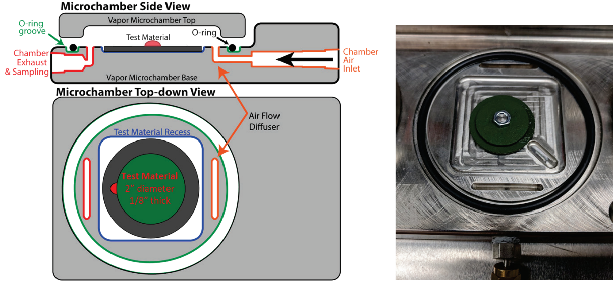
Figure 9. Schematic and photograph of a vapor microchamber used to contain the test materials.
