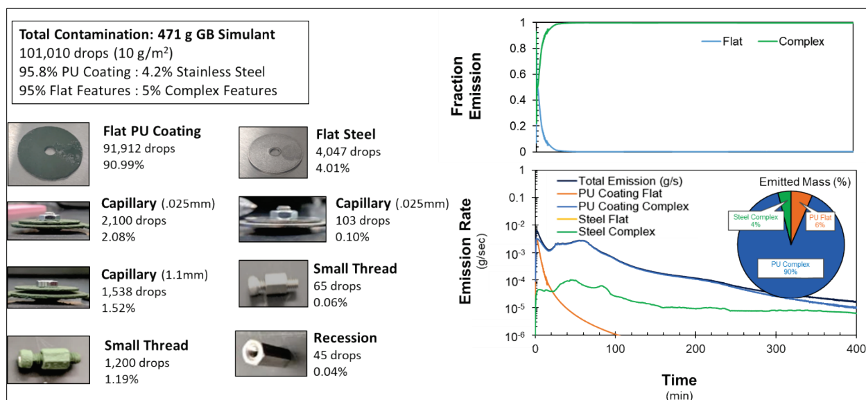
Figure 51. Predicted post-rinse vapor emission from a vehicle with 5% entrainment in capillary features.
