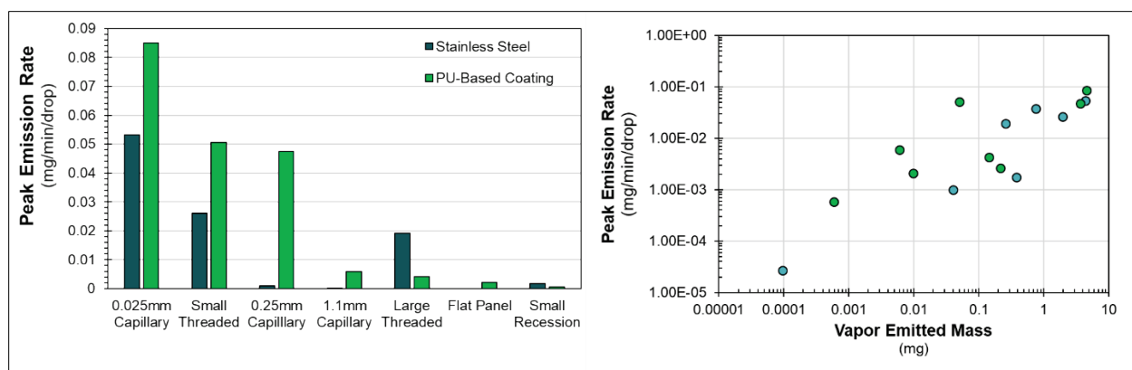
Figure 42. Peak emission rate for rinsed complex features (left) and comparison of post-rinse VEM with post-rinse peak vapor emission rate (right).
