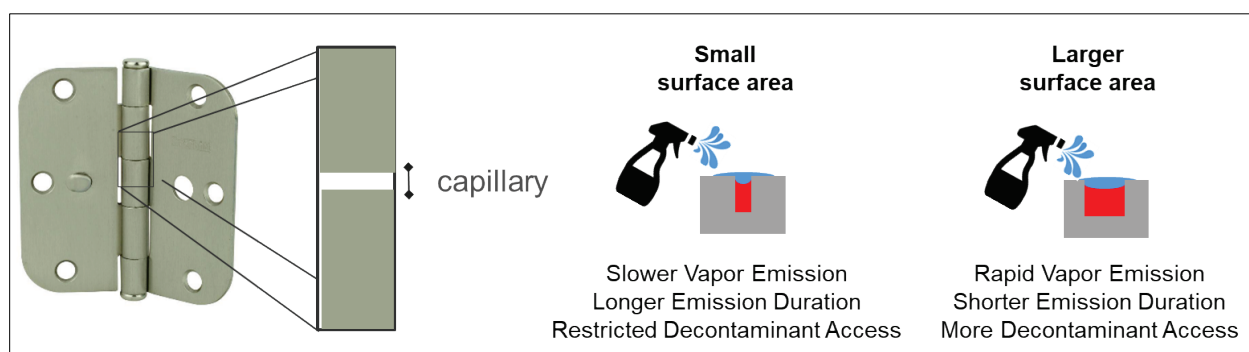
Figure 2. Capillary action explains how complex features influence contaminant retention and the resulting contaminant distribution in and on the material, decontaminant performance, and vapor emission.
