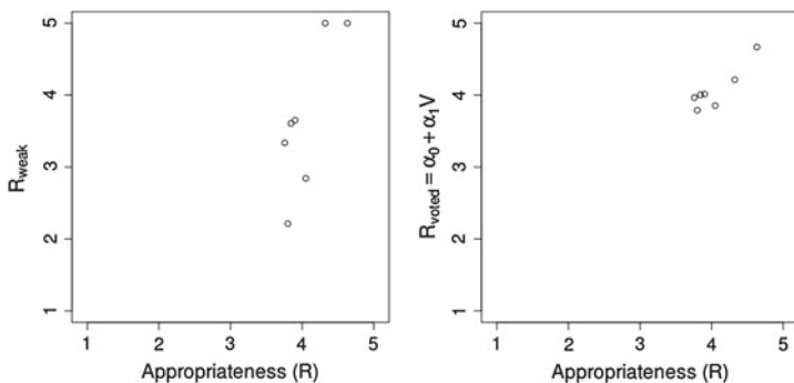
Fig. 4 Comparison between two automatic evaluation understudy measures at system level in static context setting
