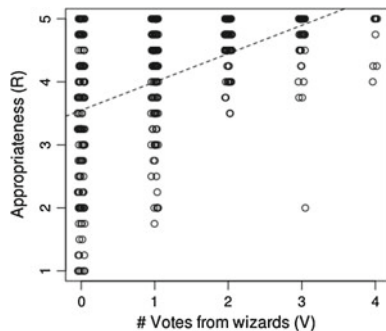
Fig. 3 Appropriateness of responses ( R ) as judges by 4 human judges plotted against the number of wizard votes ( V ) received by those responses. The dashed line indicates a fitted linear model. A small amount of jitter is added to V for visualization
