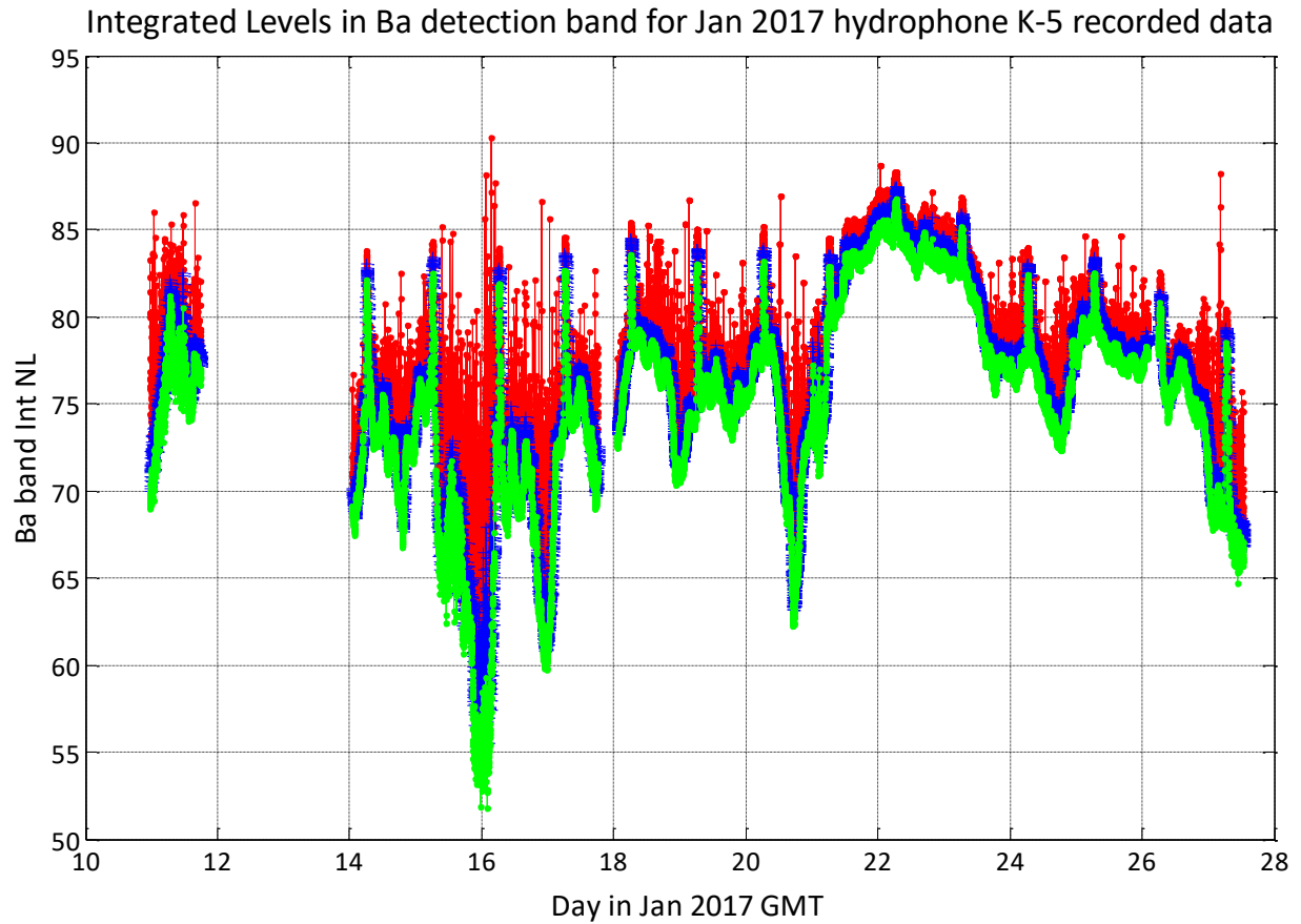
Figure 25. Minke whale boing detection band (1320 Hz to 1440 Hz) integrated spectral levels 90 th (red), 50 th (blue), and 10 th (green) percentiles for hydrophone K-5 from January 11-27, 2017.
