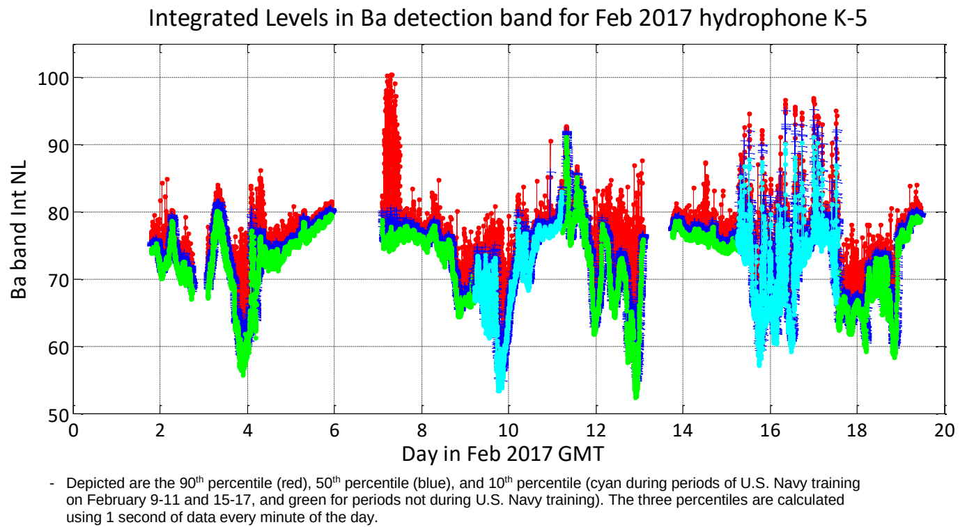
Figure 27. February 2017 integrated spectral levels over the minke whale boing detection band for available recorded data.
