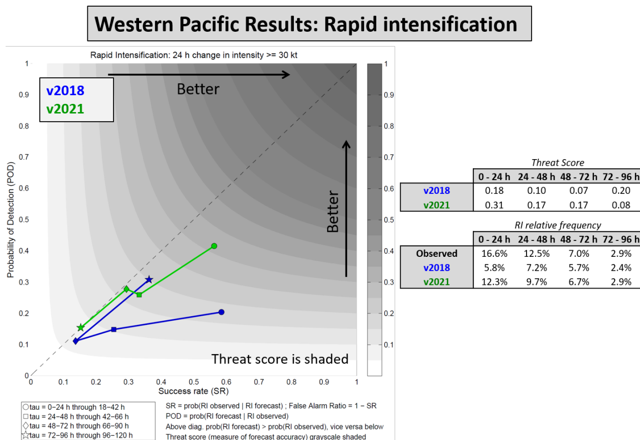
Fig. 10—RI statistics for the unperturbed control member, comparing v2018 (blue) to v2021 (green) at various lead times, for the West Pacific. The x-axis indicates success rate (SR), the y-axis indicates probability of detection (POD), and the threat score is shaded. Tables indicating the threat score and the RI relative frequency are also included.
