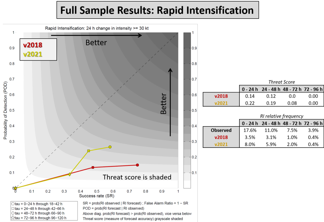
Fig. 13—RI statistics for the mean of the full 11-member ensemble, comparing v2018 (red) to v2021 (yellow) at various lead times for all basins. The x-axis indicates success rate (SR), the y-axis indicates probability of detection (POD), and the threat score is shaded. Tables indicating the threat score and the RI relative frequency are also included.
