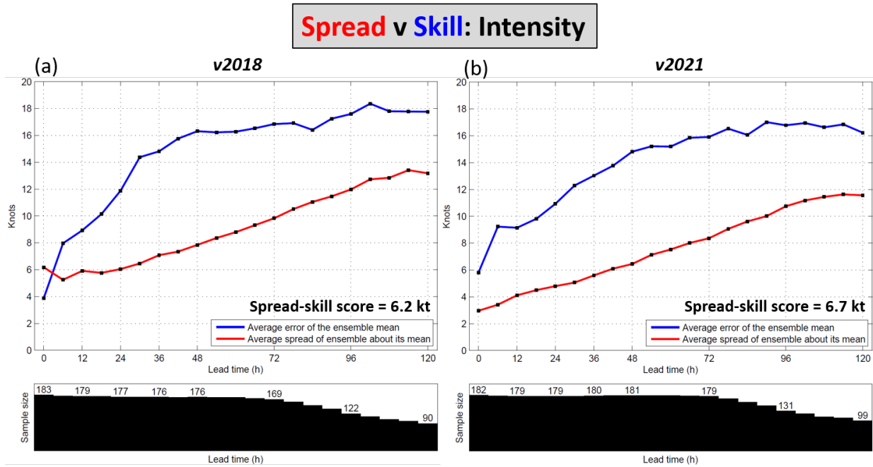
Fig. 15—Spread-skill score, which is a sample-size weighted, lead-time averaged absolute difference between spread and skill, for intensity (low score = good) for (a) v2018 and (b) v2021. The average error of the ensemble mean (blue) and the average spread of the ensemble about its mean (red) are shown. The number of cases in the sample at each forecast lead time are indicated below each panel.
