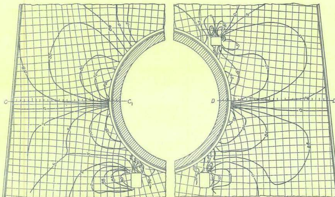
ISOCLINICS AND FORCE LINE FLOW MAP BARBETTE-COMplete ATTACHMENT.
