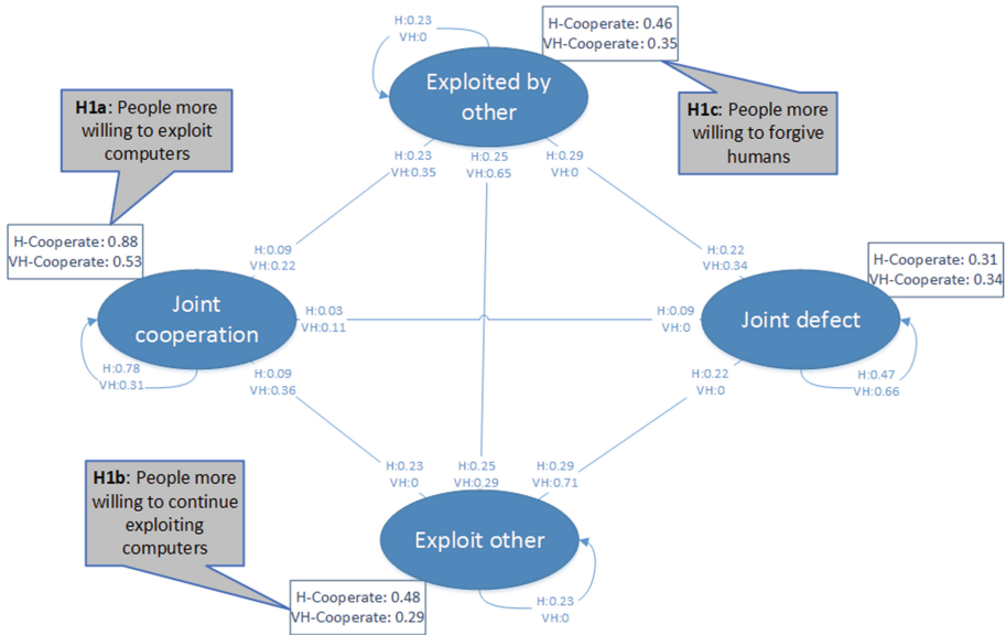
Fig. 3. Markov chain of the possible game states. Boxes display the chance a participant would choose to cooperate given in a certain state and support H1.
