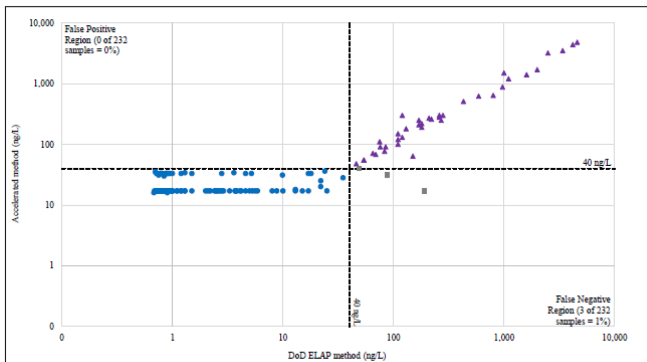
Figure 7-4. Secondary PFAS Compounds – Reliability Plots
