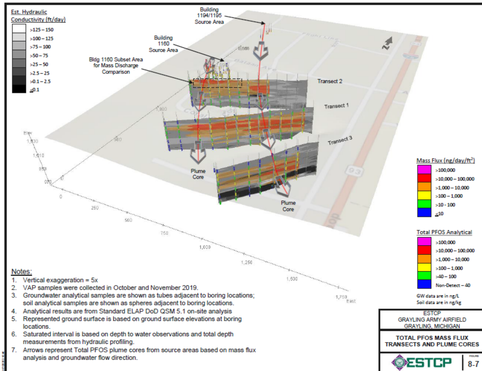
Figure 8-7. Total PFOS Mass Flux Transect and Plume Cores
