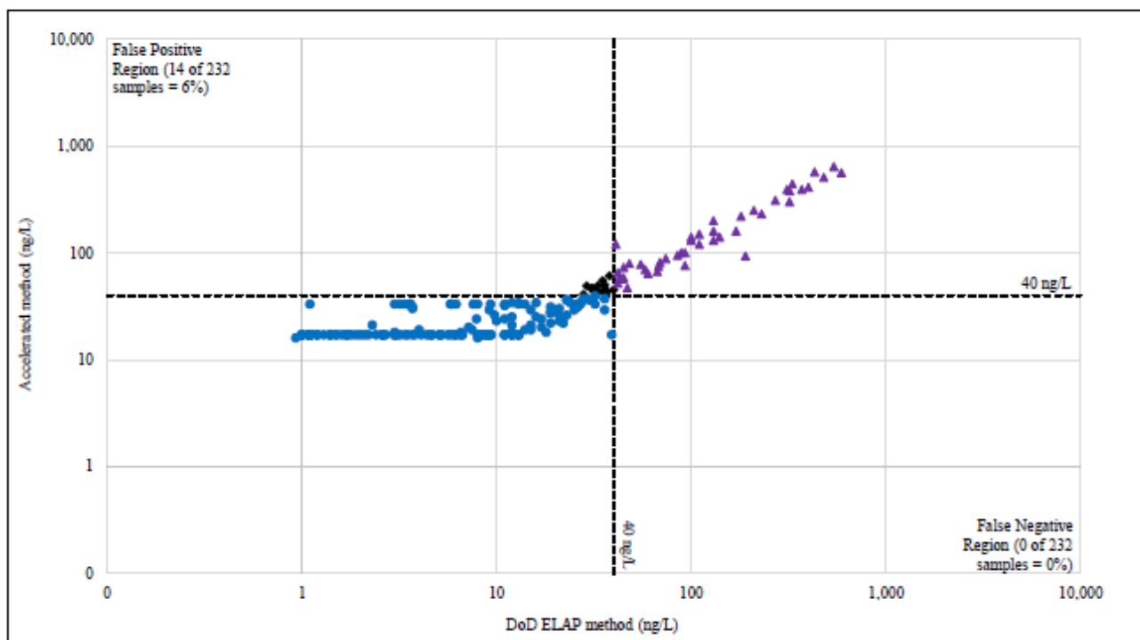
Figure 7-3. Primary PFAS Compounds –Reliability Plots
