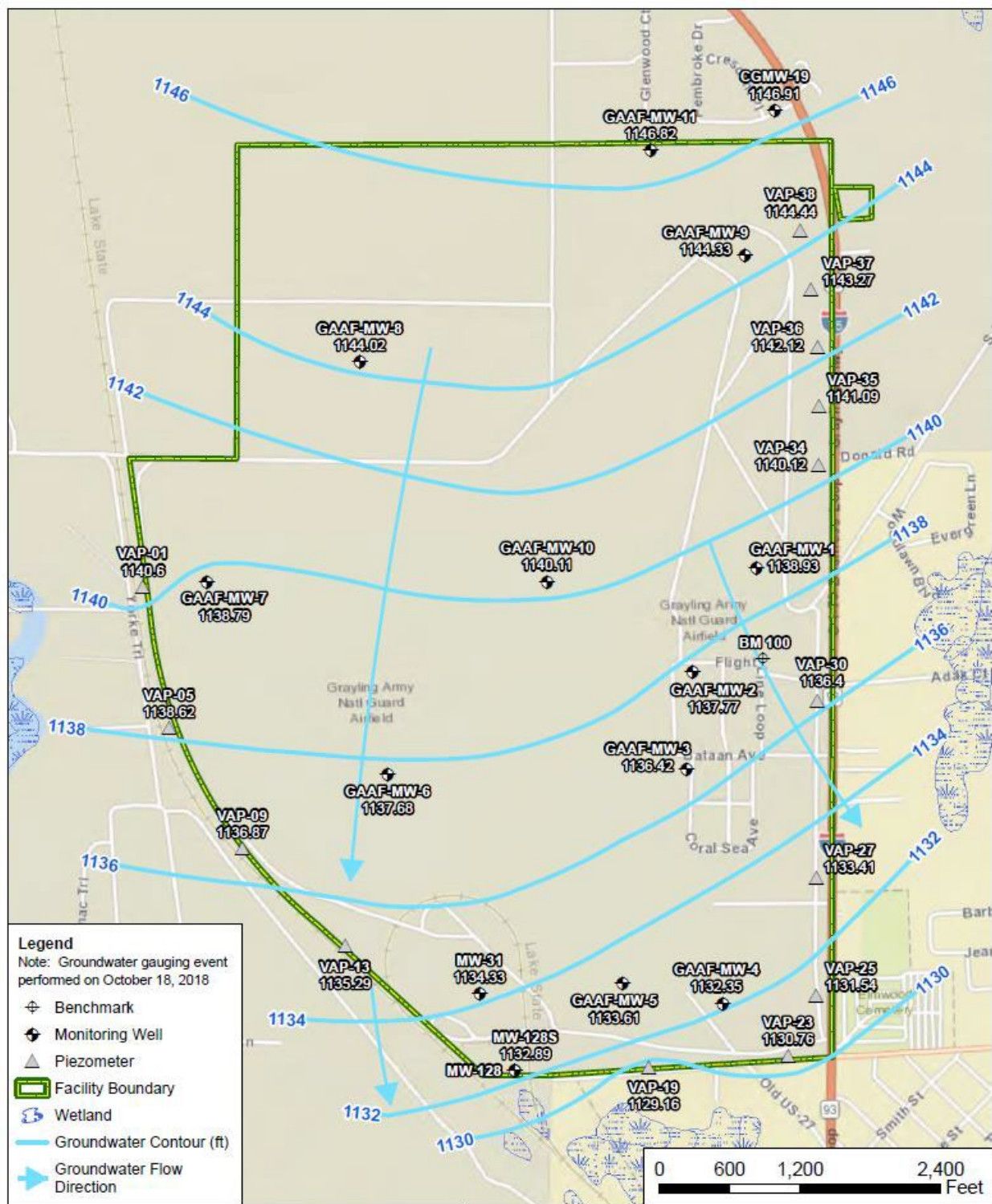
Figure 4-1. GAAF Groundwater Elevation Contour Map
