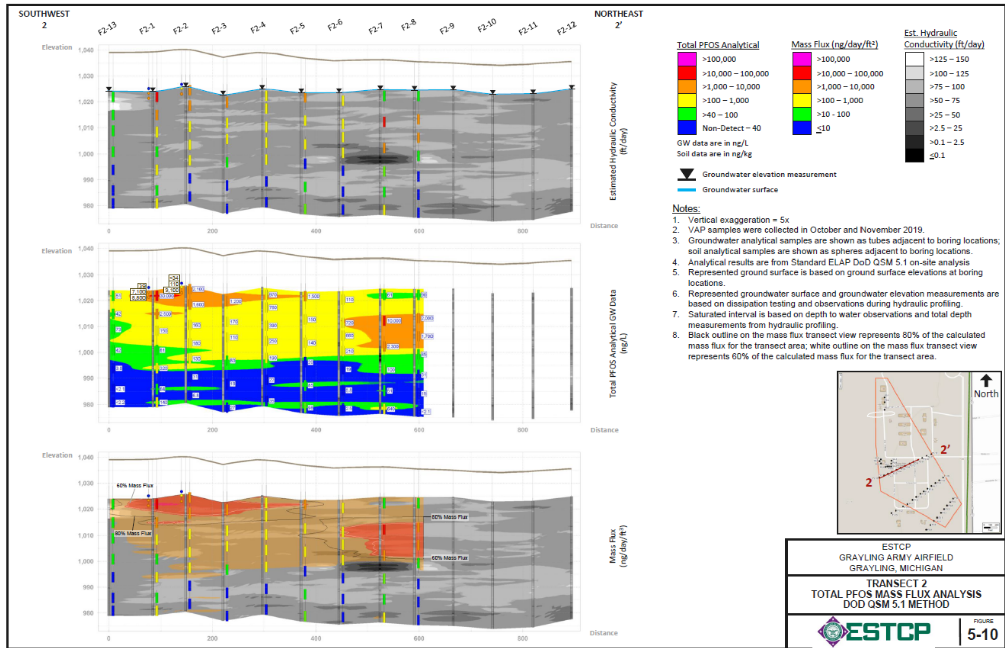
Figure 5-10. Transect 2 Total PFOS Mass Flux Analysis DoD QSM 5.1 Method
