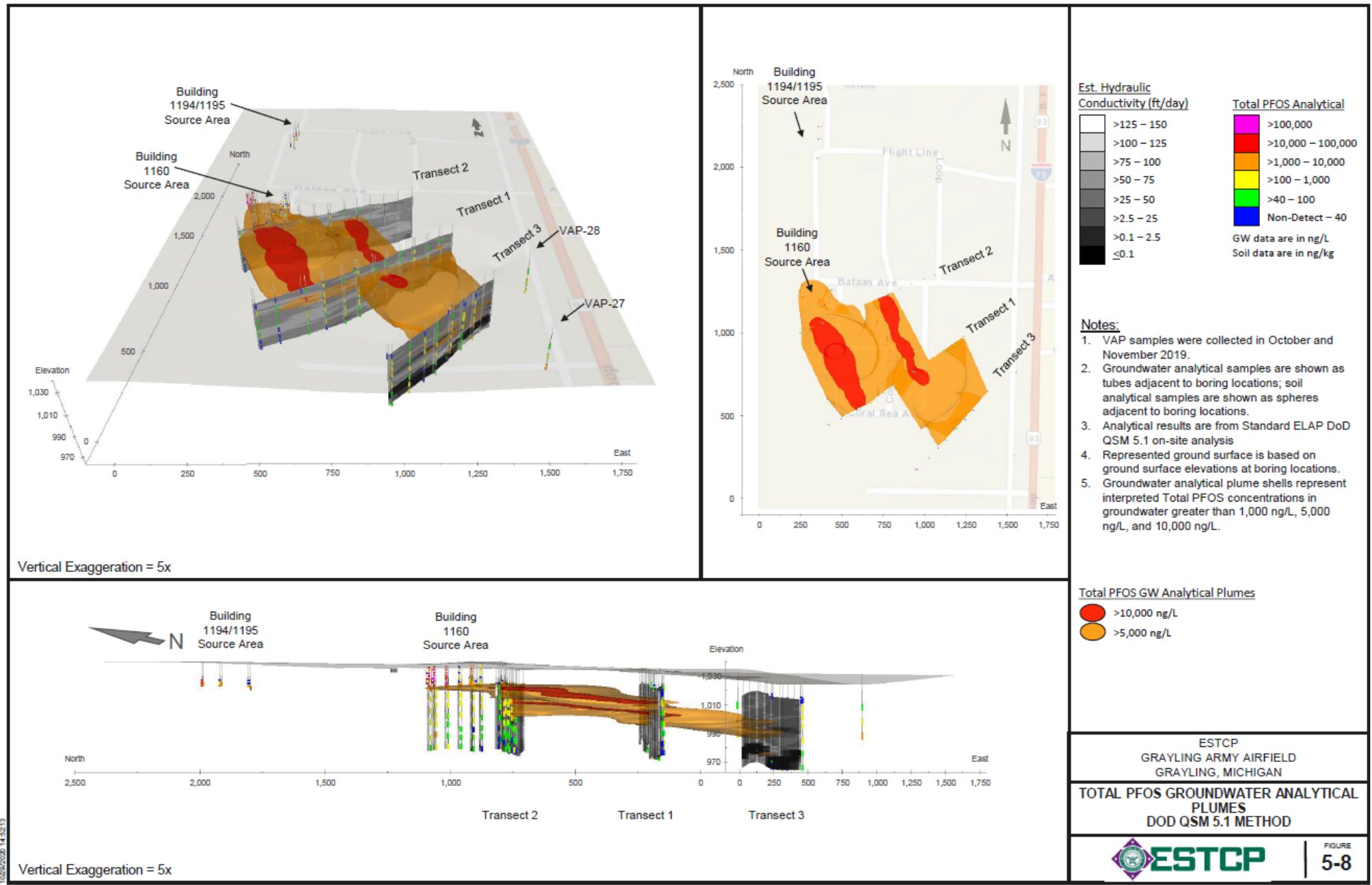
Figure 5-8. Total, PFOS Groundwater Analytical Plumes DoD QSM 5.1 Method
