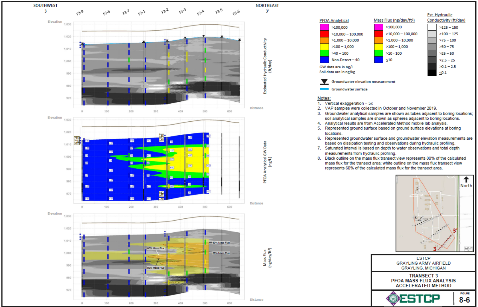
Figure 8-6. Transect 3 PFOA Mass Flux Analysis Accelerated Method
