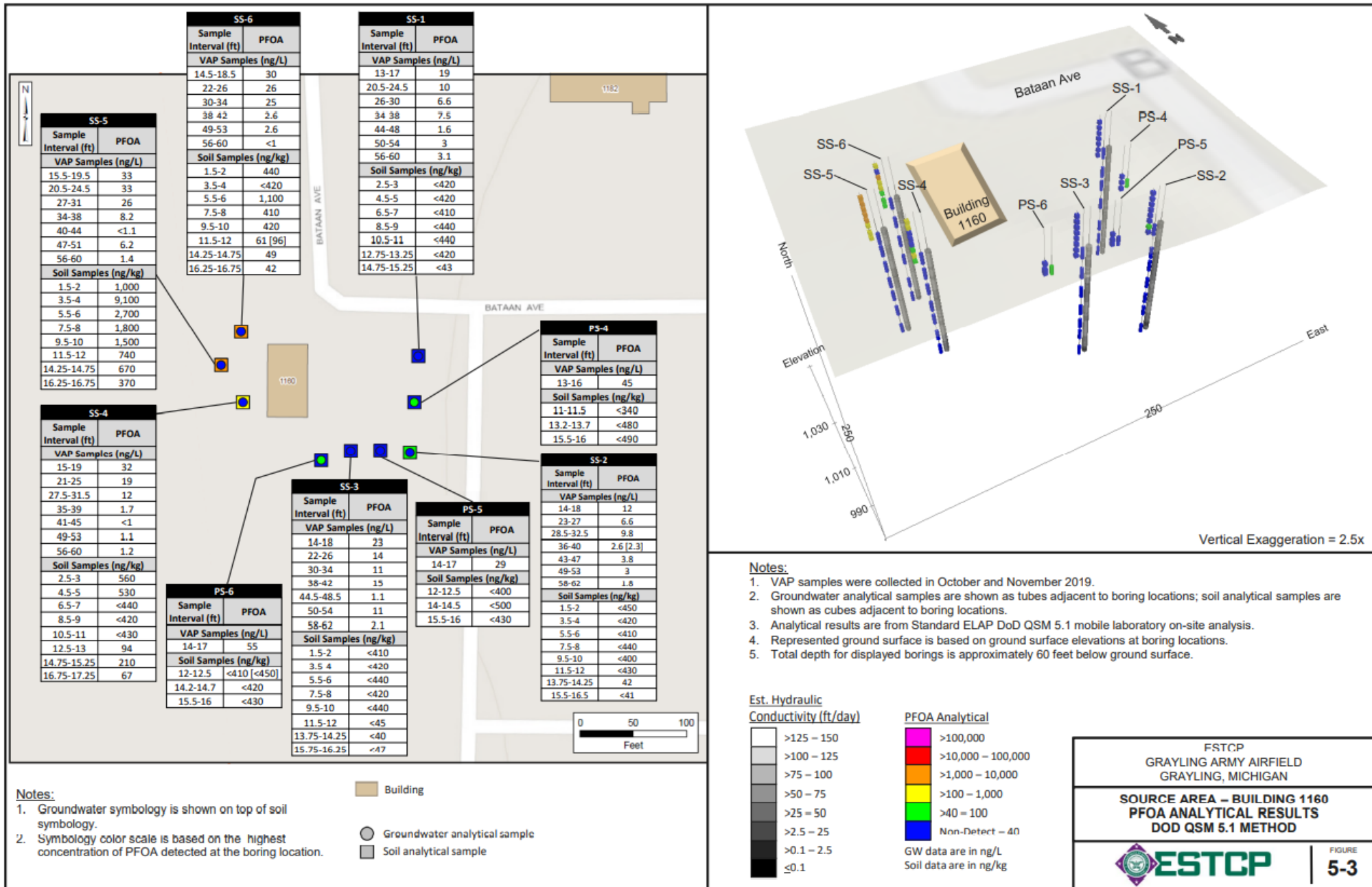
Figure 5-3. Source Area – Building 1160 PFOA Analytical Results DoD QSM 5.1 Method
