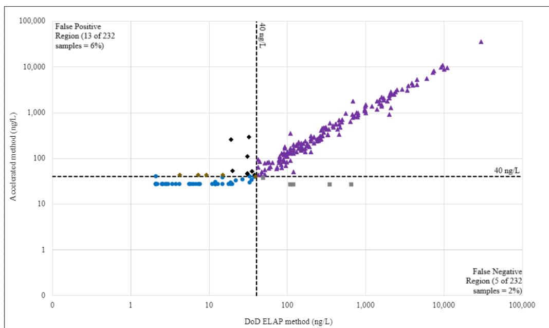
Figure ES-2. Total PFOS Reliability Based on Action/No Action at 40 ng/L
