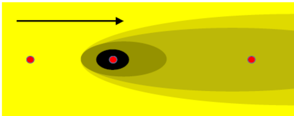
Distribution of sulfate at a site where the extent of sulfate depletion is greatest at the source.
