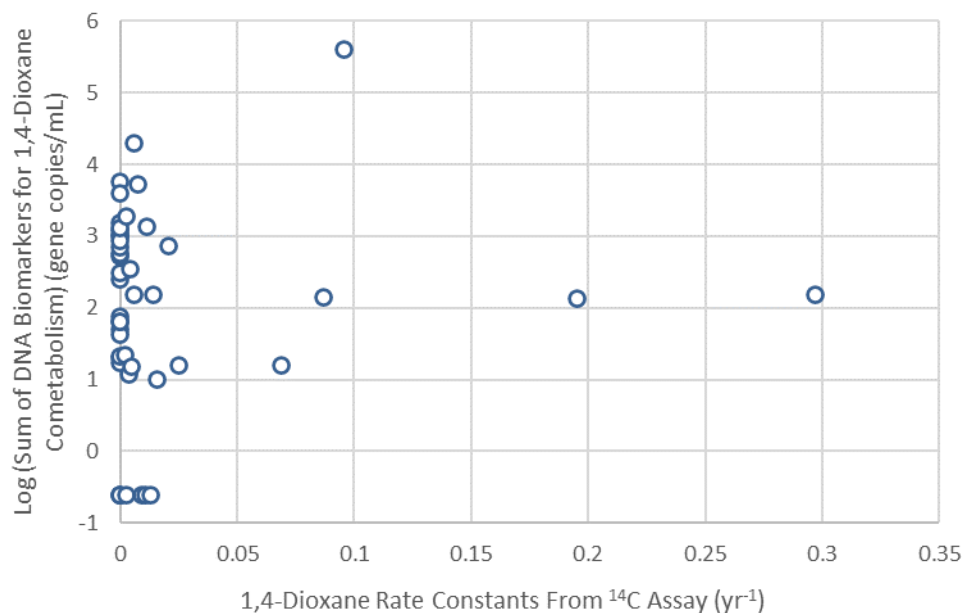
Figure 5.8.7. Comparison of DNA Biomarkers for 1,4-Dioxane Cometabolism and 1,4-Dioxane Rate Constants Obtained Using ^{14}\text{C} Assay. No clear relationship could be established.
