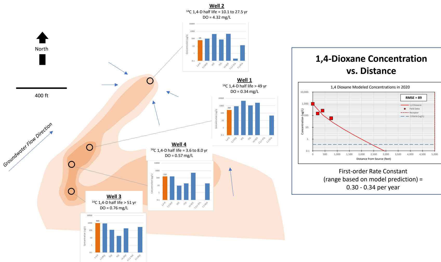
Figure 5.7.10.1. Site 10 (DoD) Summary of 1,4-Dioxane/CVOC Concentration Trends and Rate Constants.
