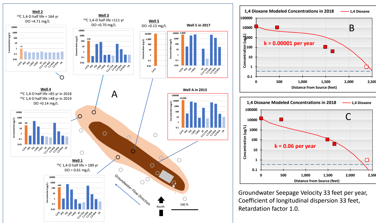
Figure 5.7.5.2. Site 5 (DoD) Summary of 1,4-Dioxane/CVOC Concentrations and Attenuation of 1,4-Dioxane with Distance from the Source. Pale values in Panel A and open symbols in other panels are plotted at the reporting limit.
