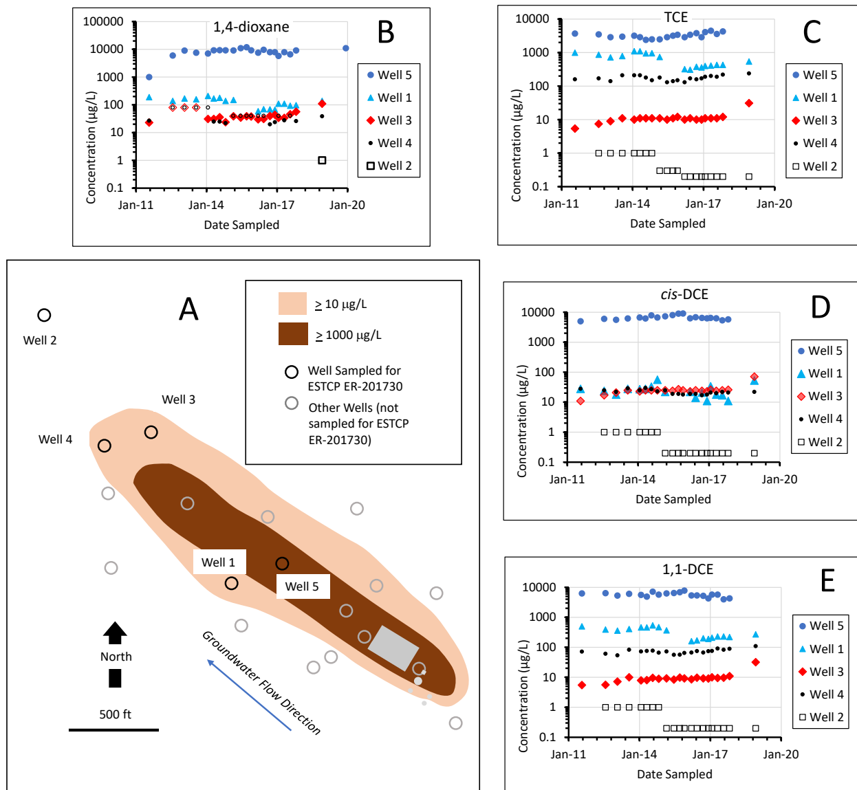
Figure 5.7.5.1. Site 5 (DoD) Changes in Concentrations of 1,4-Dioxane and CVOCs over time.
