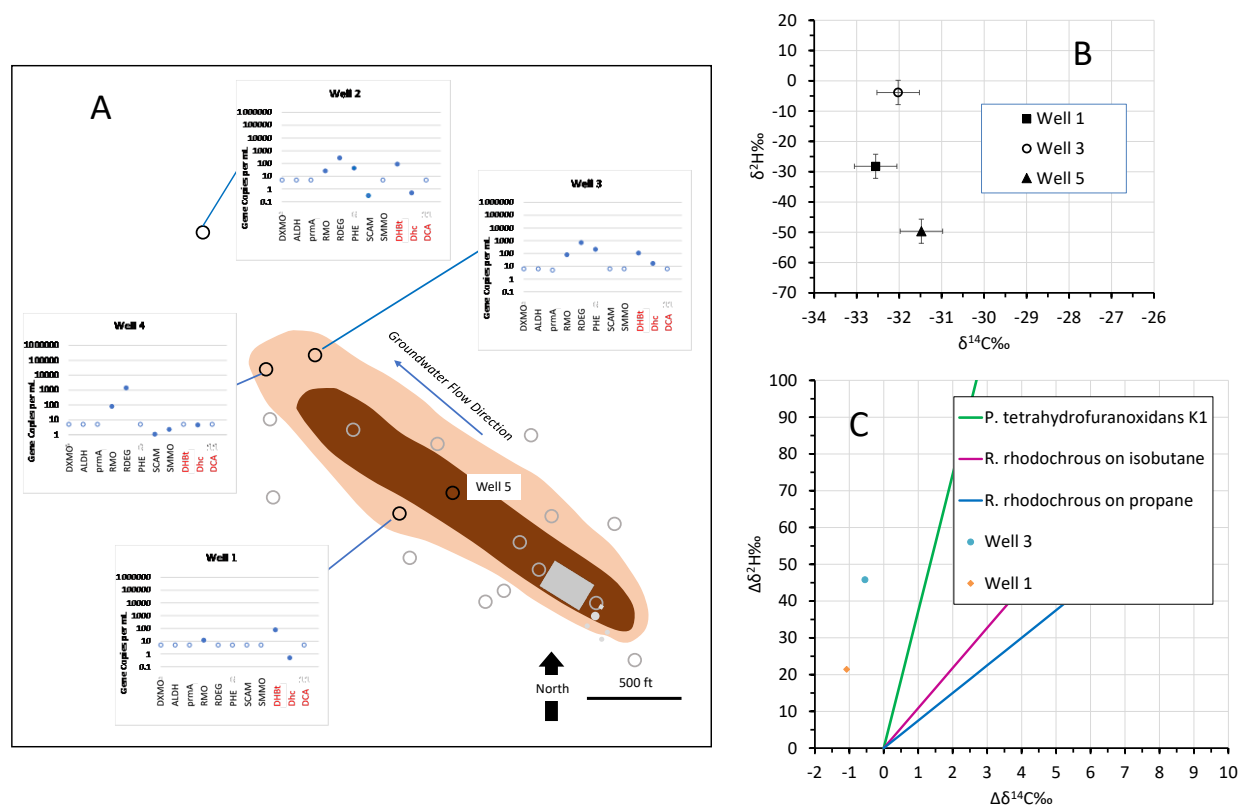
Figure 5.7.5.3. Site 5 (DoD) Summary of Biomarker Data and Isotope Data for 1,4-Dioxane. Open circles in abundance of qPCR biomarkers in Panel A indicate the limit of quantitation. Error bars in Panel B are one standard deviation.
