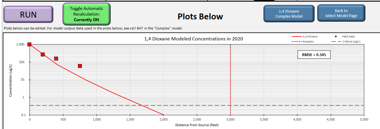
Figure 12. Example Simulation where Initial Estimate from Box 6c Used as Starting Point for 1,4-Dioxane Biodegradation (Rate Constant = 0.514 per year). Visual inspection of concentration vs. distance plot confirms that degradation is overestimated, such that model needs further calibrating.
