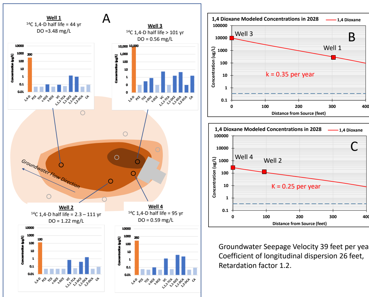
Figure 5.7.4.2. Site 4 (Industrial) Summary of 1,4-Dioxane/CVOC Concentrations and Attenuation of 1,4-Dioxane with Distance from the Source.
