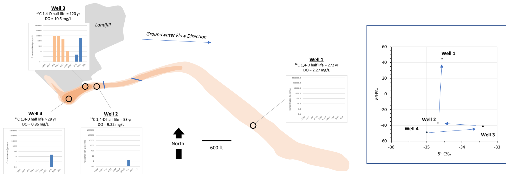
Figure 5.7.9.2. Site 9 (DoD) Summary of Biomarker and Isotope Data.
