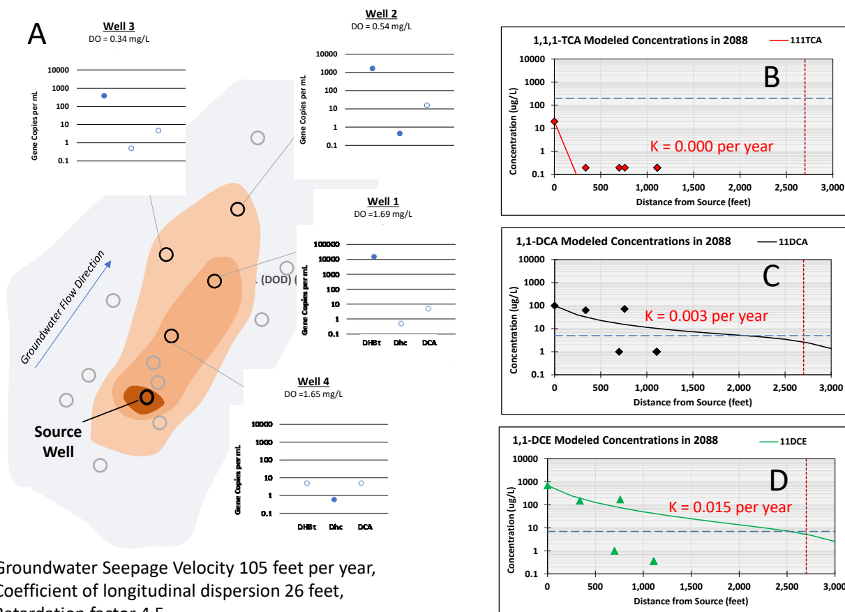
Figure 5.7.1.4. Site 1 (DoD) Summary of Biomarkers for CVOCs and Concentration Trends and Rate Constants for 1,1,1-TCA and 1,1-DCA and 1,1-DCE.
