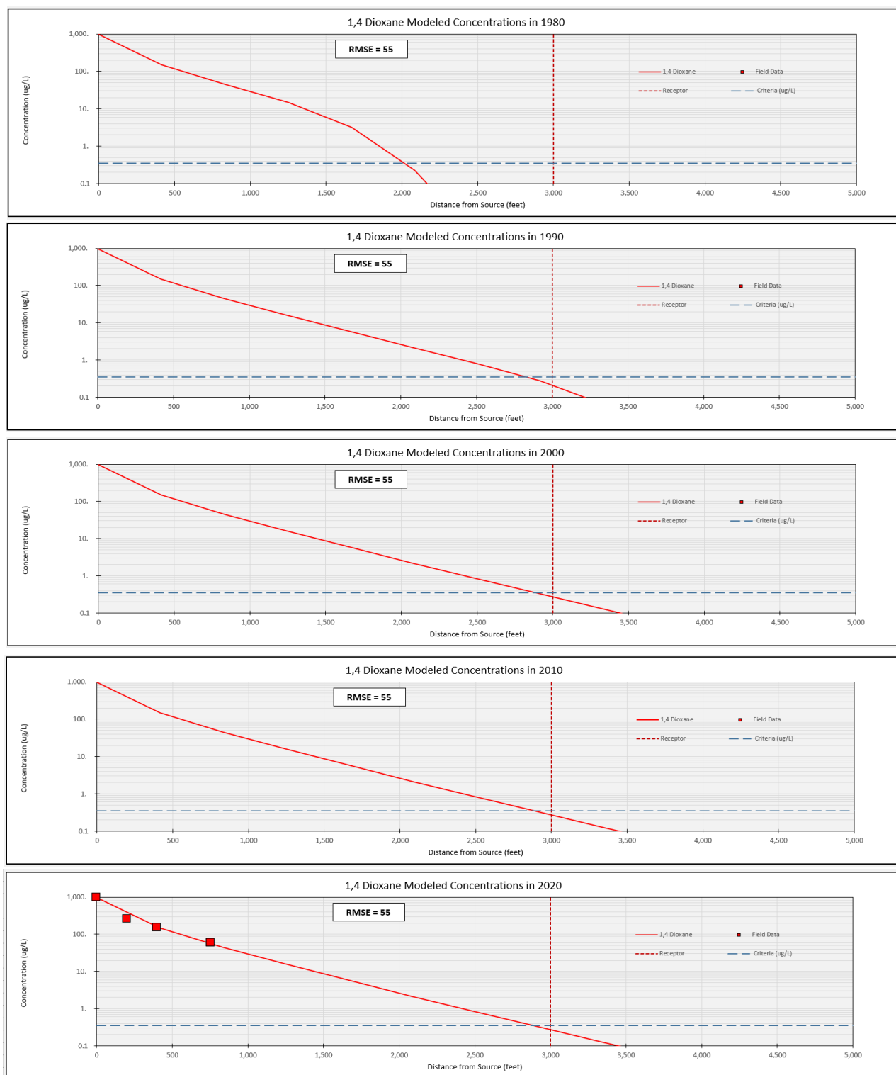
Figure 6.3. Example Simulation Showing 1,4-Dioxane Plume Extent Over Time (Rate Constant = 0.32 per year).
