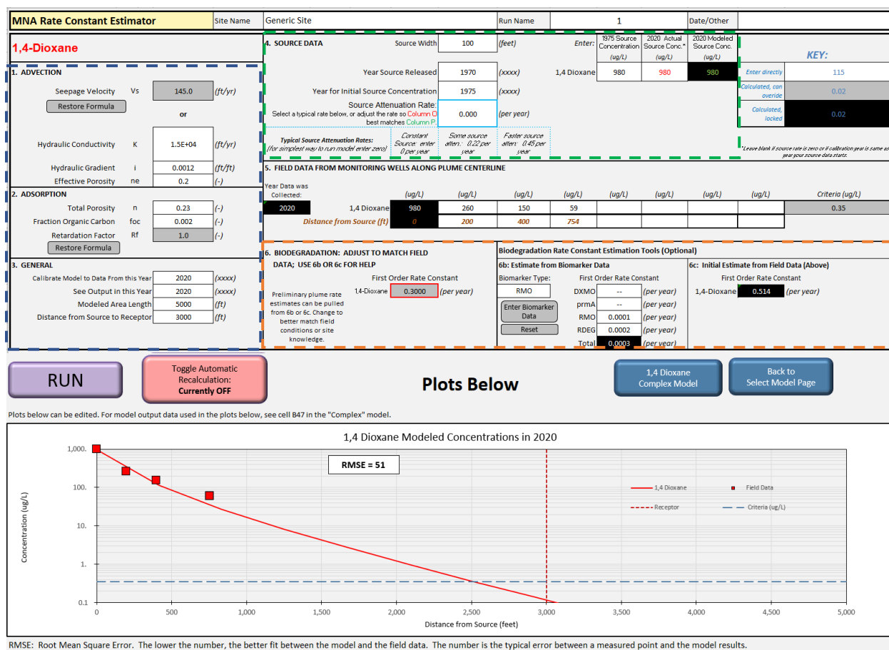
Figure 6.1. Interface for the Simple 1,4-Dioxane Model in the “MNA Rate Constant Estimator”.
