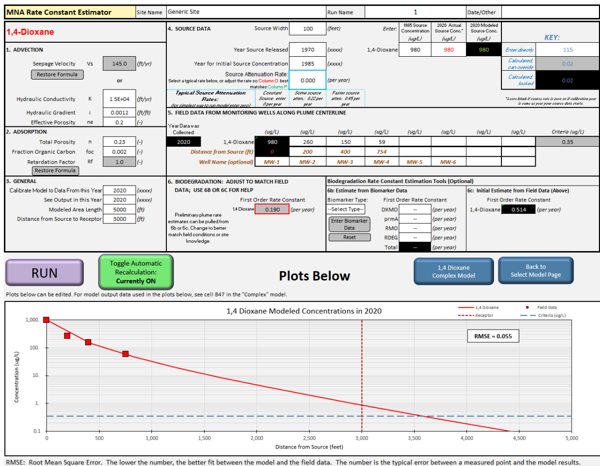
Figure 11. Example Simulation with Evidence of 1,4-Dioxane Biodegradation Based on Model Calibration (Rate Constant = 0.19 per year). Visual inspection of concentration vs. distance plot and low RMSE value confirms that model is calibrated.
