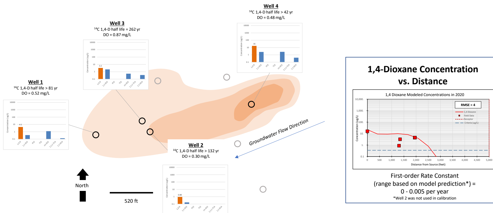
Figure 5.7.6.1. Site 6 (DoD) Summary of 1,4-Dioxane/CVOC Concentration Trends and Rate Constants.
