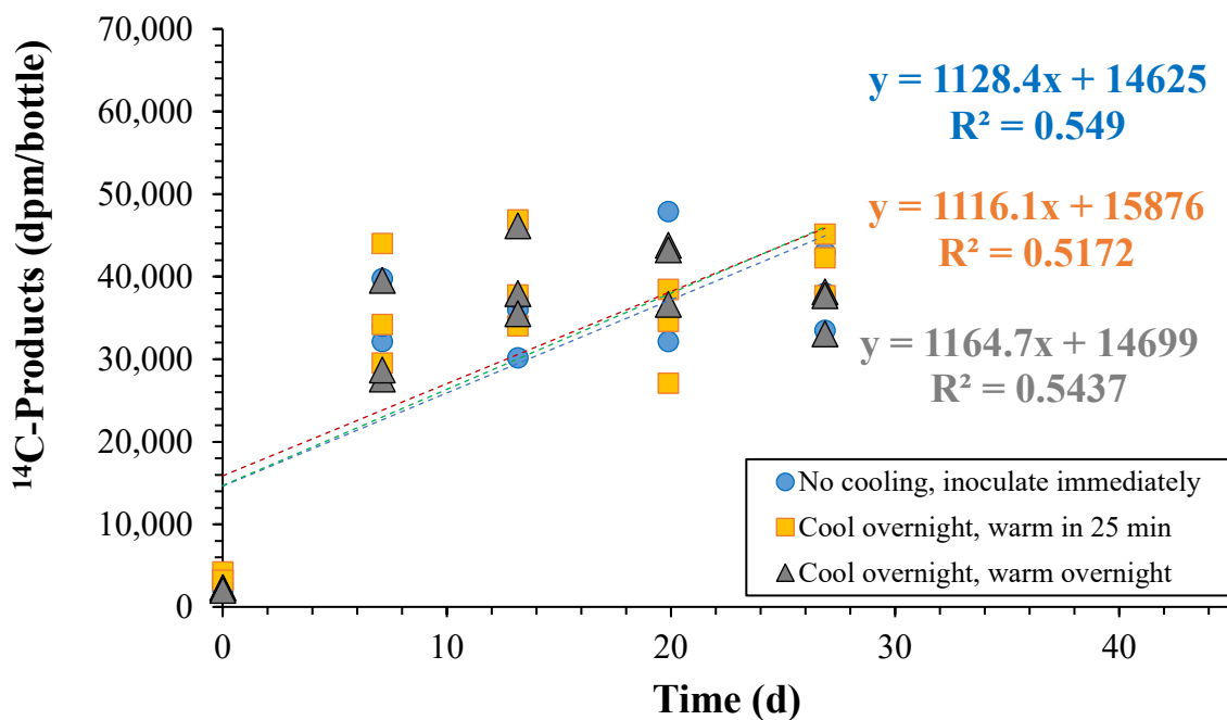
Figure 5.6.13. Effect of sample handling on biodegradation of 1,4-dioxane by the ENV487 culture at an initial concentration of 163 \mu\text{g/L} in groundwater (Site 6, Well 3).
