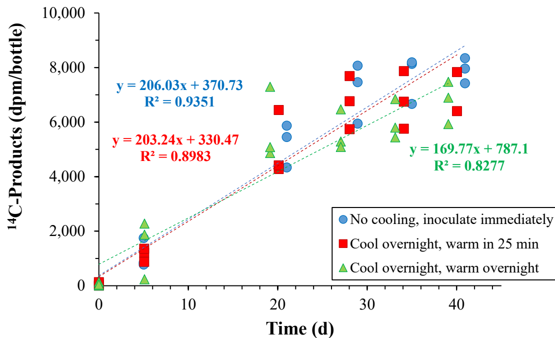
Figure 5.6.11. Effect of sample handling on biodegradation of 1,4-dioxane by the CB1190 culture at an initial concentration of 163 \mu\text{g/L} in groundwater (Site 6, Well 2).
