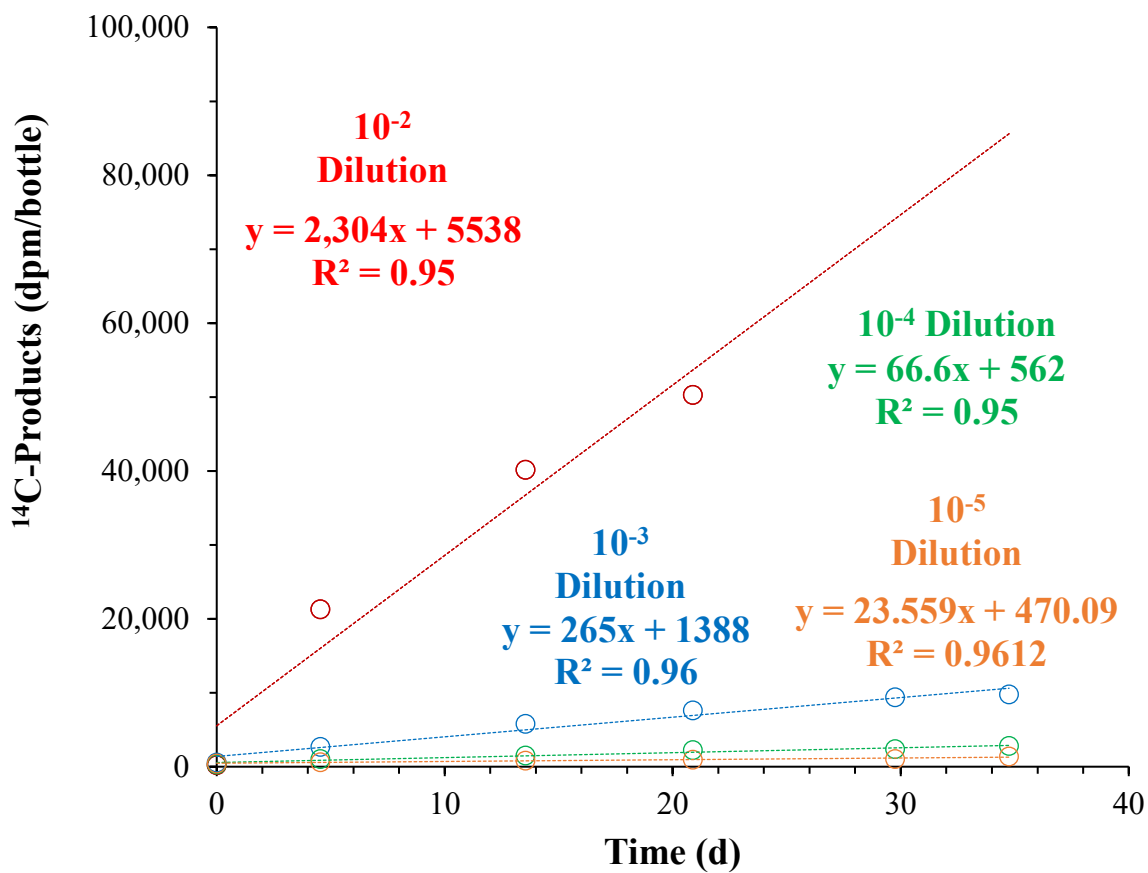
Figure 5.6.6. Evaluation of the ^{14}\text{C} assay using the ENV487 culture grown on propane at varying dilution levels. Cells were suspended in BSM.
