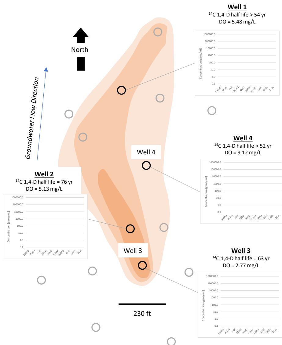
Figure 5.7.8.2. Site 8 (DoD) Summary of Biomarker and Isotope Data. All qPCR biomarkers were below limits of quantitation.
