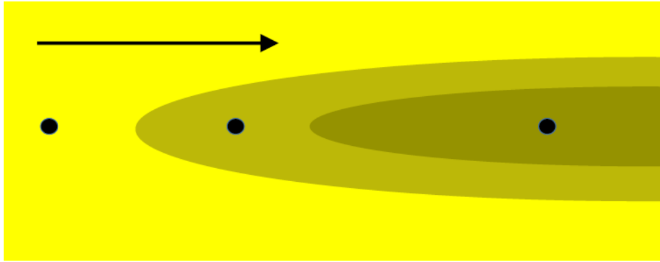
Distribution of sulfate at a site where there is a decrease in sulfate concentration along the flowpath.
