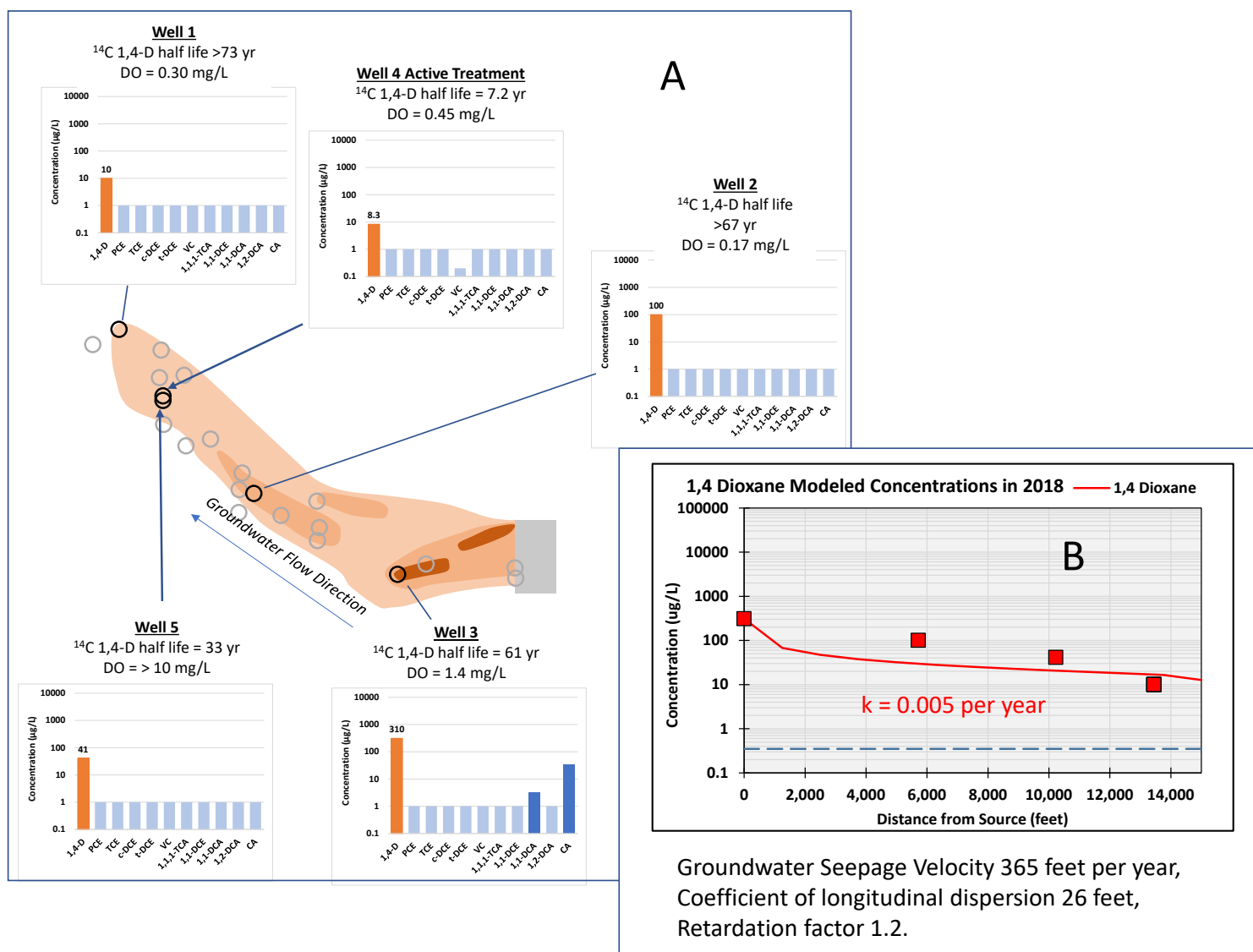
Figure 5.7.3.2. Site 3 (Industrial) Summary of 1,4-Dioxane/CVOC Concentrations and Attenuation of 1,4-Dioxane with Distance from the Source.
