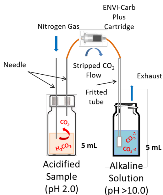
Figure 5.6.2. Schematic of the apparatus used to separate ^{14}\text{CO}_2 .
