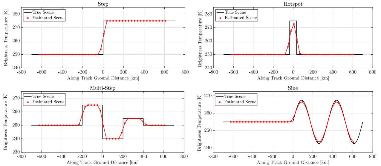
Fig. 4 — Baseline: truth and reconstructed brightness temperature scenes using parameters from Table 1 for (Top Left) step, (Bottom Left) multistep, (Top Right) hotspot, and (Bottom Right) sine.
