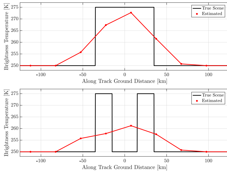
Fig. 6 — (Top) Hotspot and (Bottom) dual-hotspot scenes. All parameters taken from Table 1.
