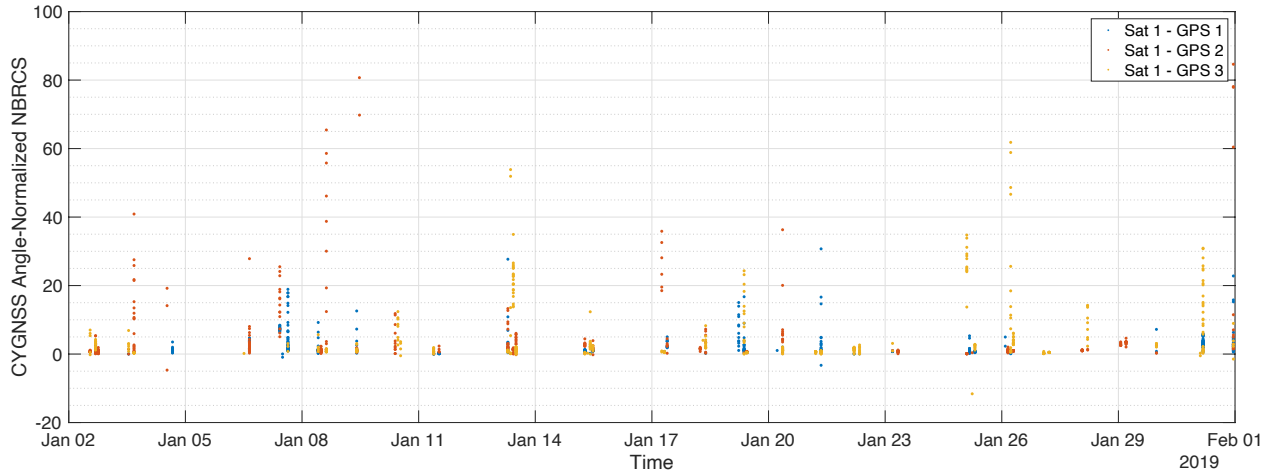
Fig. 8 — CYGNSS satellite 1 incidence angle normalized NBRCS values
