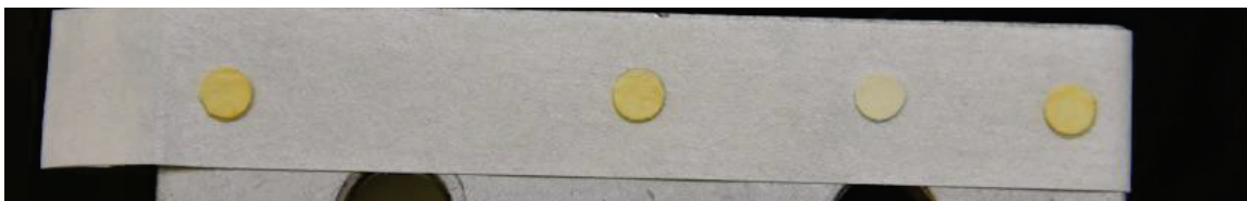
Figure 37. Three VX dots were exposed to VX in the chamber for a total of 100 min. Concentration of chamber was 0.056 \text{ mg/m}^3 at 100 min. Slight color change was observed when an unexposed dot was placed (third from left) for contrast.
