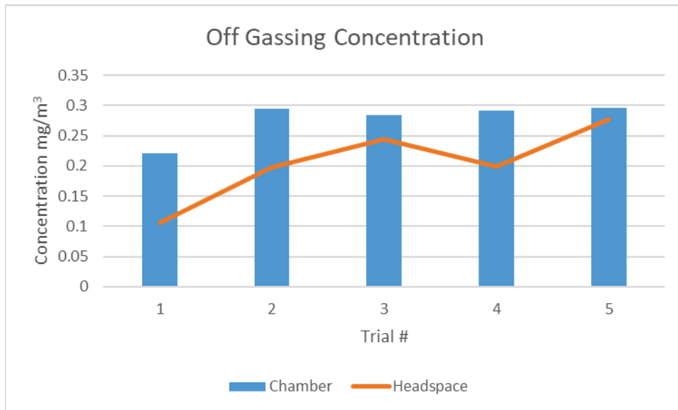
Figure C-1. Off-gassing concentration.
