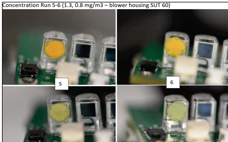
Figure 29. New dots before (top) and after (bottom) HD exposure for concentration runs 5 (no. 9) and 6 (no. 10) in blower housing 60.
