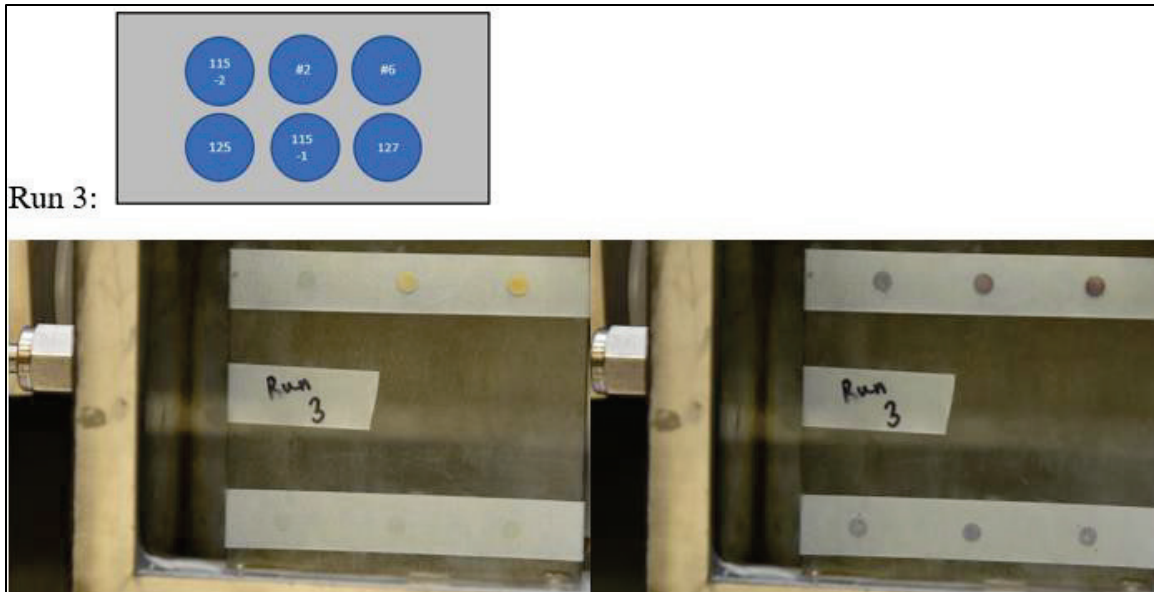
Figure 15. Run 3: (Top) Third of three randomized arrays of six dots. (Bottom) Images of dots in chamber before (left) and after (right) GB exposure. GB exposure was 21.5 \text{ mg/m}^3 for 20 min for six randomly placed dots.
