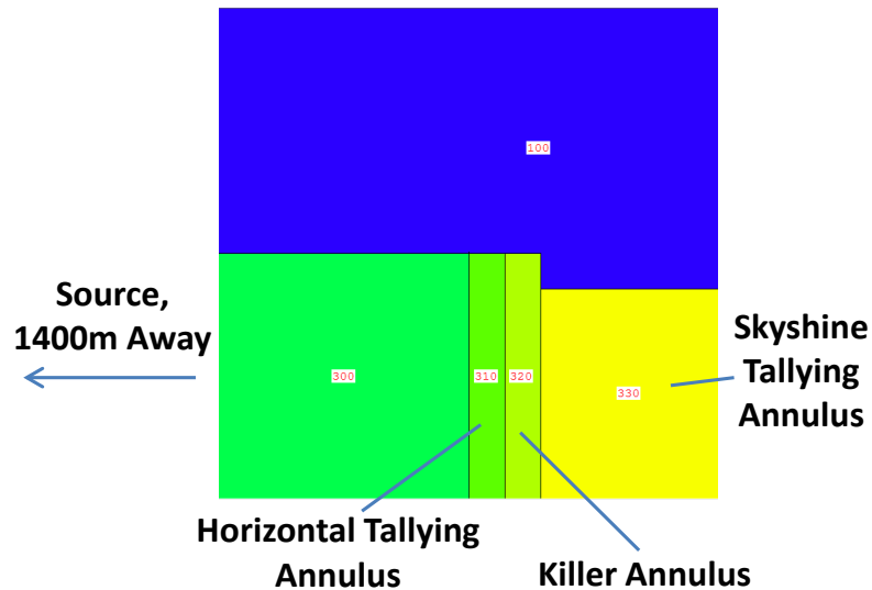
Figure 32. Cross section of tallying annuli and a killer annulus for Step 1 simulations. All cells in this image consist of air. Cell 320 is a killer annulus that eliminates all incident photons from the simulation.
