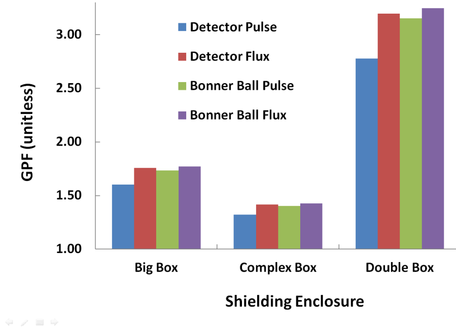
Figure 27. GPFs based on pulse and flux calculations for simulations of a LaBr 3 scintillator and a Bonner ball. Due to the large number of summed bins, the uncertainties for these results are \pm 0.001 , too small to resolve error bars.
