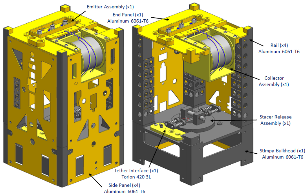
Fig. 10—Tether assembly
