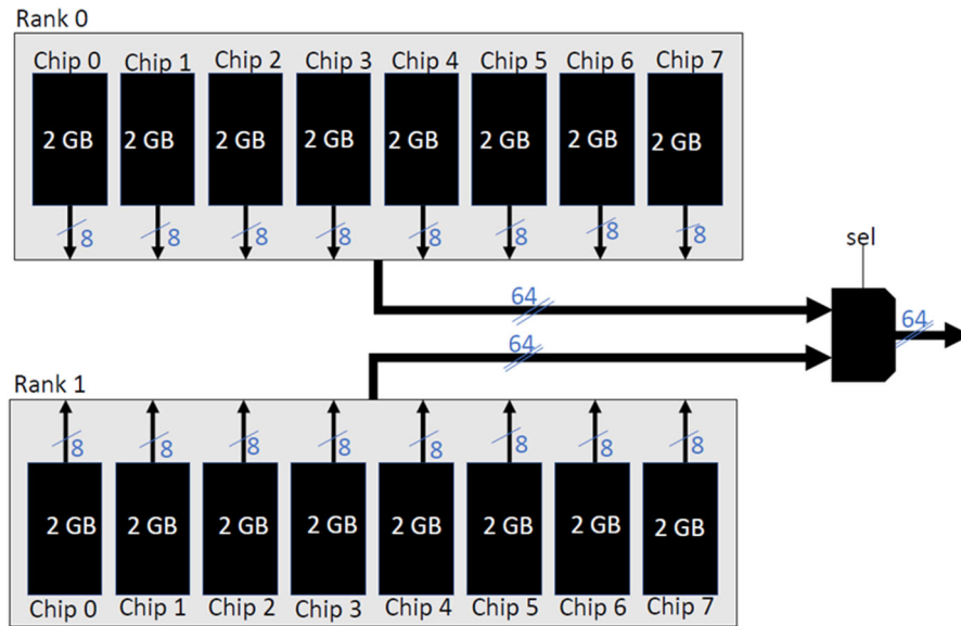
Figure 7. Internal structure of selected DDR4 SO-DIMMs
