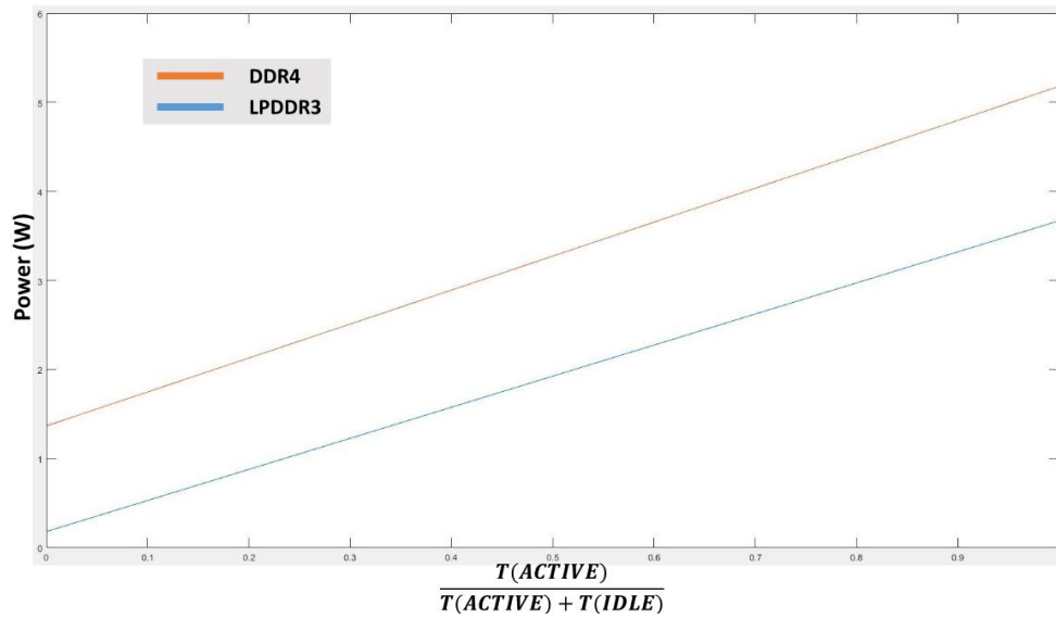
Figure 6. Power Consumption - LPDDR3
