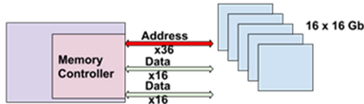
Figure 3. Memory design using 32 x 2 GB DRAM chips
