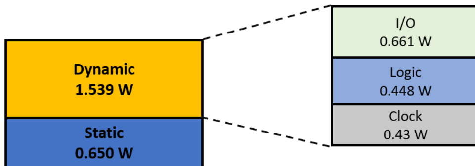
Figure 13. Power consumption
