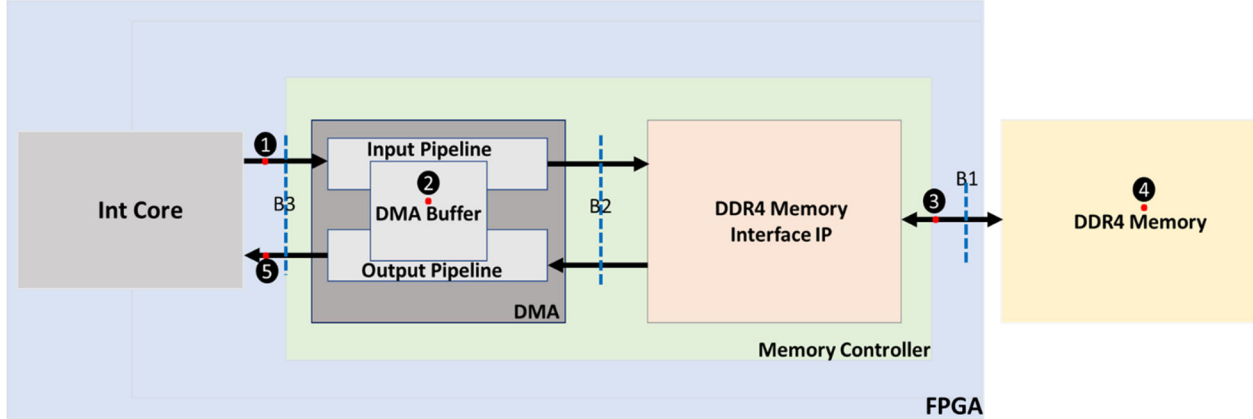
Figure 8. Conceptual design of the FPGA memory controller
