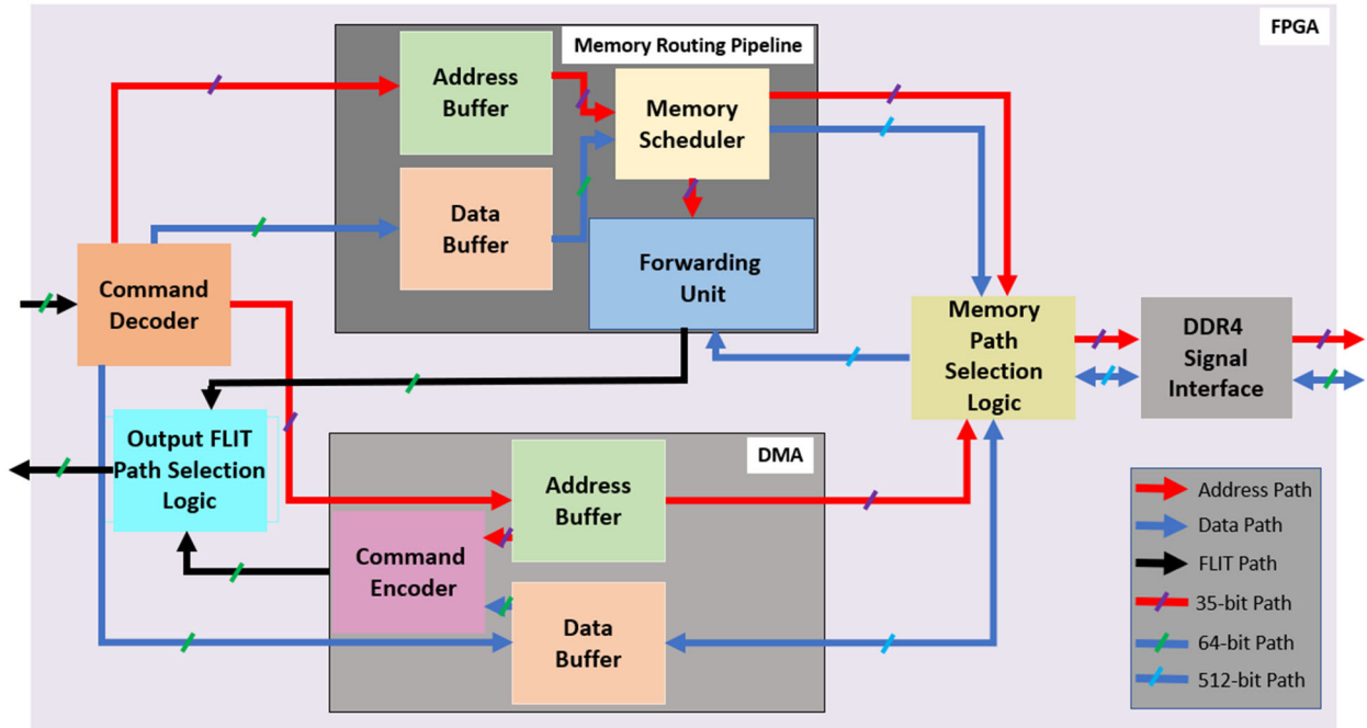
Figure 9. Overview of the memory controller
