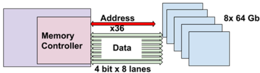
Figure 5. Memory design using 16 x 4 GB DRAM chips
