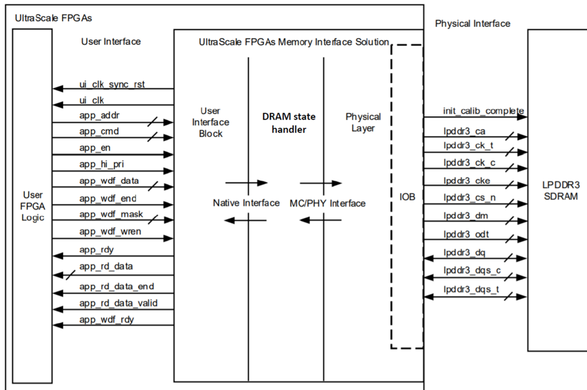
Figure 12. Xilinx UltraScale Architecture-Based FPGA Memory Signal Interface Core
