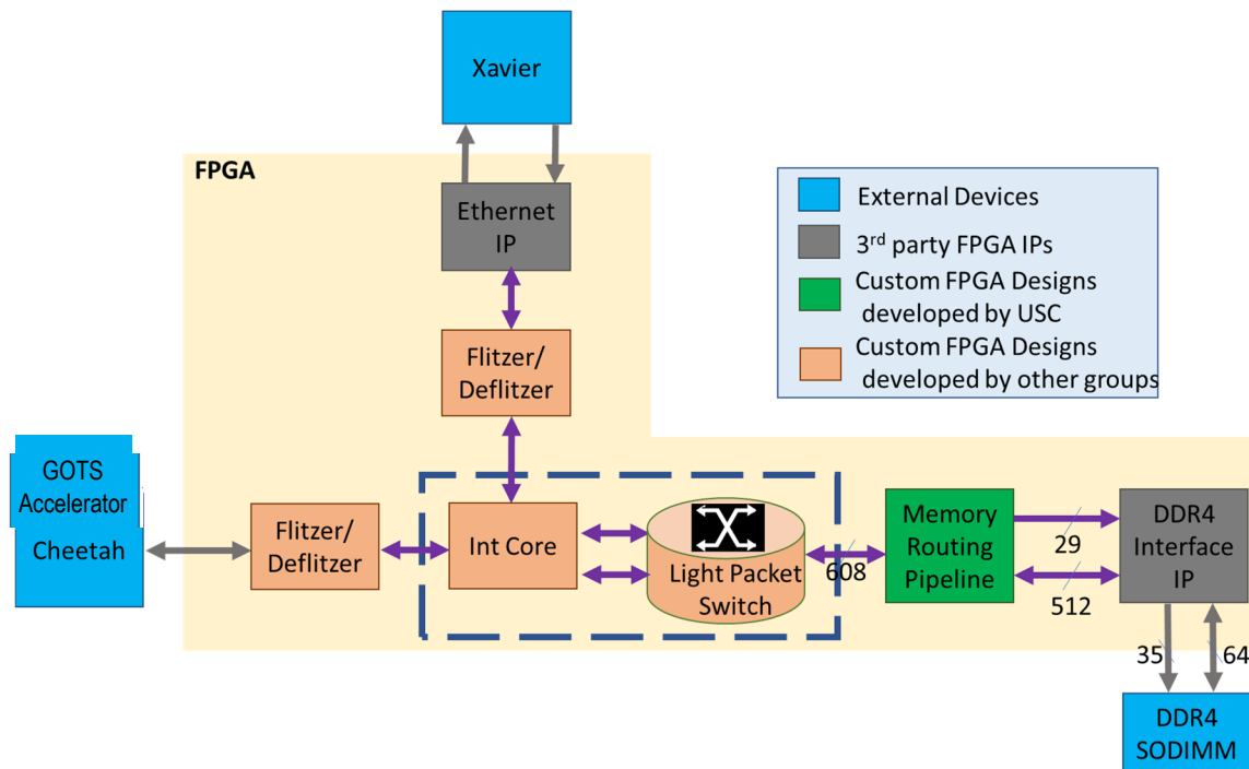
Figure 2. Top level model of FPGA design
