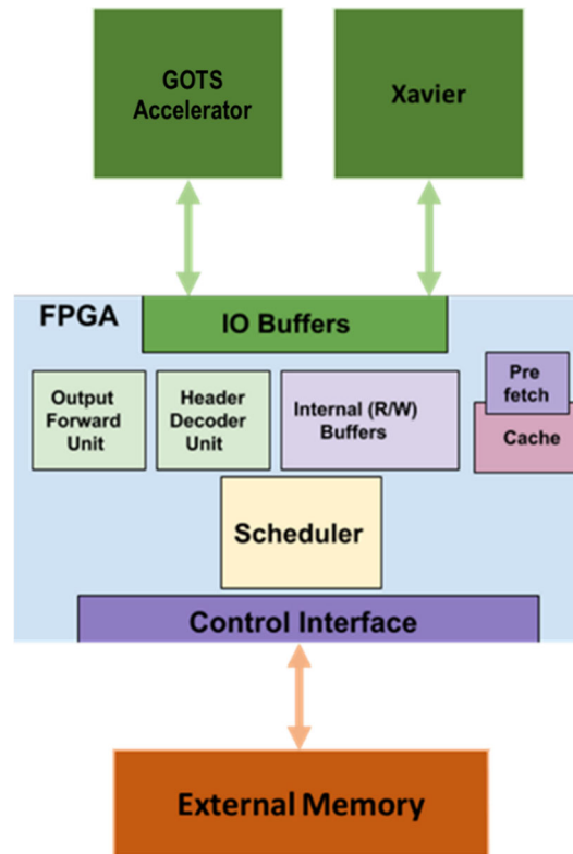
Figure 1. Conceptual design
