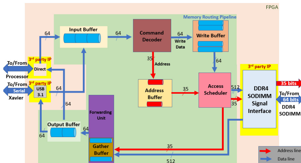
Figure 11. Memory Routing Pipeline
