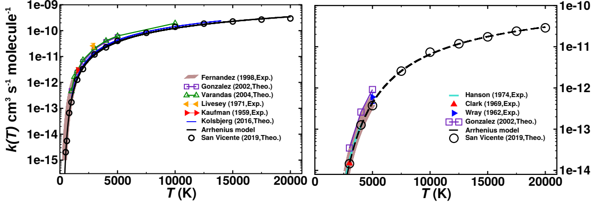
Figure 1: Total rates for the \text{N}(^4\text{S}) + \text{O}_2(^3\Sigma_g^-) \leftrightarrow \text{O}(^3\text{P}) + \text{NO}(^2\Pi) reactions. The left panel shows the rates for the forward reaction and the right panel show the rates for the reverse reaction. Arrhenius model are fits of the rates from Ref. 105 to a modified Arrhenius model. Data taken from Ref. 105
