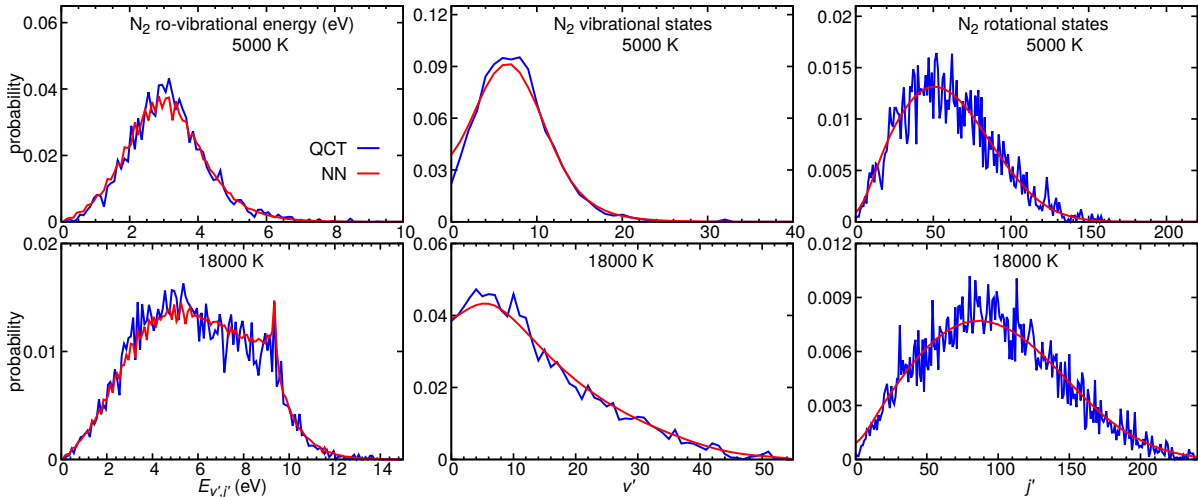
Figure 5: Distributions of product ro-vibrational states and ro-vibrational energies at 5000 and 18000 K for the \text{N} + \text{NO} \rightarrow \text{O} + \text{N}_2 reaction calculated from QCT on the ^3A' PES (blue) and predicted by the NN state-to-state model (red), respectively. Data taken from Ref. 165
