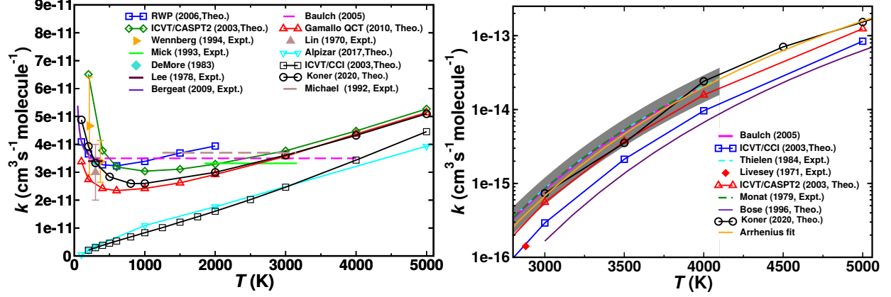
Figure 3: Rate coefficients for the \text{NO}(\text{X}^2\Pi) + \text{N}(^4\text{S}) \leftrightarrow \text{N}_2(\text{X}^1\Sigma_g^+) + \text{O}(^3\text{P}) as a function of temperature. Left panel shows rates for the forward reaction while the right panel shows the rates for the backward reaction. The results calculated in the present work are shown as lines with open circles. Experimental (assigned as ‘Expt.’) and Theoretical rates (assigned as ‘Theo.’) available in the literature are shown. 94,108,121,123–128,130–134 Data taken from Ref. 137
