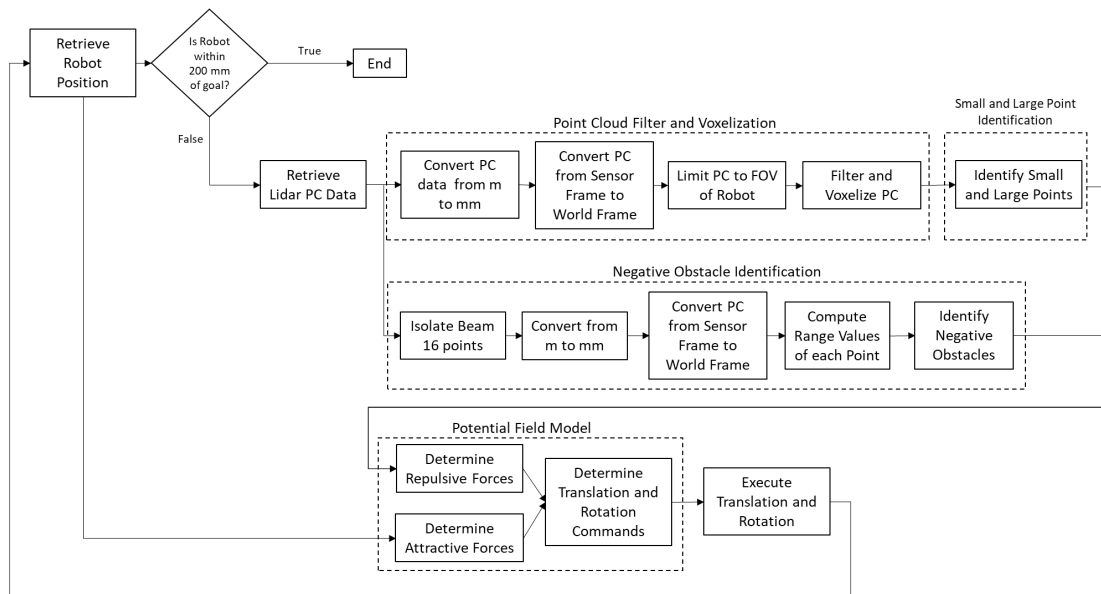
Figure 41. Block Diagram of the Control Algorithm
