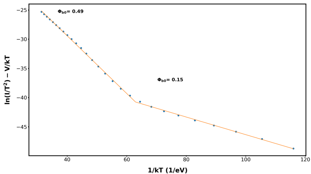
Figure 107. Device 19 post-stress Richardson plot
