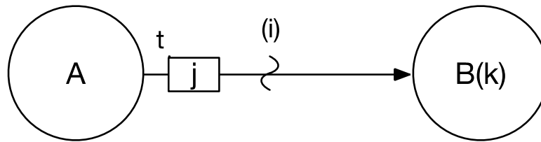
Figure 6. Simple Event Graph. Source: Buss (2017).
