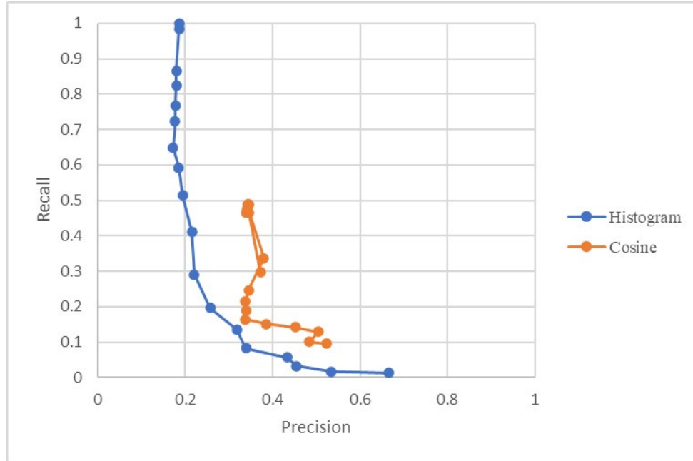
Figure 25. Histogram and Cosine Recall vs. Precision
