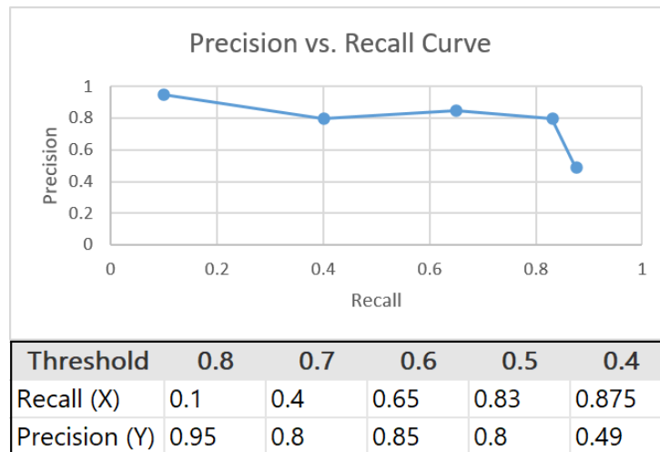
Figure 14. Example of Precision vs. Recall Curve
