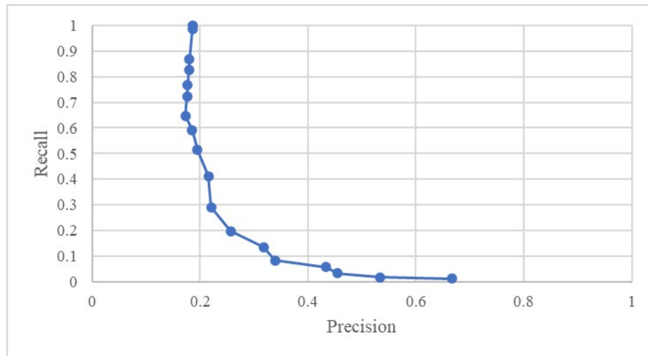
Figure 21. Histogram Recall vs. Precision
