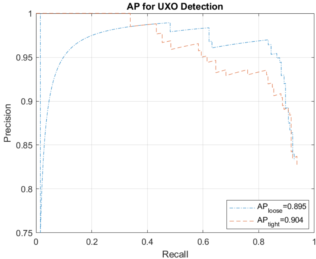
Figure 16. Combined Precision-Recall Graphs
